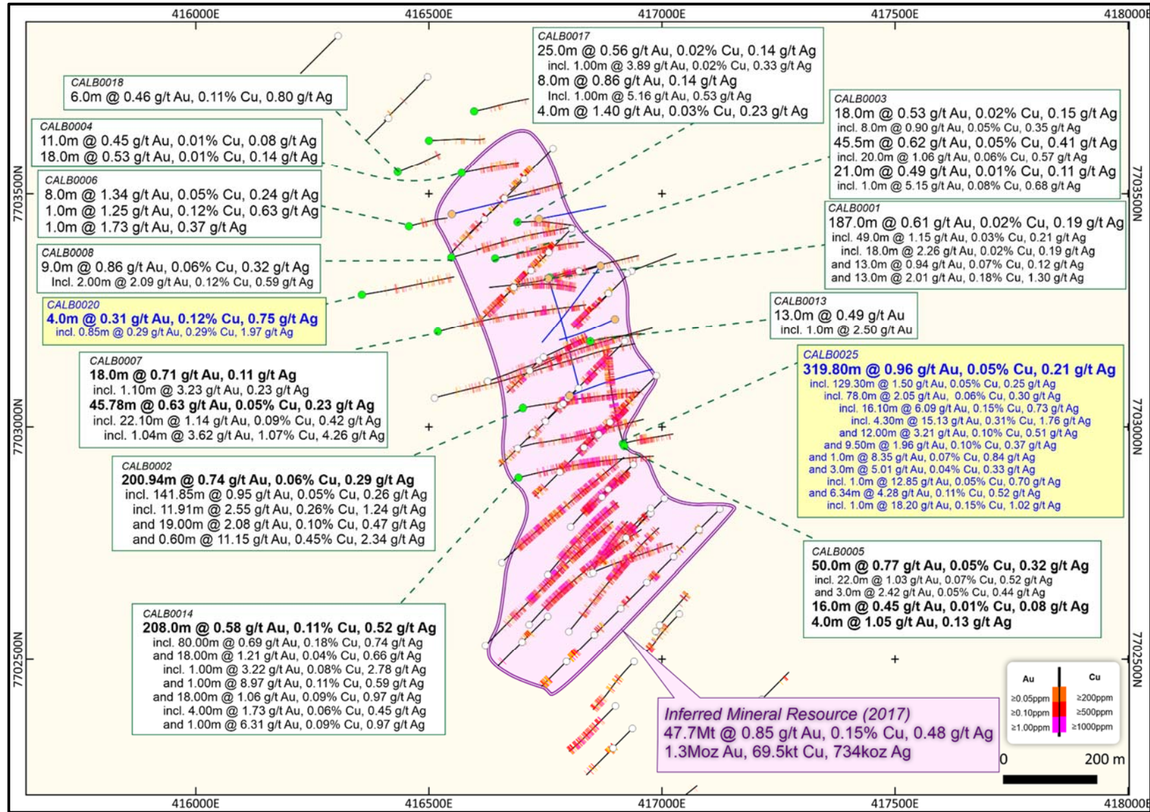
Figure 3: Calibre Deposit plan showing all Calibre drill (including 2020) holes depicting gold and copper grade distribution, with intersection labels for a selection of 2020 holes. NB: 500m MGA Zone 51 / GDA 2020 grid.
