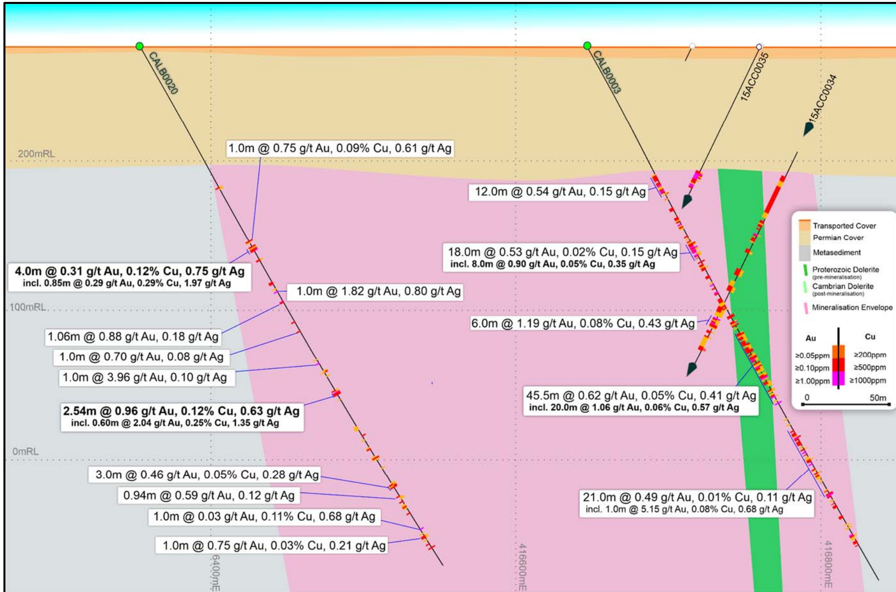
Figure 5: Calibre Deposit interpreted cross-section showing drill hole Au-Cu-Ag intersections including CALB0020 which is located outside to the west of the 2017 Mineral Resource. NB: 200m horizontal x 100m vertical MGA Zone 51 / GDA 2020 grid – Approx. north looking.
