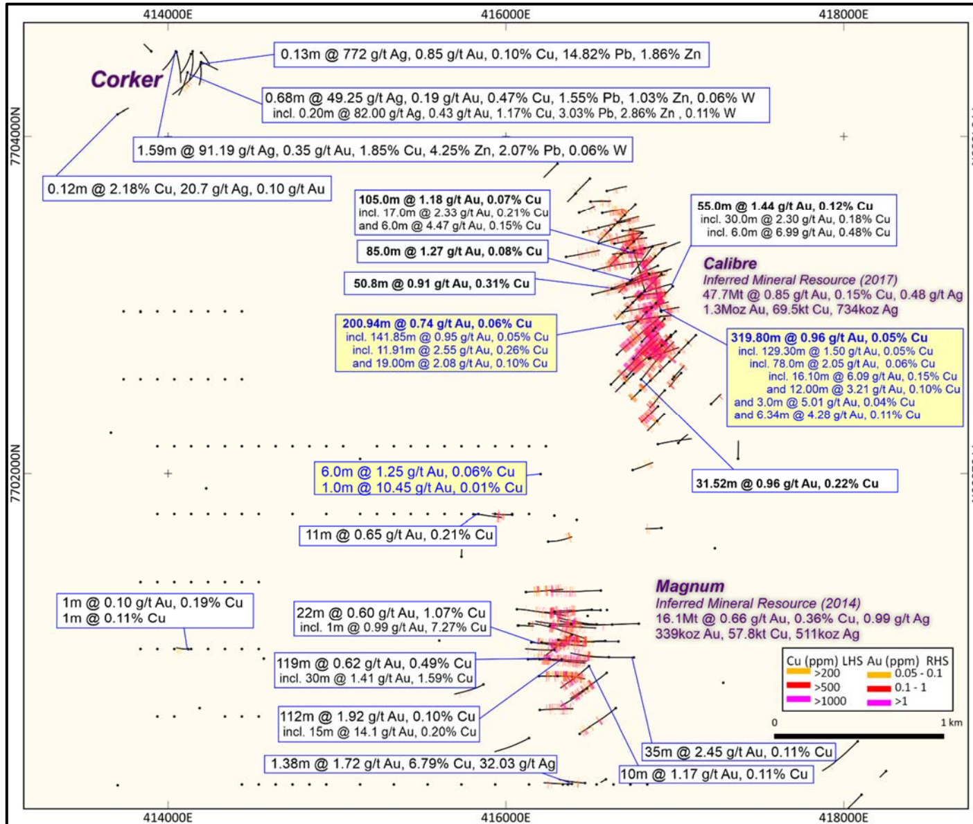
Figure 6: Magnum Dome plan showing Calibre, Magnum and Corker deposits, all drill (including 2020) holes depicting gold and copper grade distribution, with intersection labels for a selection of holes. NB: 2 km MGA Zone 51 / GDA 2020 grid.
