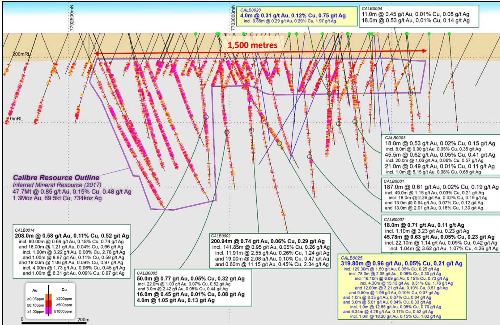
Figure 2: Calibre Deposit west looking vertical projection showing all Calibre drill (including 2020) holes depicting gold and copper grade distribution, with intersection labels for a selection of 2020 holes. Note significant gold-copper drill intersections substantially outside the limit of the 2017 Mineral Resource boundary. NB: 500m horizontal x 200m vertical MGA Zone 51 / GDA 2020 grid.
