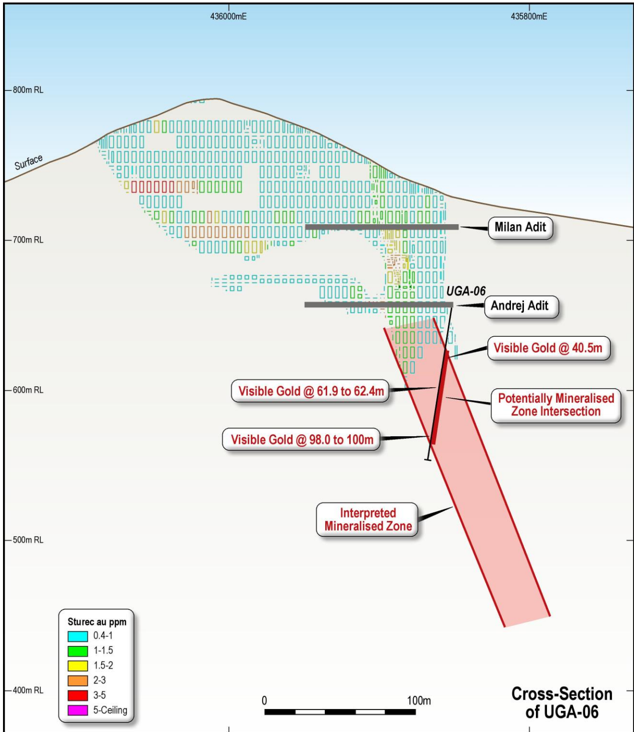
Figure 7: Cross-section showing the current interpretation of the extents of the potentially mineralisation zone below the current Sturec Mineral Resource, from approximately 36.5m to 104.5m down hole intersected in UGA-06
