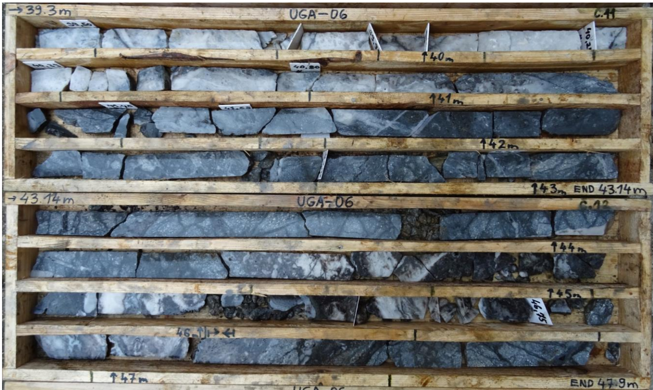
Figure 9: UGA-06 drill core; interval from 39.3m to 47.9m (down-hole) showing quartz filled vein/stockwork/breccia structures, variably rich in fine to very fine grained sulphides (mainly pyrite/marcasite) and hosted within strongly argillic altered andesite host rock. Traces of visible gold identified at 40.5m
