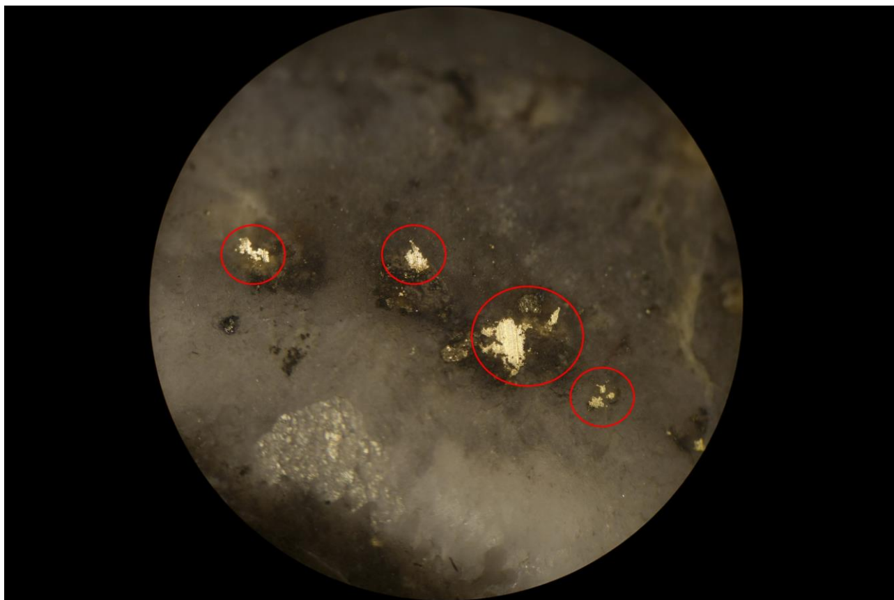
Figure 6: Stereoscope image of the visible gold at 98.85m associated with pyrite (x40 magnification: field of view is ~5mm) in UGA-06
