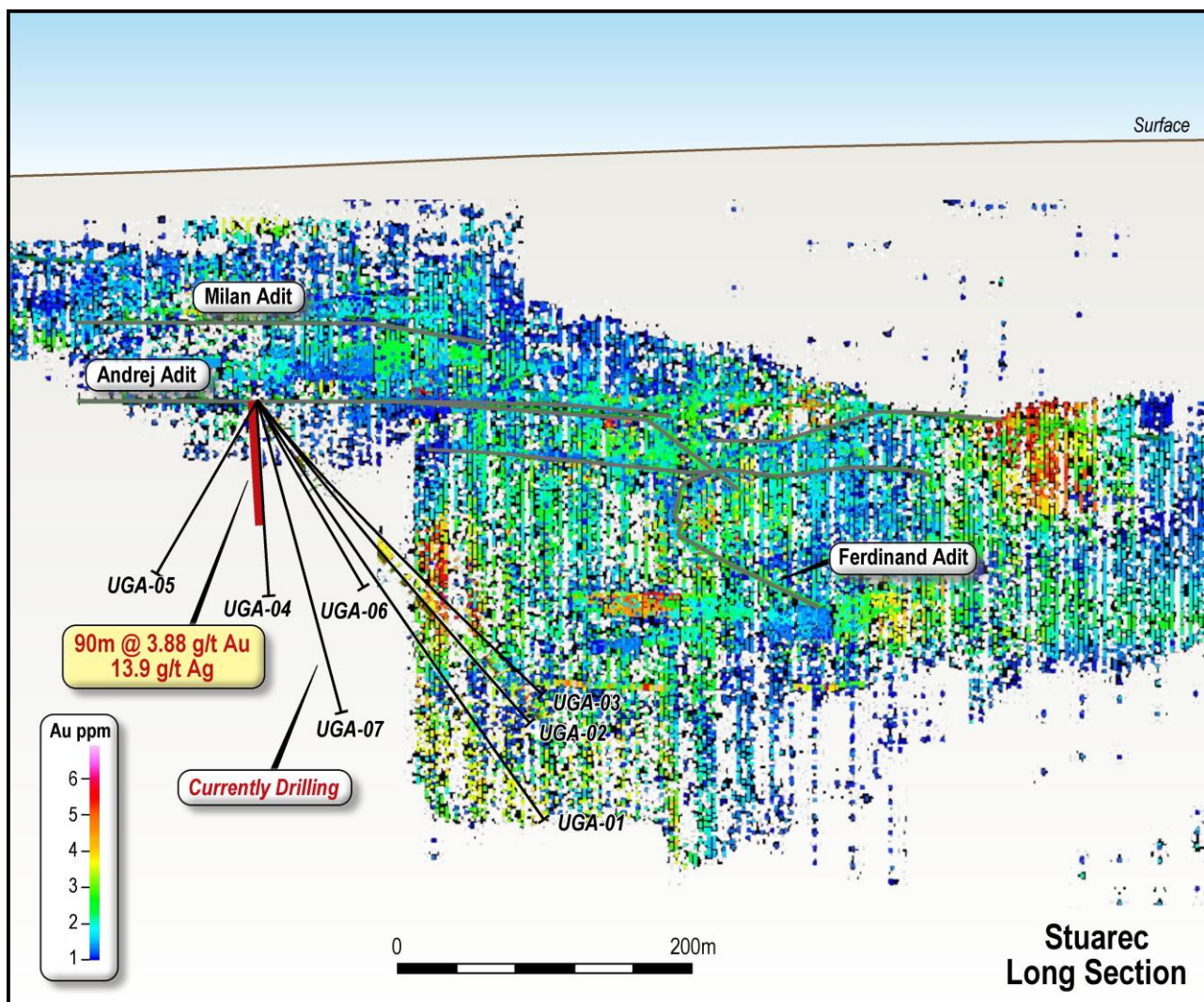
Figure 8: Long-section showing the traces of drill holes from the current drill program; shown relative to mineralisation within the existing Sturec Mineral Resource displayed as a 3D point cloud (grade scale shown with pseudocolor spectrum). This view is looking west.
