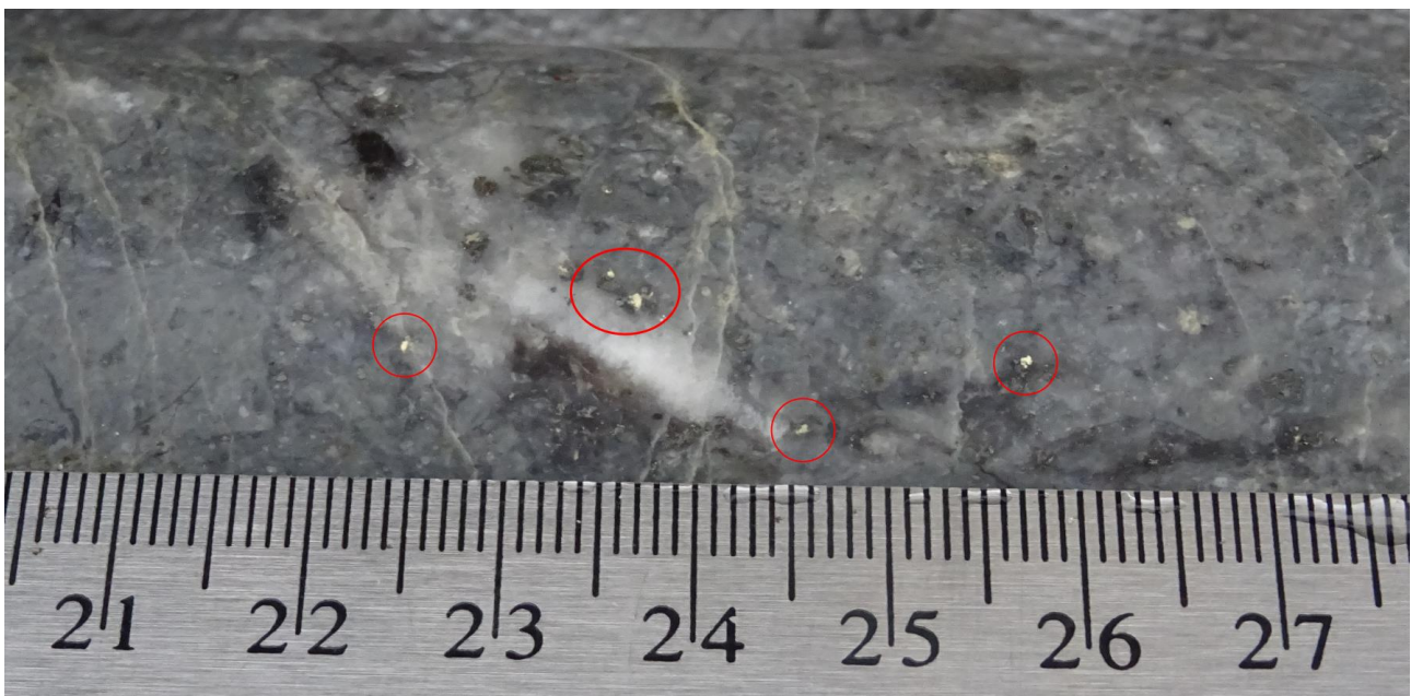
Figure 1: Visible gold associated with pyrite in drusy, fine grained, white, grey to dark grey chalcedonic quartz at 98.81-98.85m in UGA-06 (close up of visible gold shown in Figure 6)
