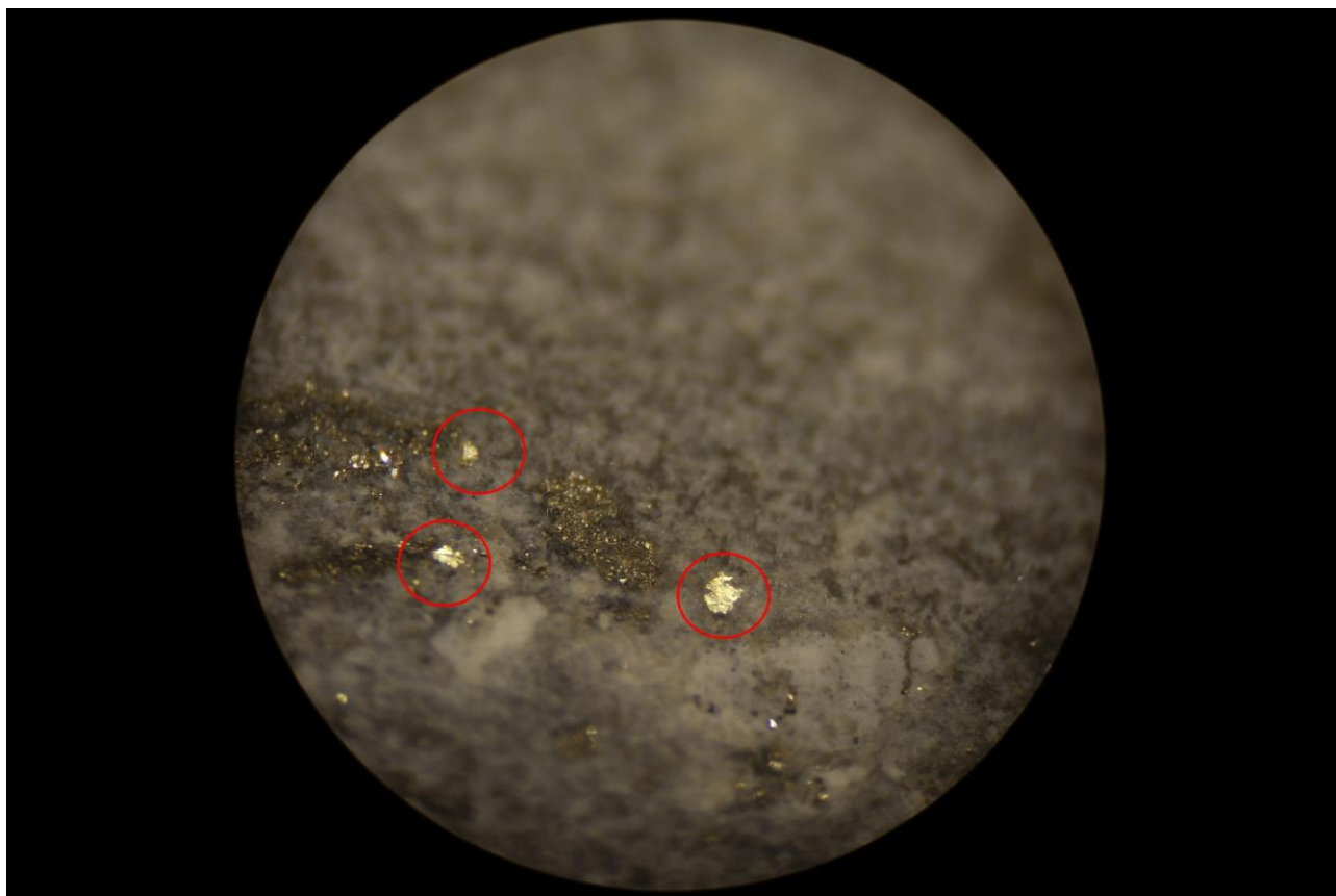
Figure 3: Stereoscope image of the visible gold at 61.9m associated with pyrite (x40 magnification: field of view is ~5mm) in UGA-06
