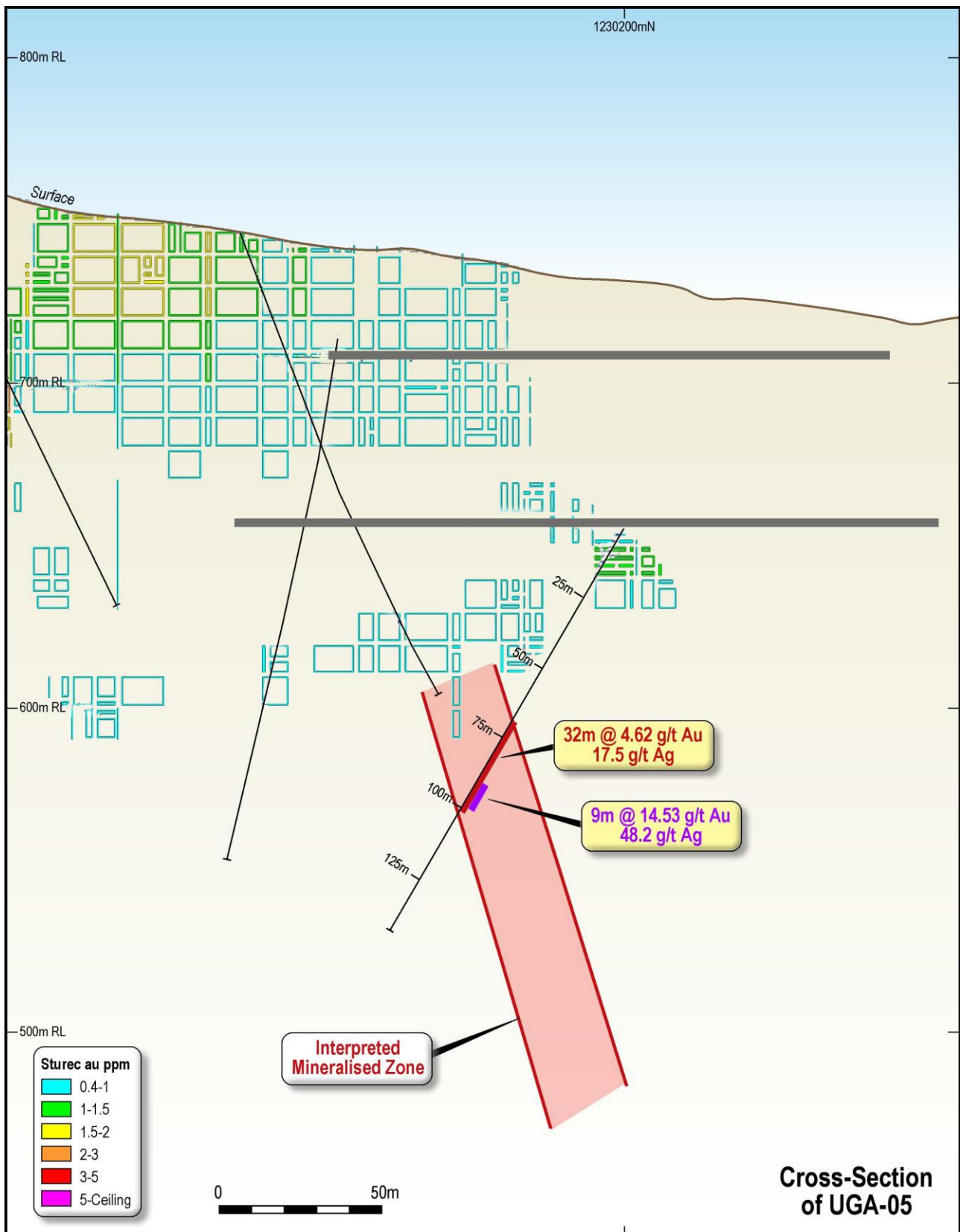
Figure 3: Cross-section showing UGA-05 and the interpretation of the extents of the mineralisation zone below the current Sturec Mineral Resource.
