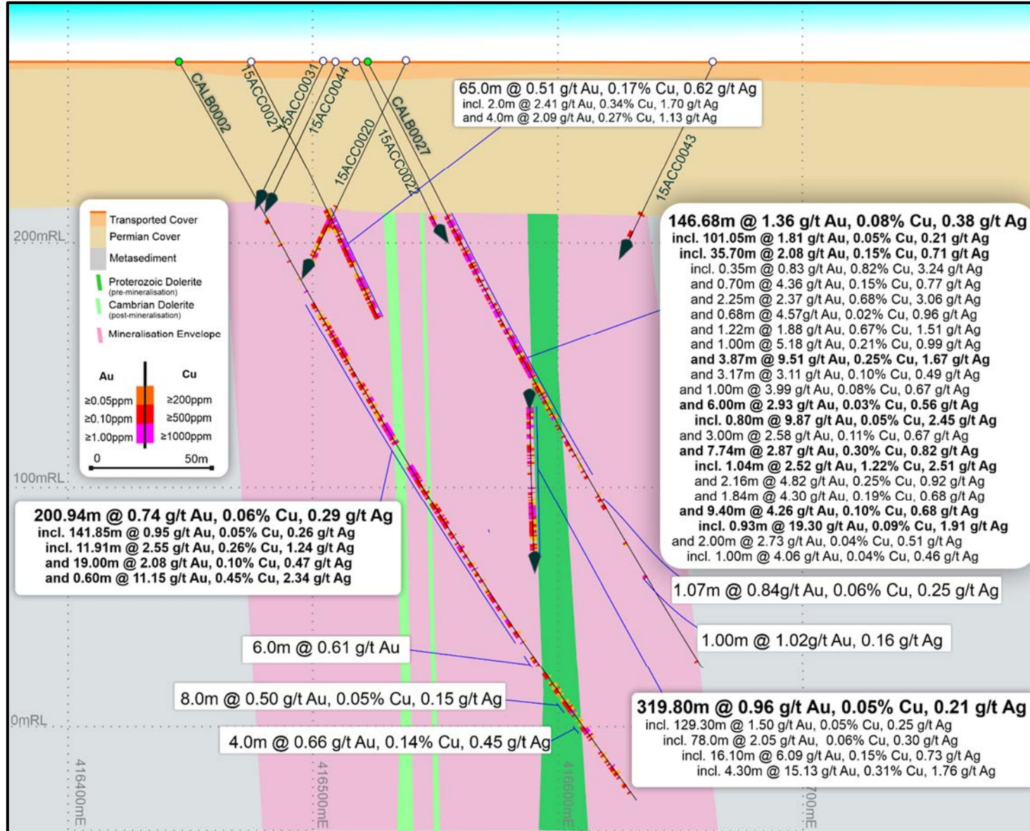
Figure 4: Calibre Deposit interpreted east-west cross-section showing drill hole Au-Cu-Ag intersections including CALB0027. NB: 100m horizontal x 100m vertical MGA Zone 51 / GDA 2020 grid – Approx. north looking.
