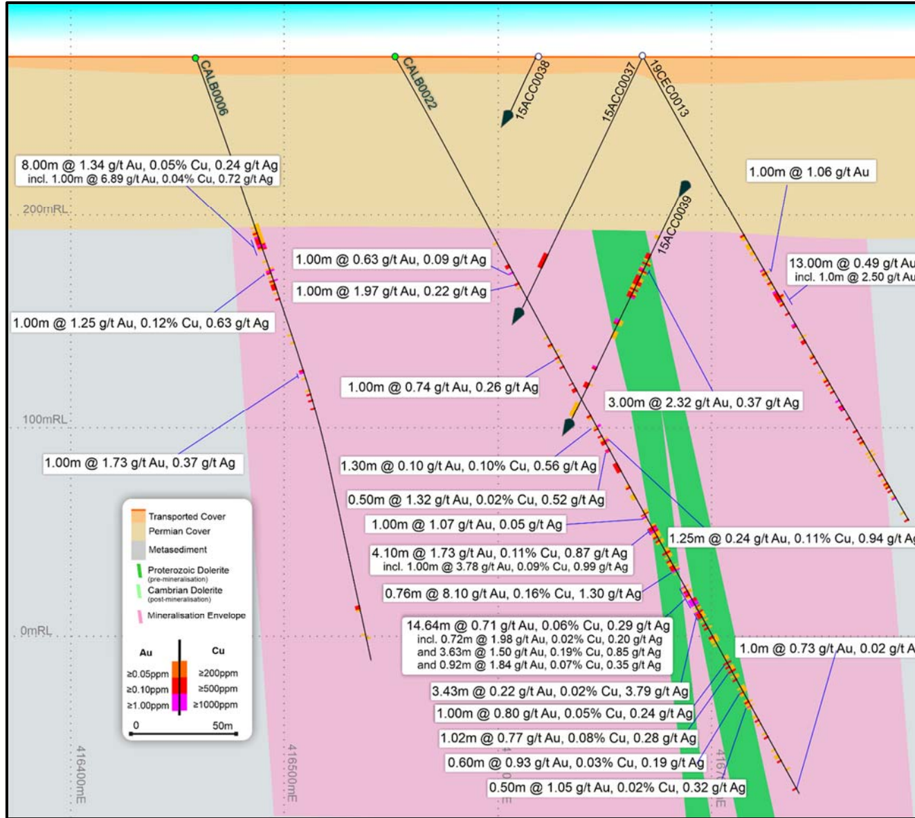
Figure 5: Calibre Deposit interpreted east-west cross-section showing drill hole Au-Cu-Ag intersections including CALB0022. NB: 200m horizontal x 100m vertical MGA Zone 51 / GDA 2020 grid – Approx. north looking.
