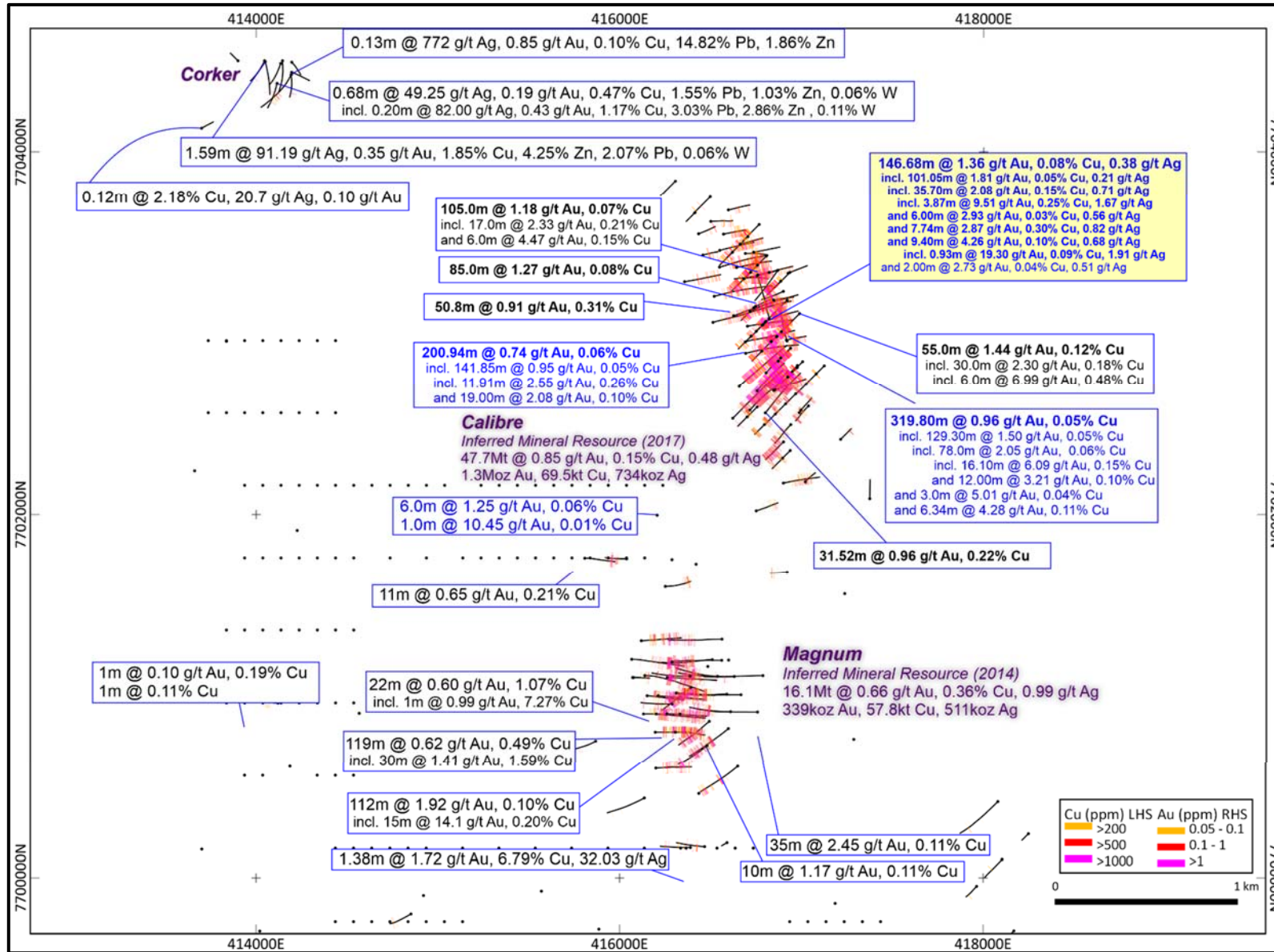
Figure 6: Magnum Dome plan showing Calibre, Magnum and Corker deposits, all drill (including 2020) holes depicting gold and copper grade distribution, with intersection labels for a selection of holes. NB: 2 km MGA Zone 51 / GDA 2020 grid.
