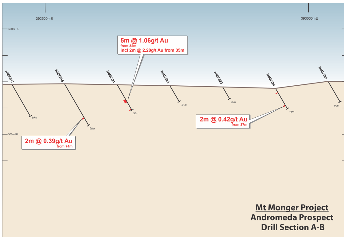
Figure 4. Andromeda Prospect drill cross-section line A-B showing gold intercepts.
