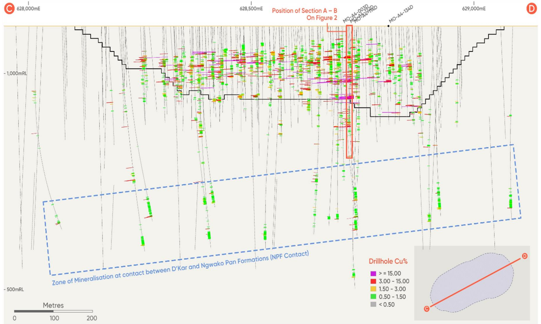
A4 Longitudinal projection looking north showing optimised pit shell for the A4 Maiden Resource and copper grades represented as histograms for holes where assays have been received. Deeper intersections within the blue rectangle are related to NPF contact mineralisation announced previously by MOD Resources Ltd.
