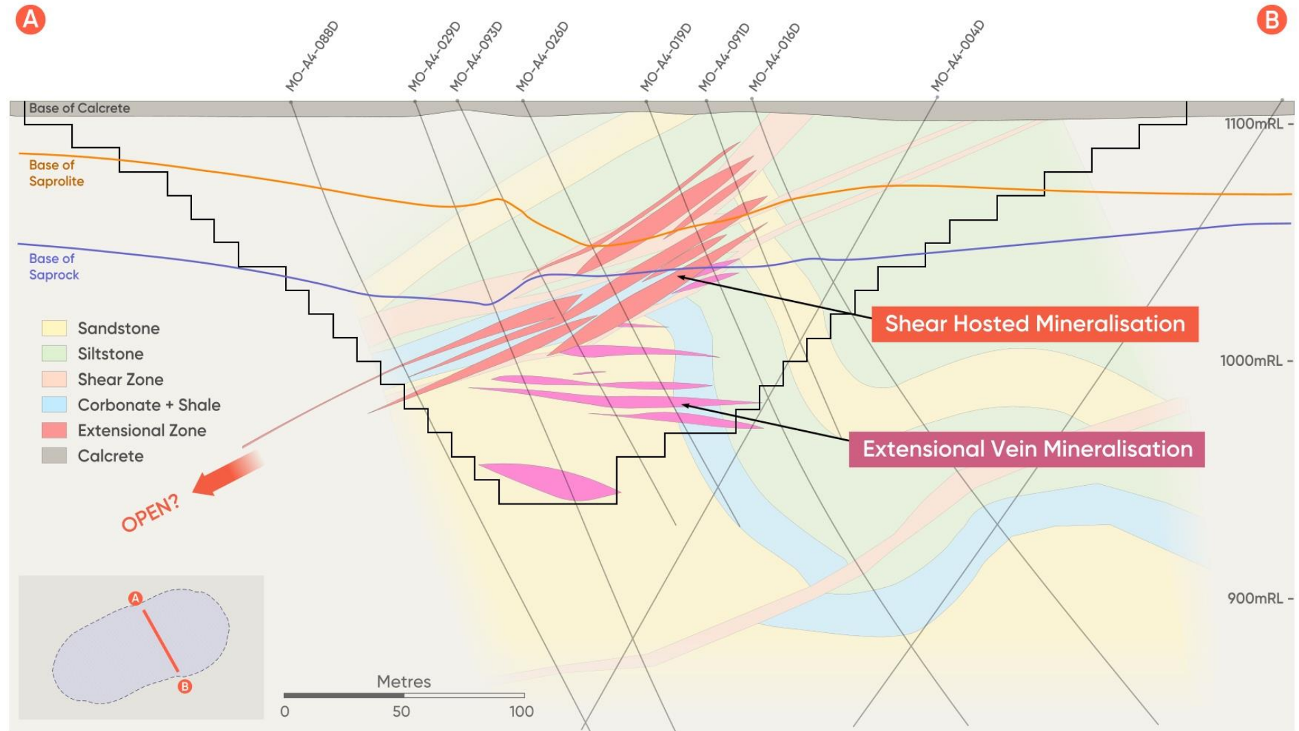
A4 schematic cross-section – showing interpreted geology and mineralisation styles across the A4 Deposit. US$4.50/lb Cu price optimised pit shell used to constrain the MRE shown in black outline.
