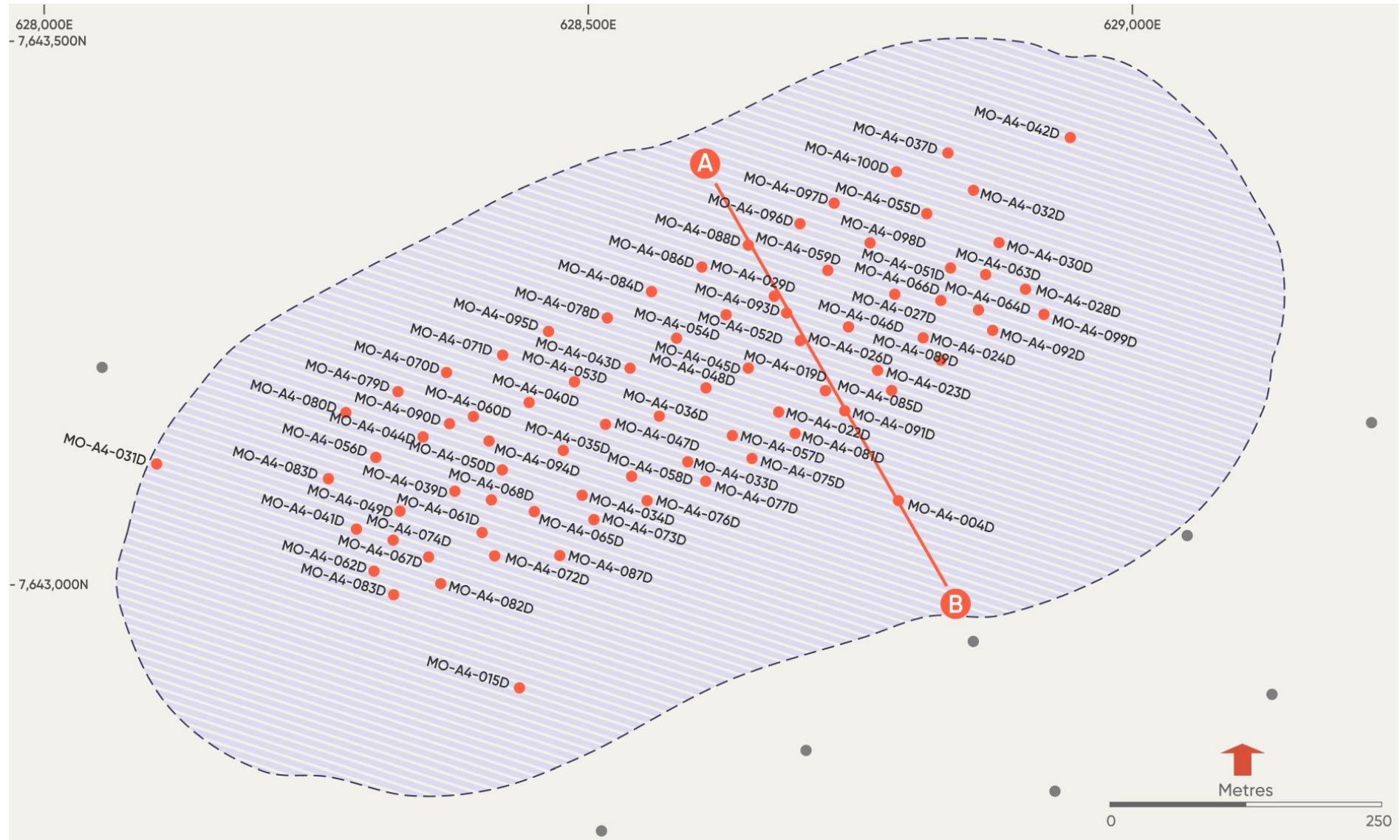
A4 Plan view – collar location of drill holes used to inform the Mineral Resource Estimate (MRE). US$4.50/lb Cu price optimised pit shell shown in dashed black outline. Grey collars represent existing holes targeting deeper mineralisation not included in the MRE.
