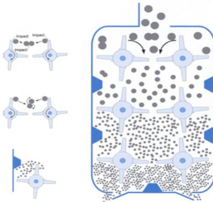
Figure 2: Six shaft model showing internal milling process mechanism.
