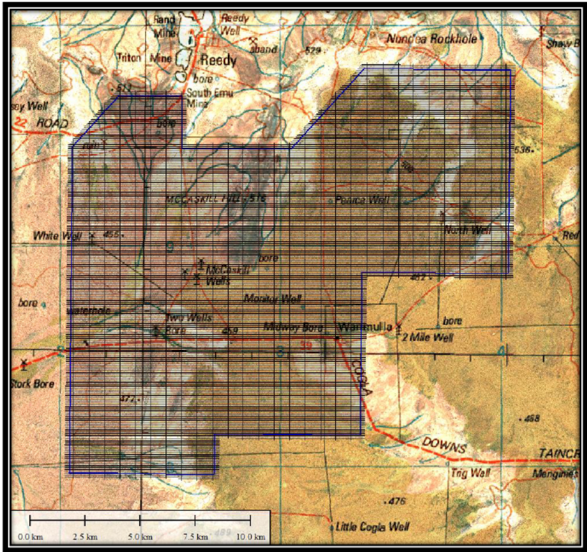
Figure 1: Aeromagnetic survey outline at Reedy South
