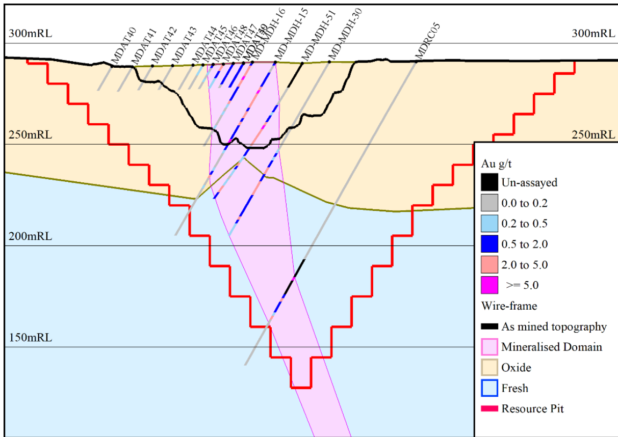
Figure 2 – May Day pit optimisation cross section
