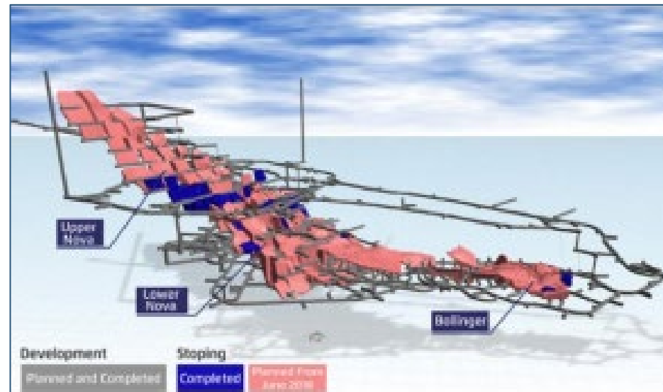
3D View of the Nova Nickel Mine
