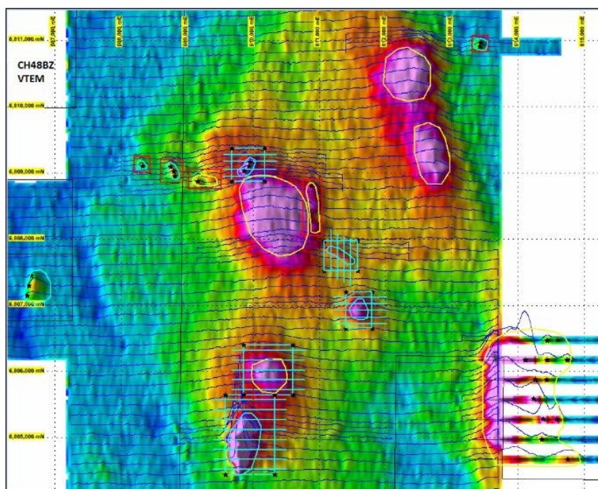
Narndee Project: Recent VTEM survey outlining priority targets
