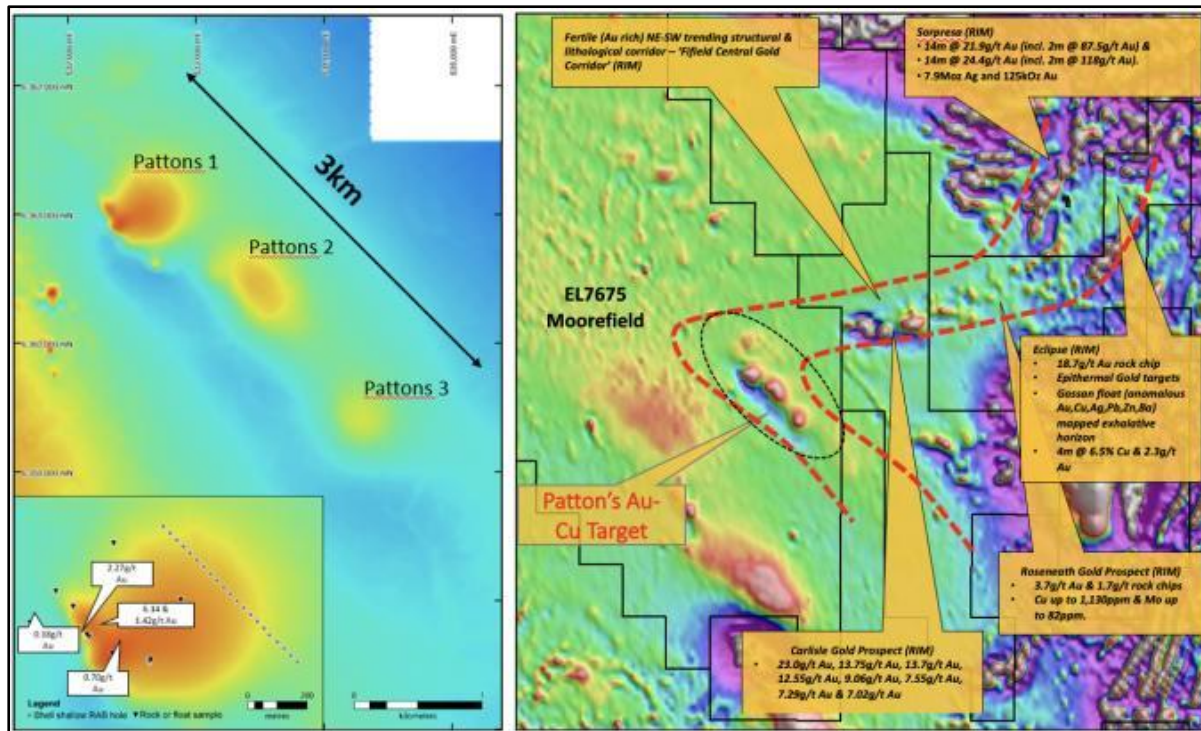
Pattons, Ghost Hill, Lima, Meloolla base metal prospects
