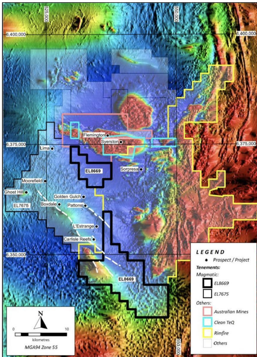
Moorefield project showing tenement holders over the RTP magnetic image highlighting the Boxdale-Carlisle and Pattons trends extending into EL8669 Exploration Potential
