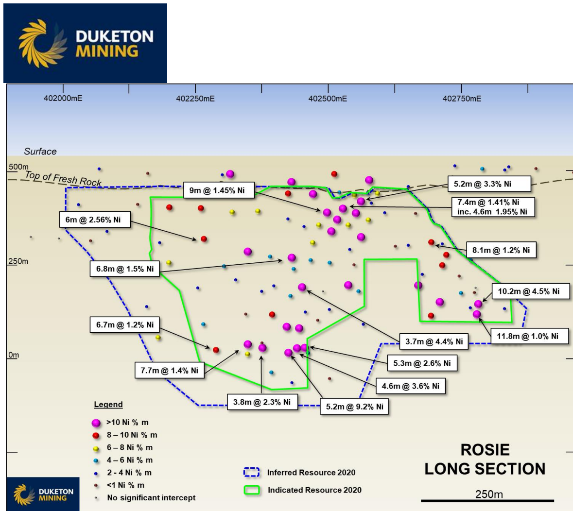
Figure 3. Long Section of Rosie, looking north east.
