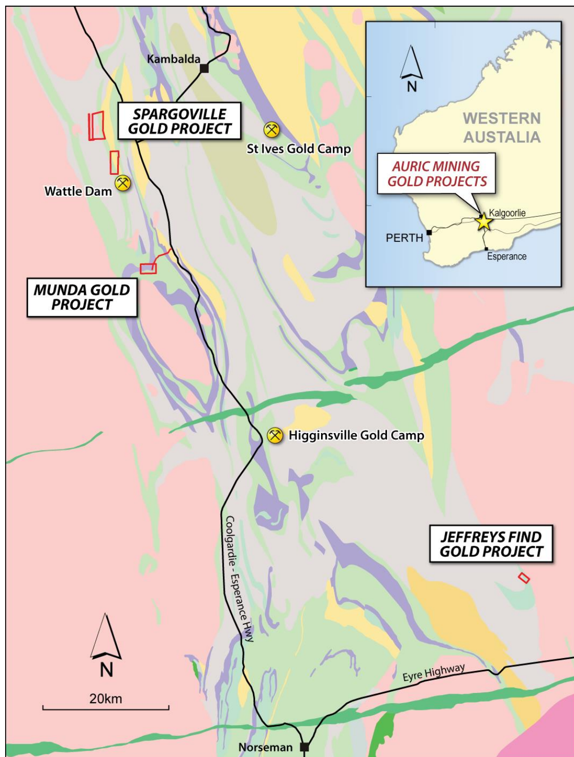
Geological map derived from Striewski, 2020. Figure produced November 2020. Tenements shown in red.
