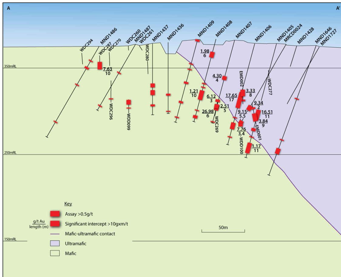
Figure 5: Munda representative cross section
