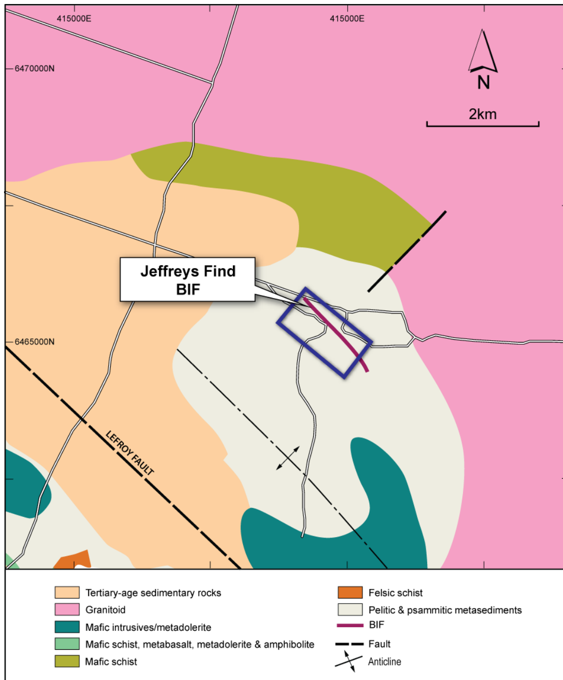
Figure 8: Jeffreys Find local geology and tenure
