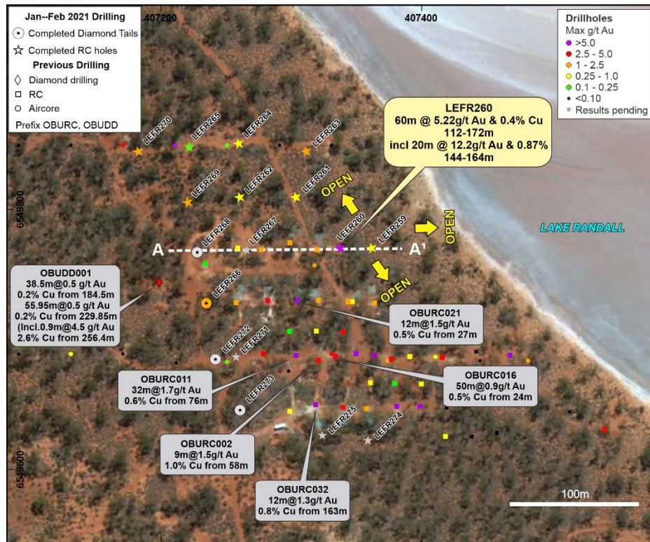
Figure 4 Inset plan highlighting drill hole plan at the Burns prospect and the location of LEFR260 relative to previous drill hole intercepts. Refer to Figure 5 for cross section AA'
