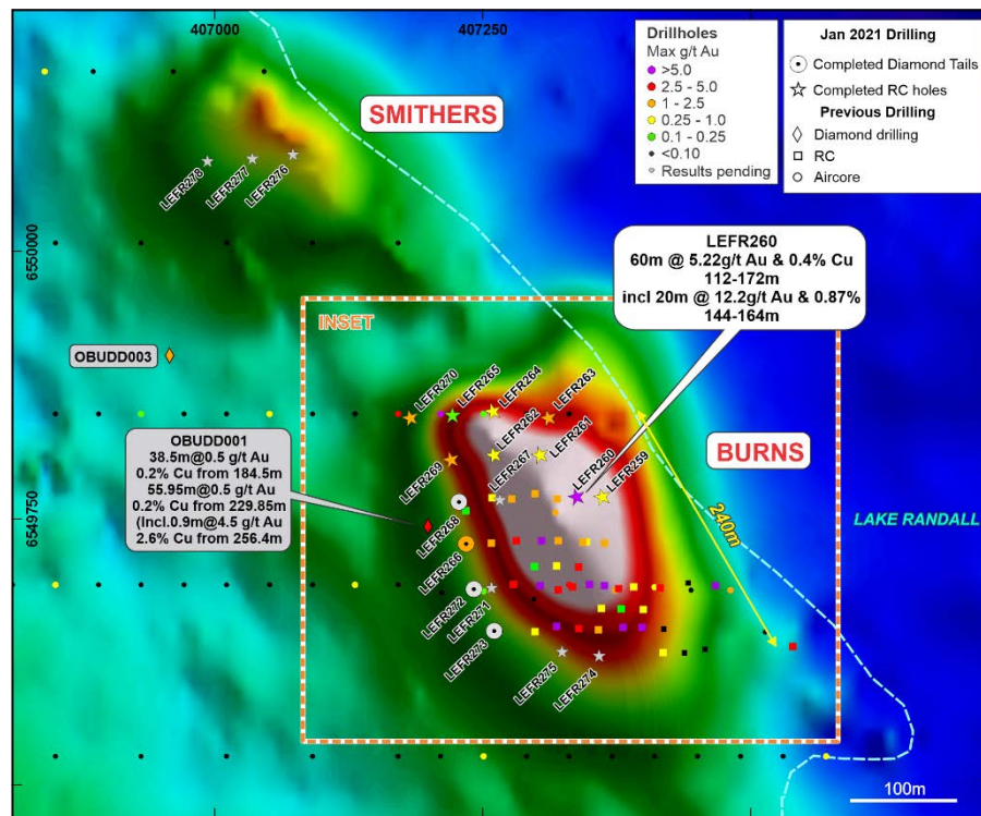
Figure 3 Inset plan highlighting drill hole plan at the Burns prospect over a magnetic image (TMI RTP) prepared from merged ground and aeromagnetic data. The warm colours highlight a strong magnetic response from the bedrock (refer to Figure 4 for detailed drill hole plan).
