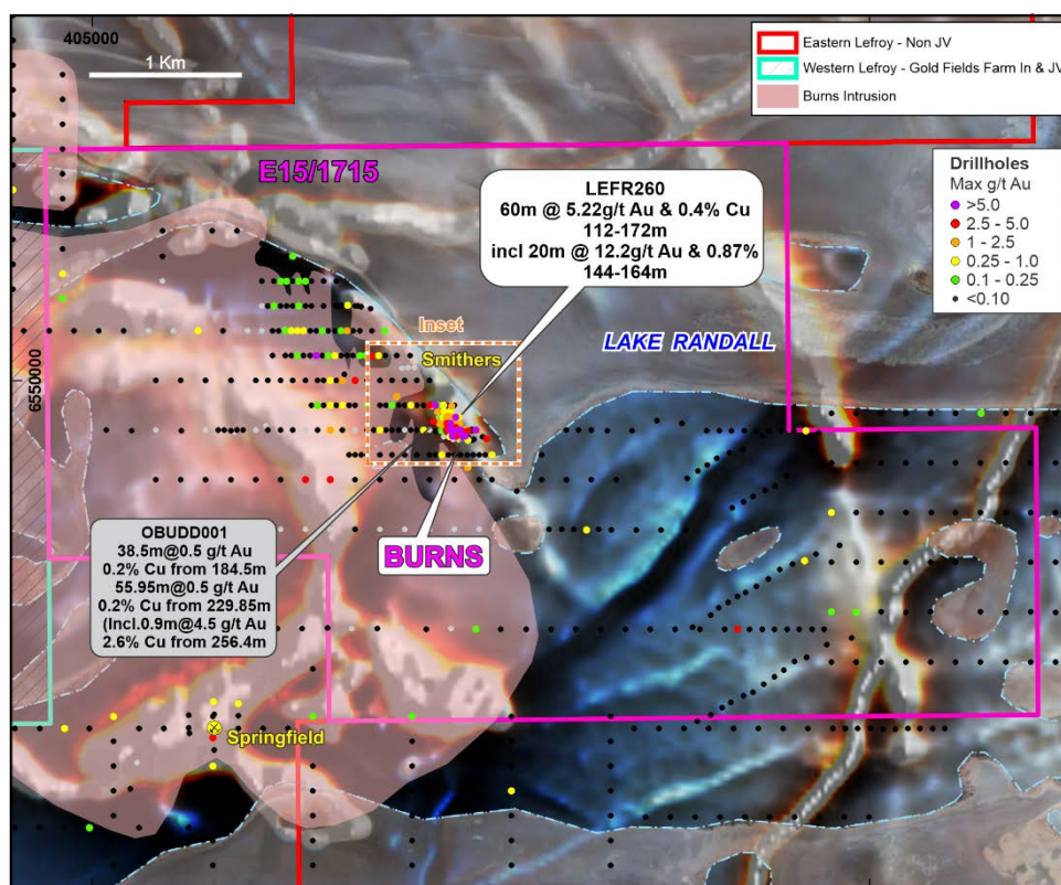
Figure 2 Inset plan highlighting tenement E15/1715, the Burns prospect, extent of the Burns Intrusion and the strike extension of the Lucky Strike BIF with compiled previous drill holes. Refer to Figures 3 and 4 for the Burns drill hole plan.
