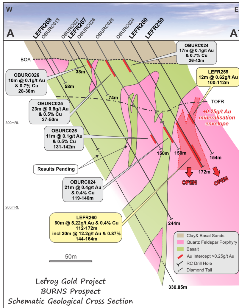
Figure 5 Schematic geological cross section highlighting LEFR260.
