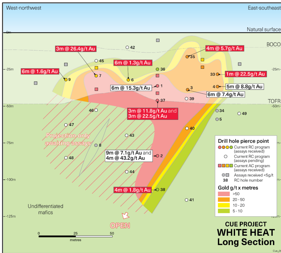
Figure 4: Long section along the plane of the mineralisation showing current drill holes at the White Heat Prospect
