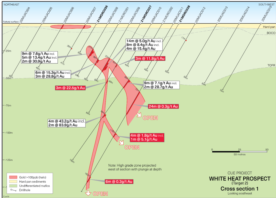
Figure 3: Cross-section showing current drill holes at the White Heat Prospect
