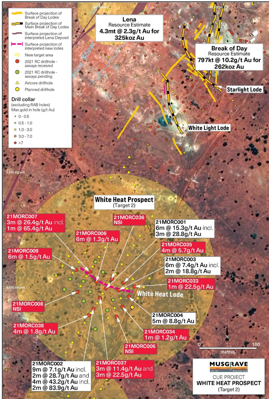
Figure 2: Plan showing drill hole collars at White Heat prospect and new assay results (assays are pending for RC drill holes that are not labelled)
