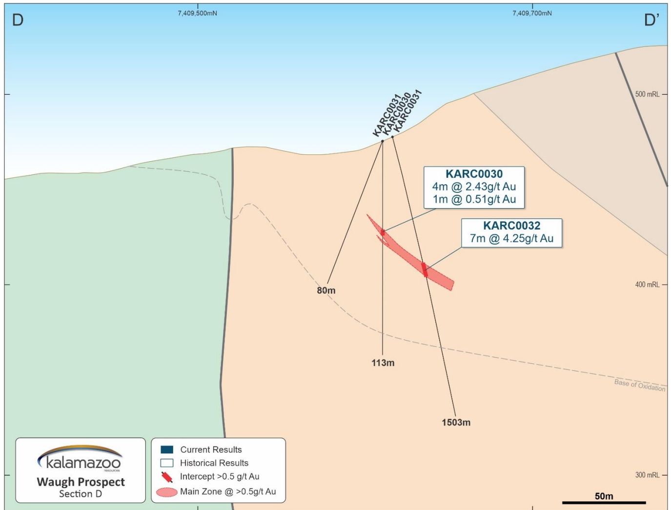
Figure 7: Cross-section interpretation of the geology and mineralised intercepts at section line D
