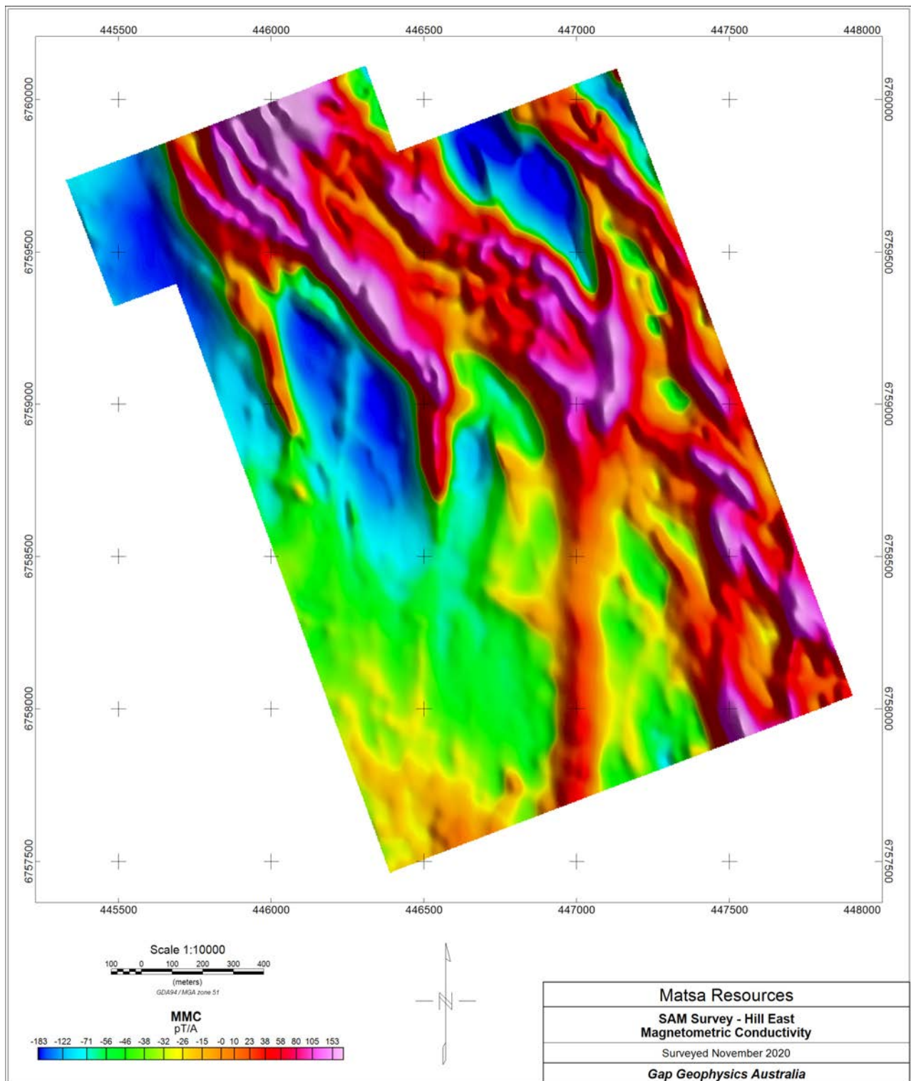
Figure 4 Hill East – magnetometric conductivity, stitched grids.
