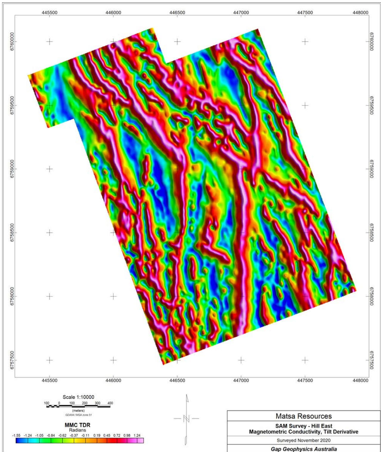
Figure 5 Hill East – magnetometric conductivity, tilt derivative, stitched grids.
