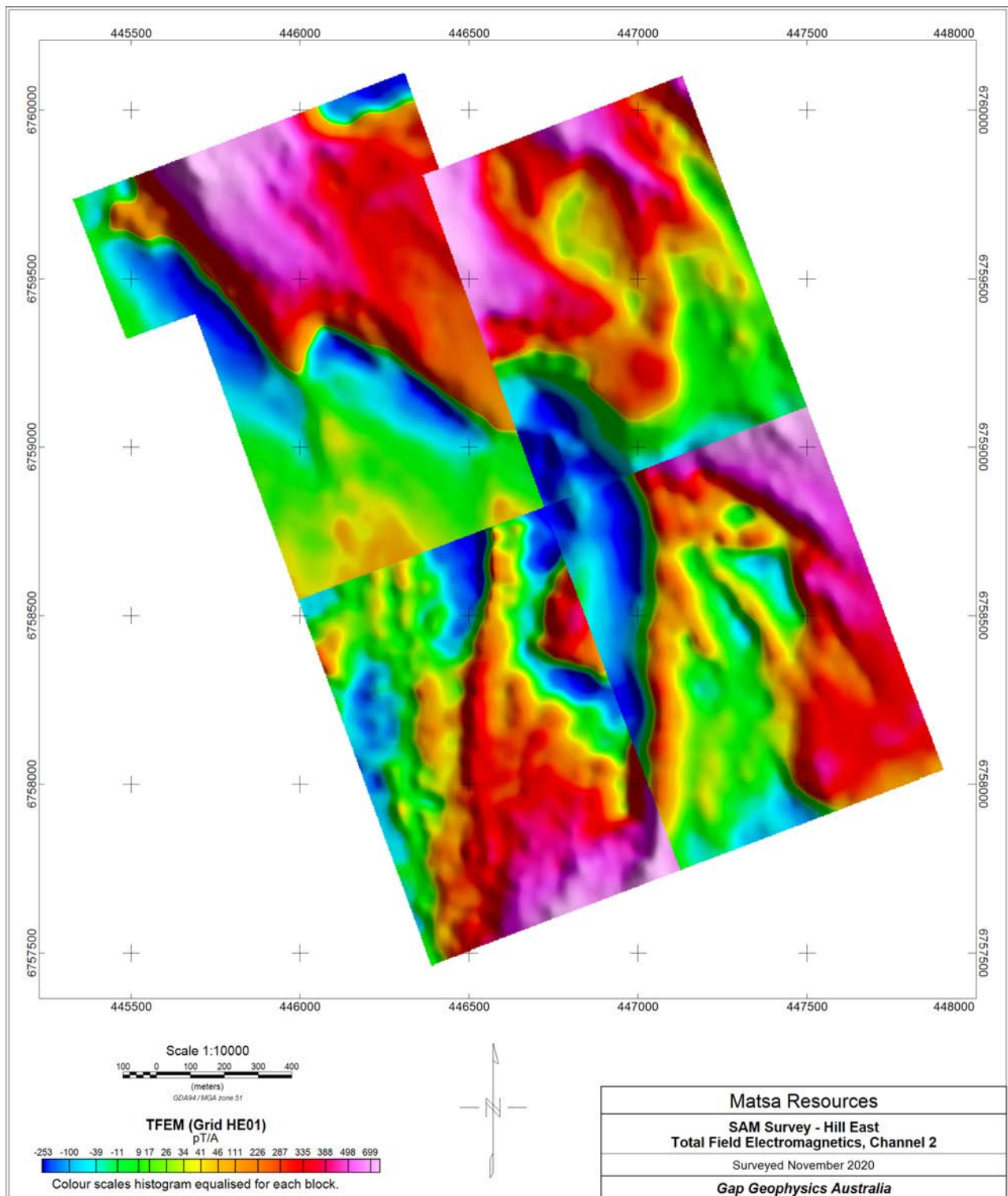
Figure 7 Hill East – total field electromagnetics, channel 2, mosaic.
