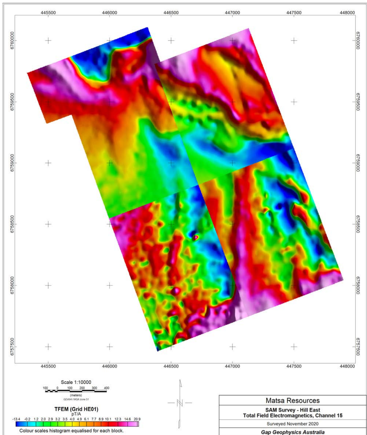
Figure 20 Hill East – total field electromagnetics, channel 15, mosaic.
