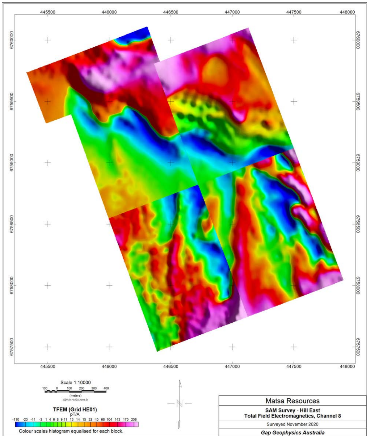
Figure 13 Hill East – total field electromagnetics, channel 8, mosaic.
