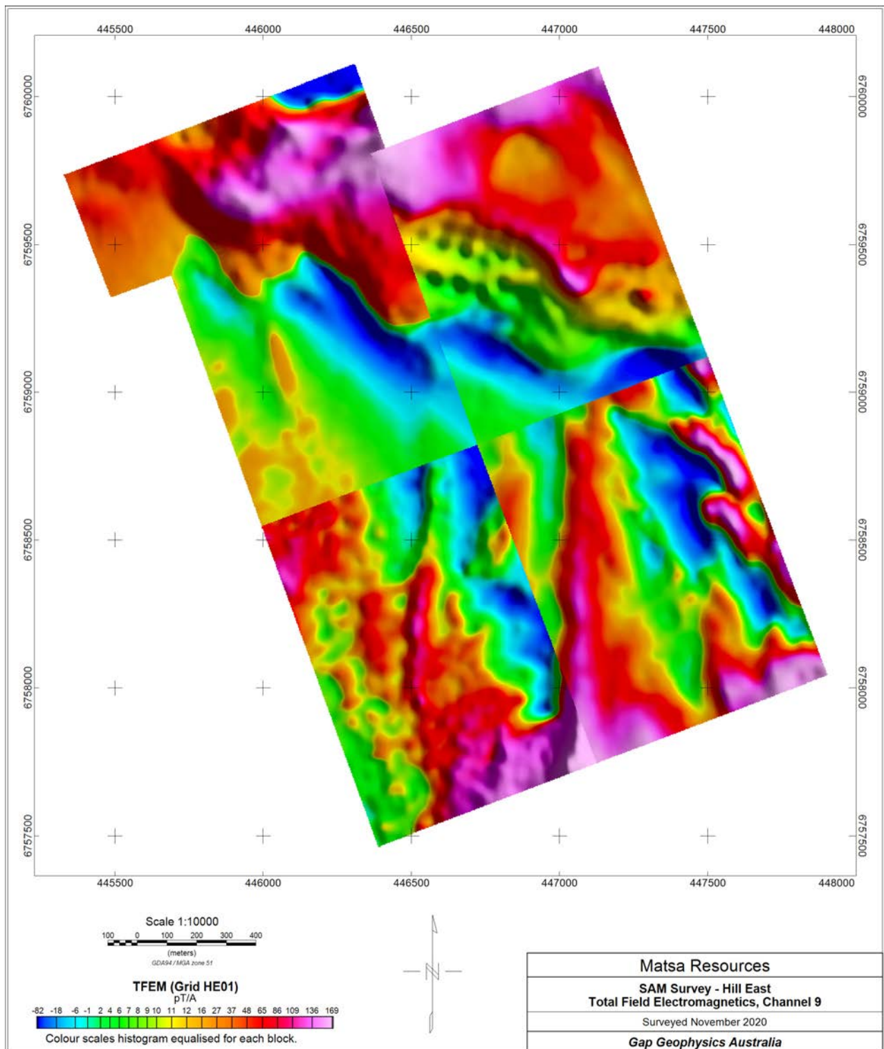
Figure 14 Hill East – total field electromagnetics, channel 9, mosaic.
