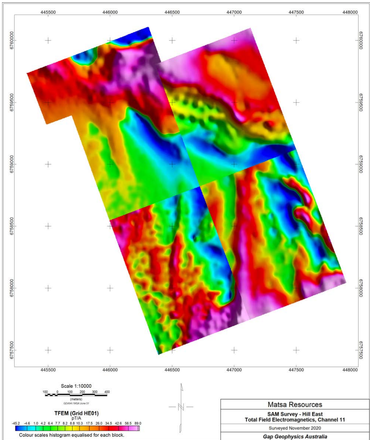
Figure 16 Hill East – total field electromagnetics, channel 11, mosaic.
