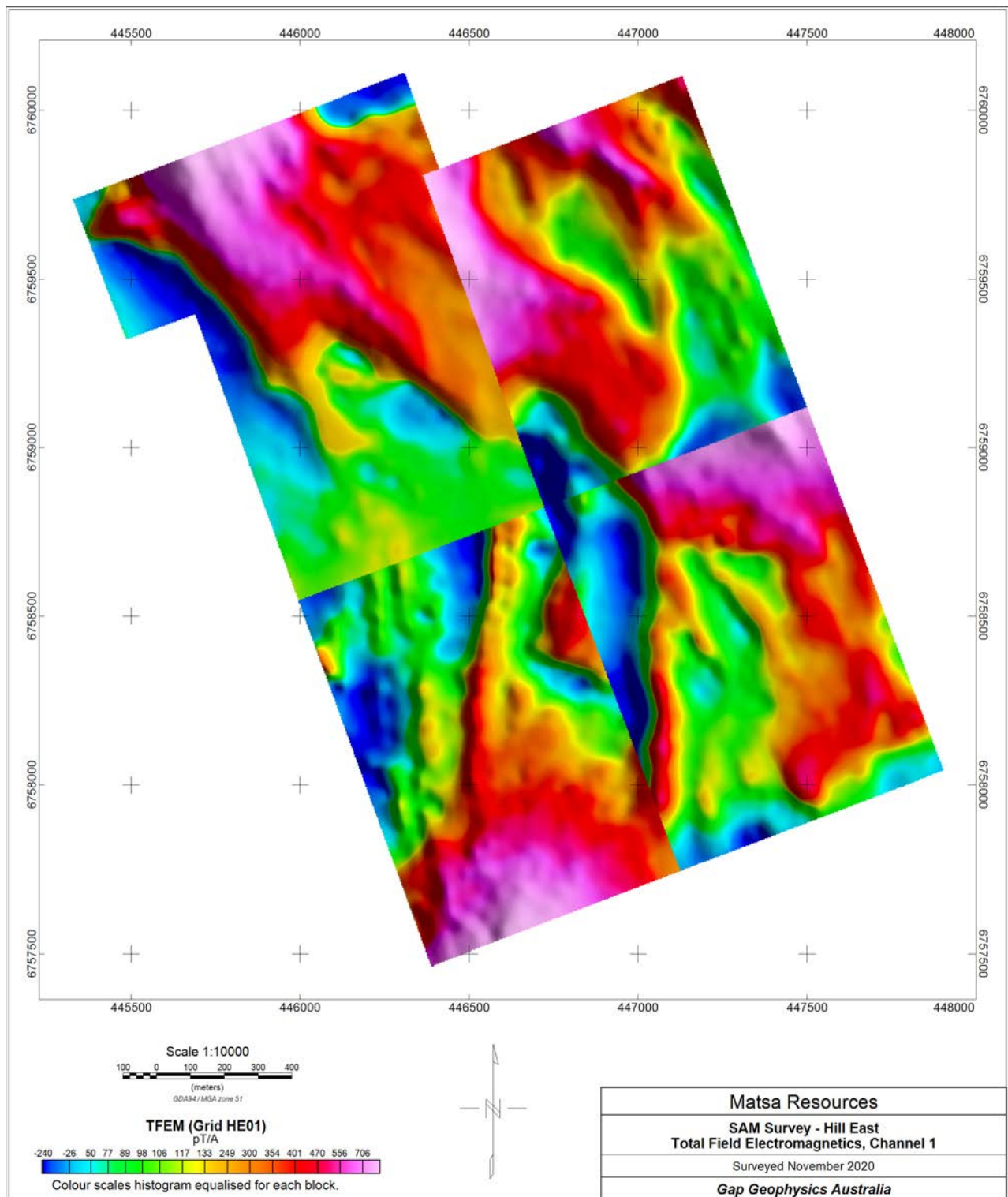
Figure 6 Hill East – total field electromagnetics, channel 1, mosaic.
