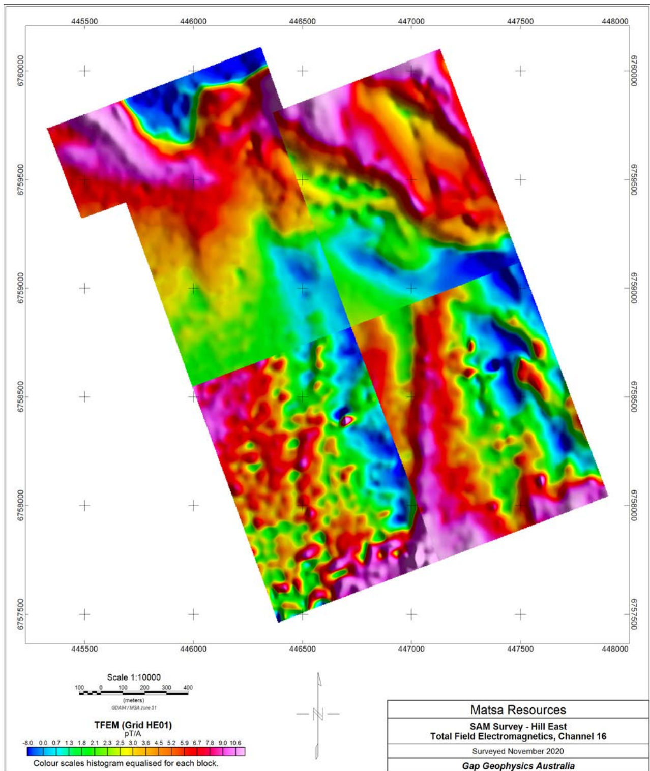
Figure 21 Hill East – total field electromagnetics, channel 16, mosaic.
