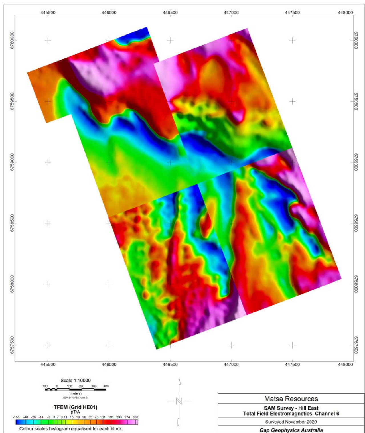
Figure 11 Hill East – total field electromagnetics, channel 6, mosaic.
