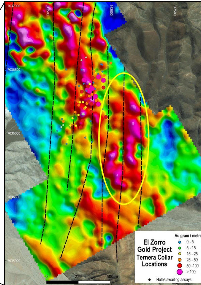
Ternerera Prospect Potential Ternerera repeat IP Anomaly in yellow circle
