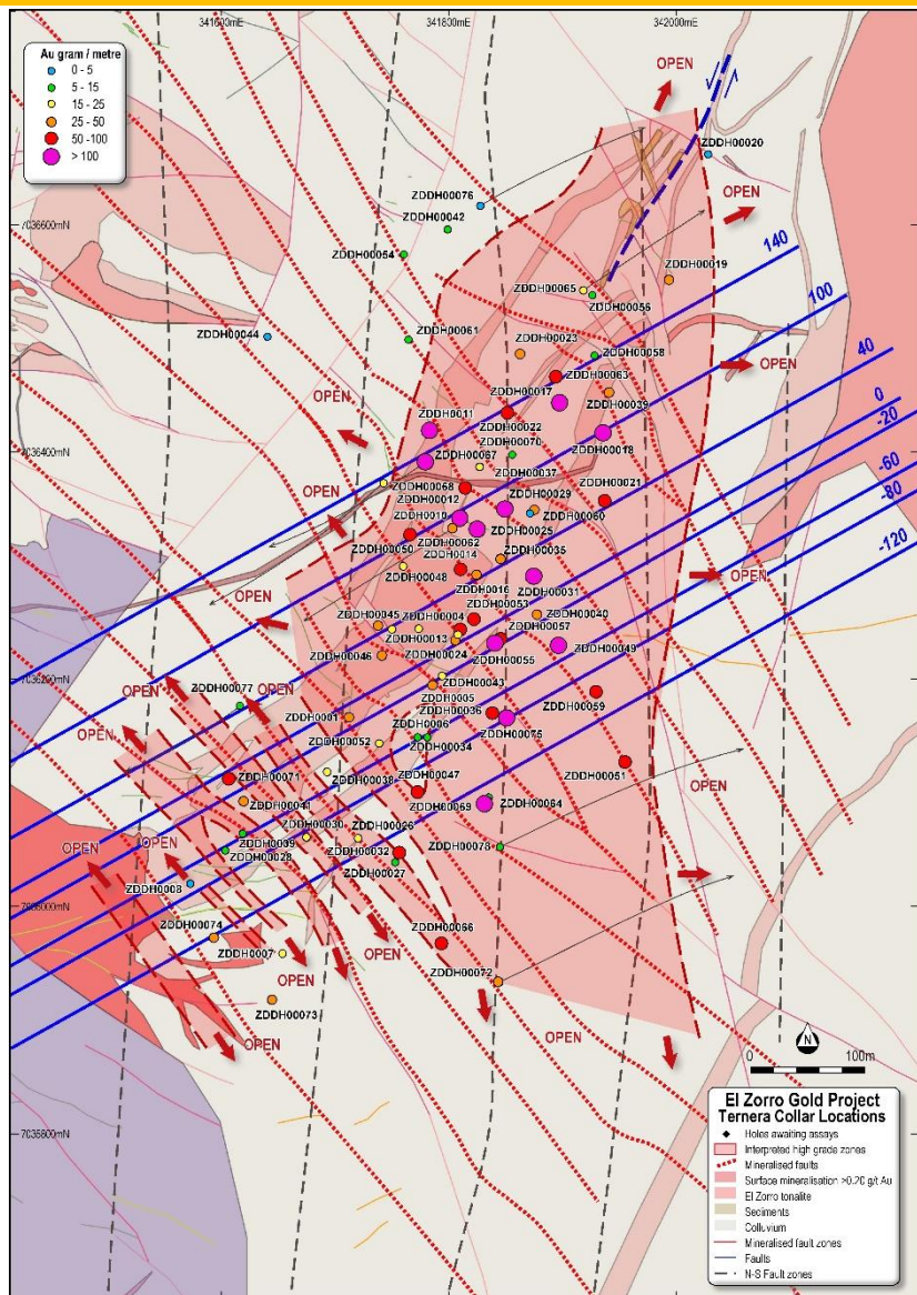
Ternerera Prospect Surface geology and drill collars Blue Lines show section locations
