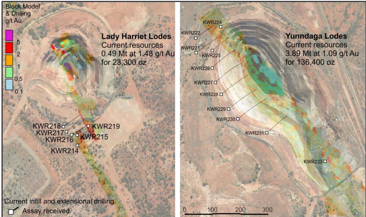
Figure 3: Plan showing all new drill holes within the Lady Harriet and Yunddaga Systems on resource block model background
