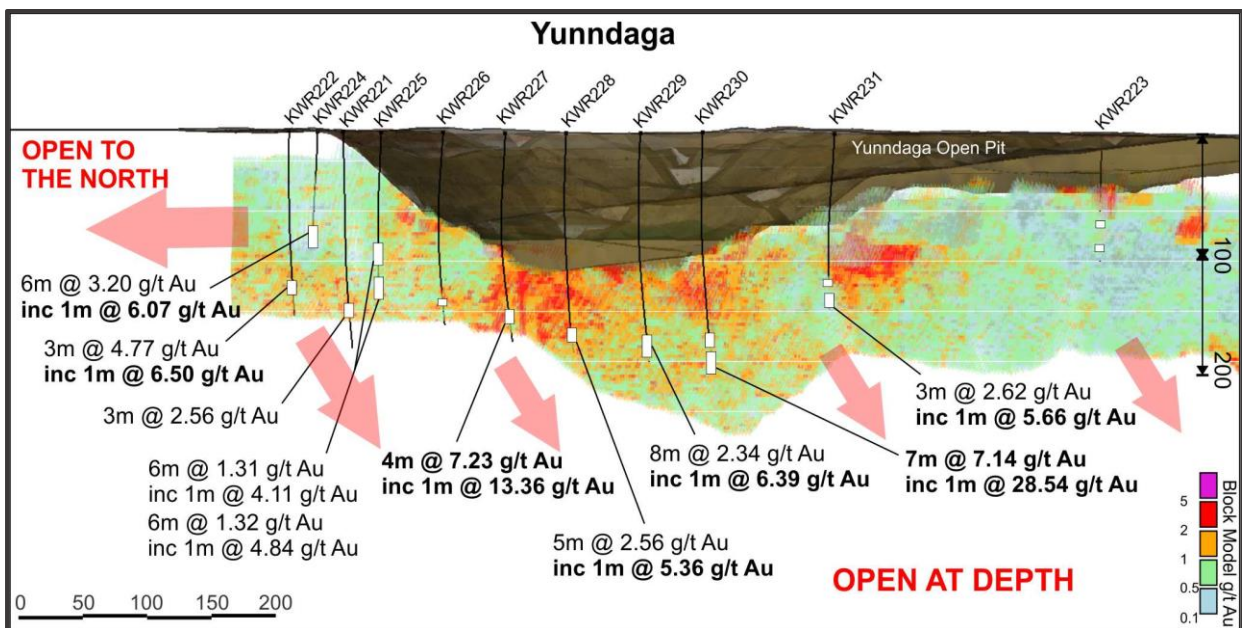
Figure 4: Yunddaga long section with new drill holes and MRE block model background
