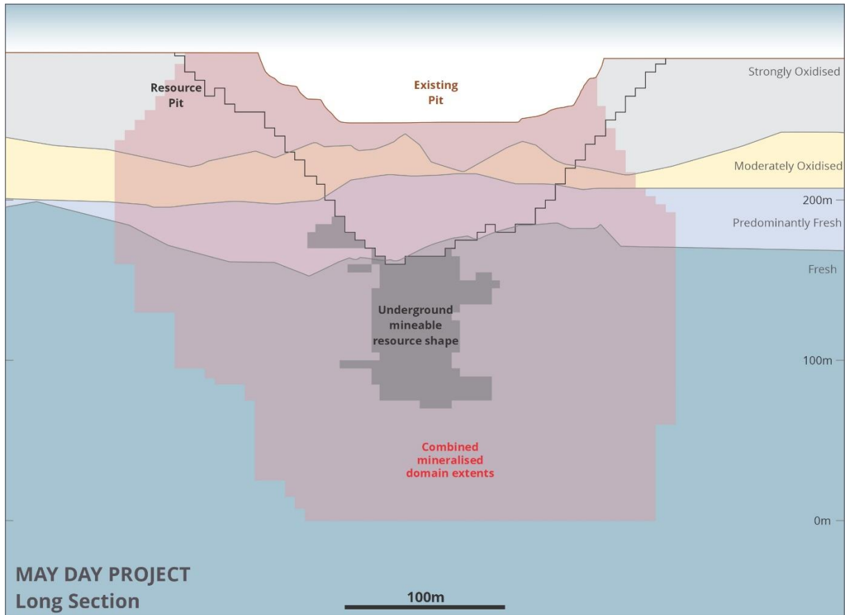
Figure 3 – May Day pit optimisation long section
