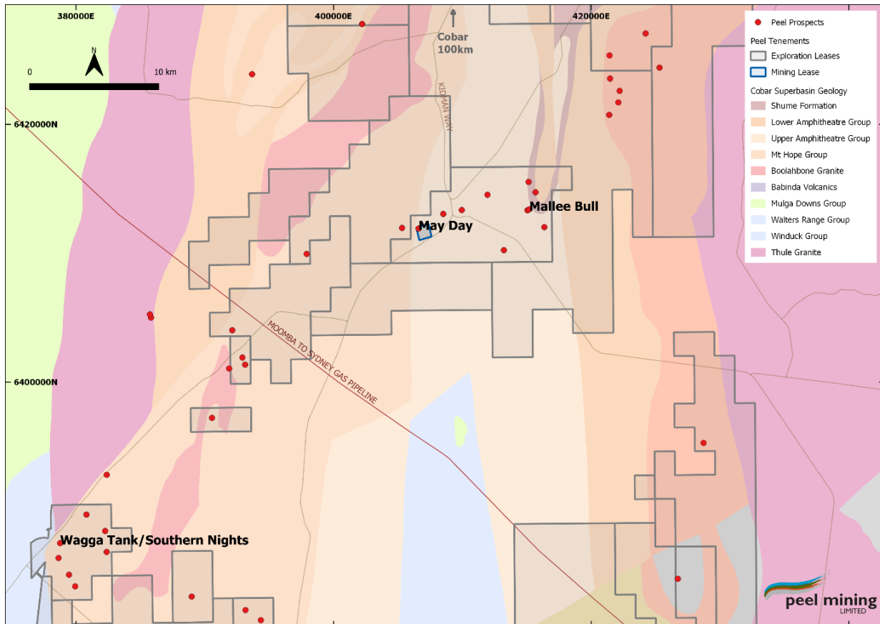
Figure 1 – Location of May Day deposit, Gilgunnia NSW
