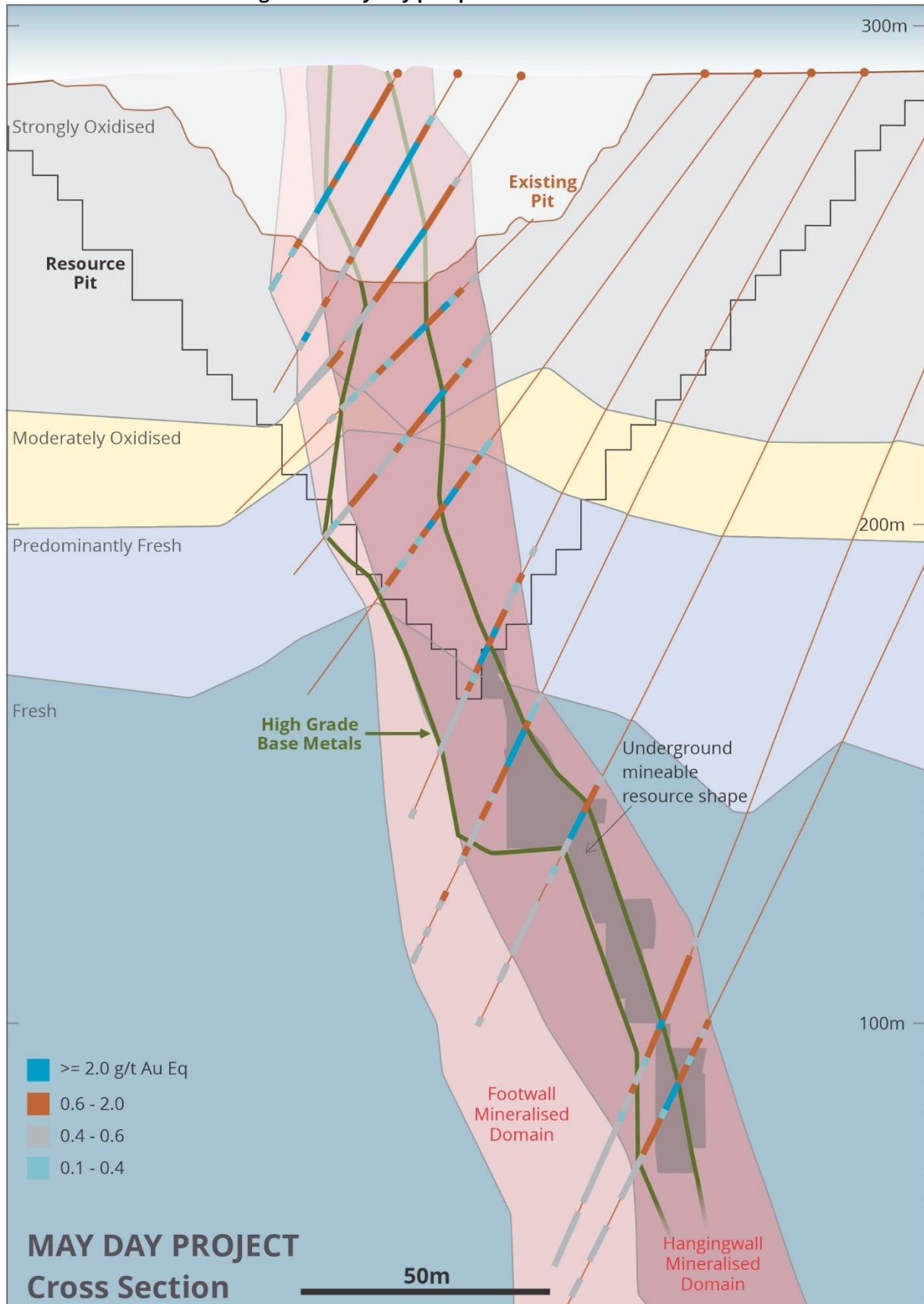
Figure 2 – May Day pit optimisation cross section
