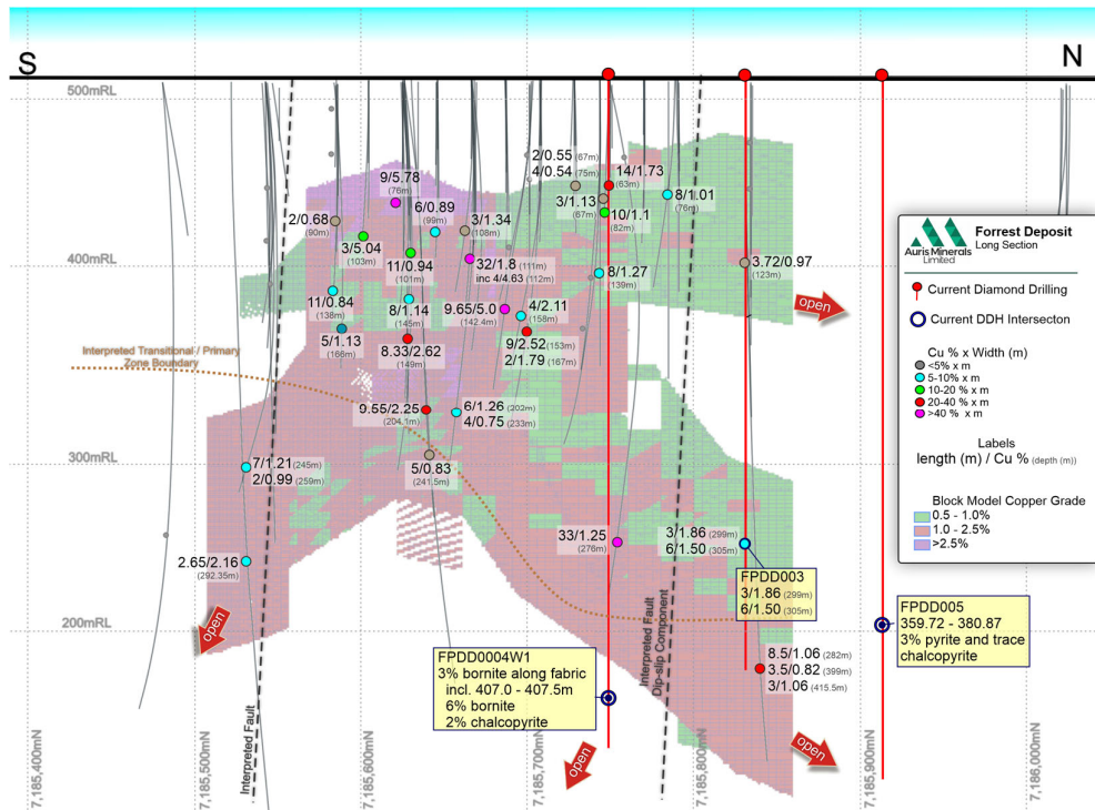
Figure 1 -Forrest Deposit Longitudinal Projection
