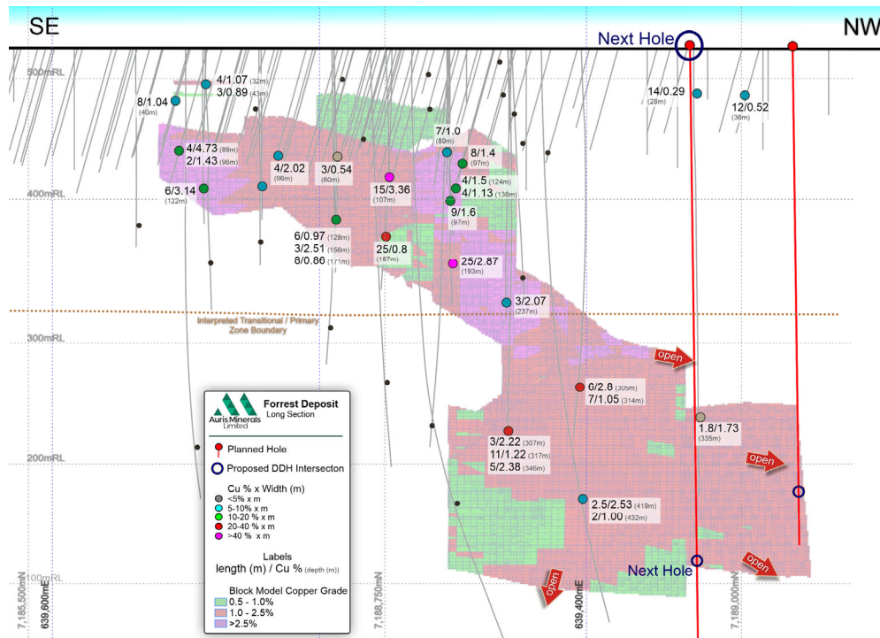
Figure 3 -Wodger Deposit Longitudinal Projection
