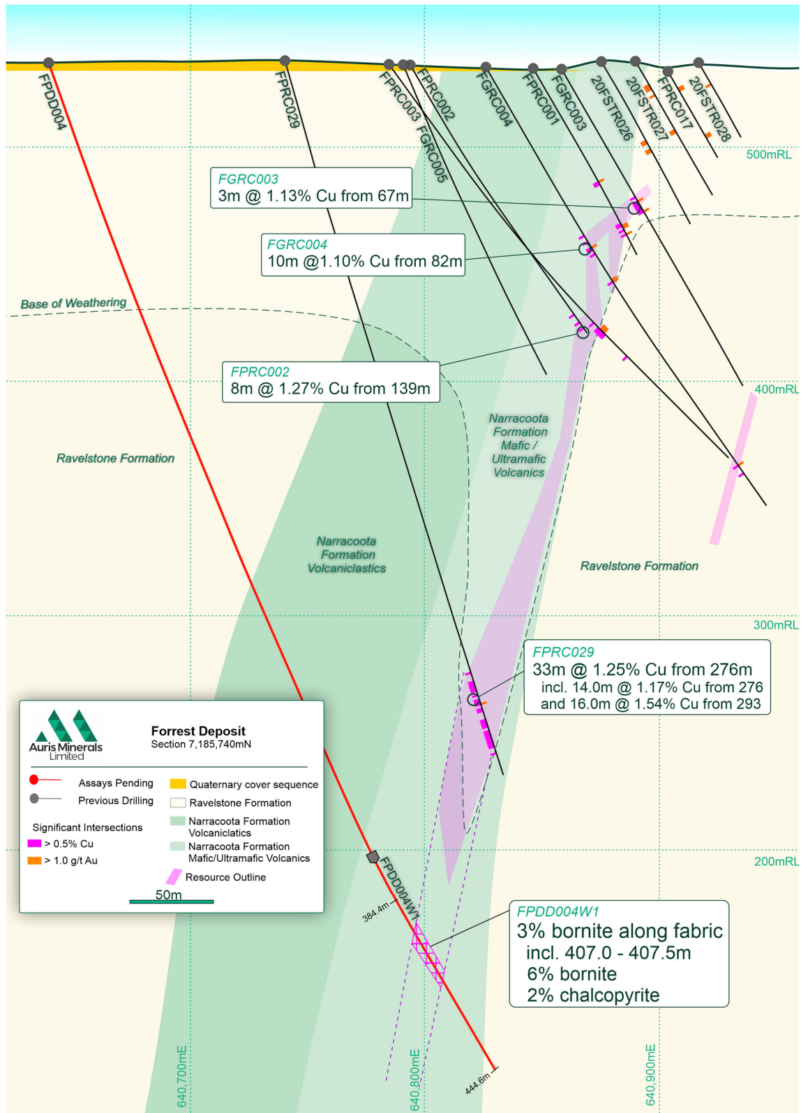
Figure 2 -Forrest Deposit Cross Section 7,185,740mN
