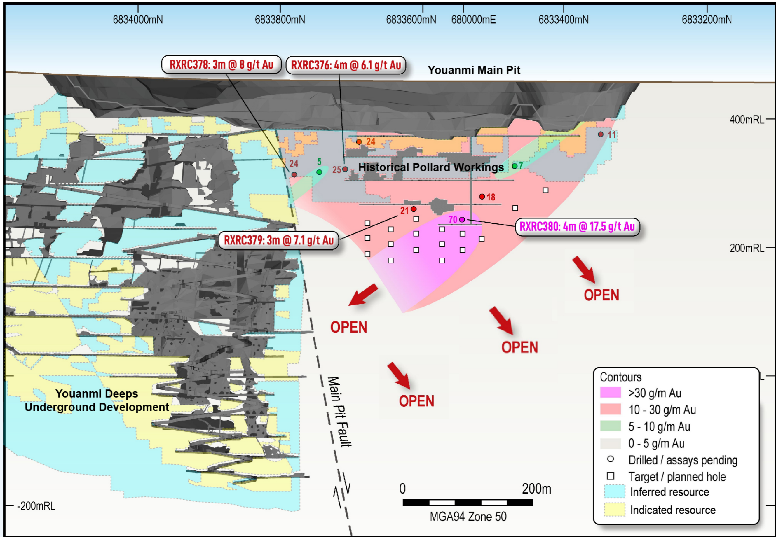
Figure 2. Junction Long Section – Rox intersections and Au gram-metre contours
