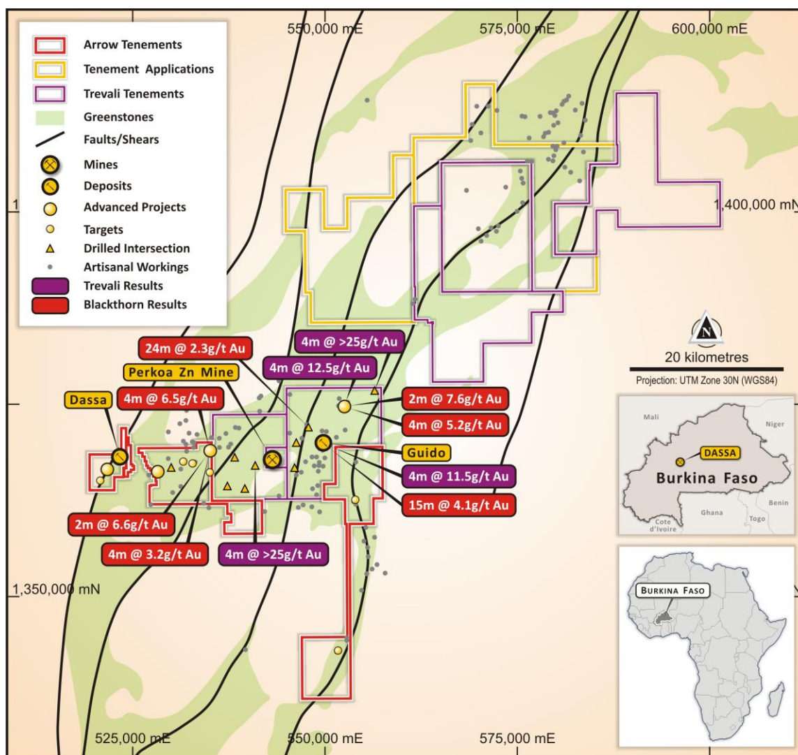
Figure 1: Boromo Belt with Arrow permits, Trevali permits, and targets for 2021
