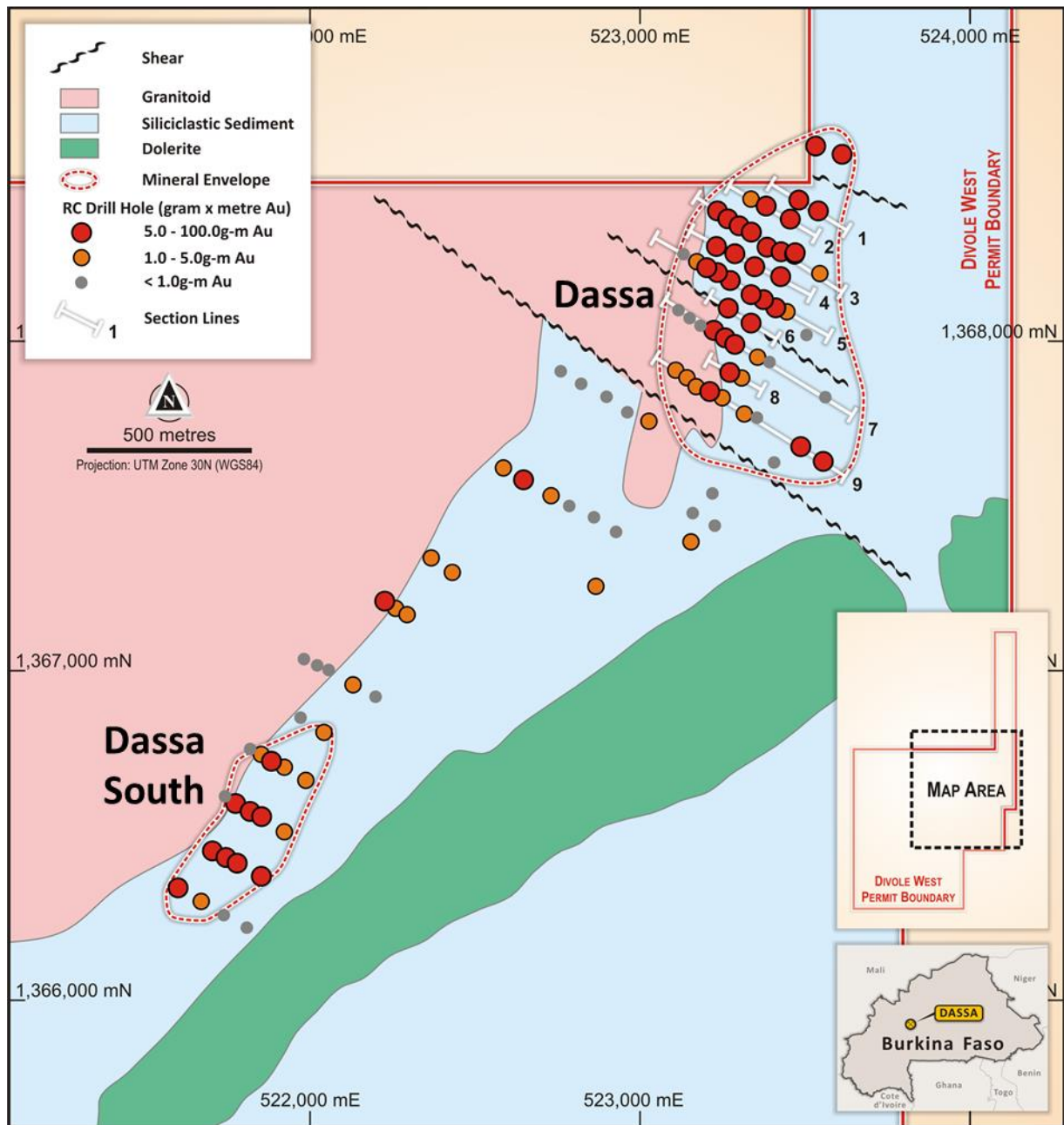
Figure 2: Dassa deposit with drilling completed by Arrow Minerals
