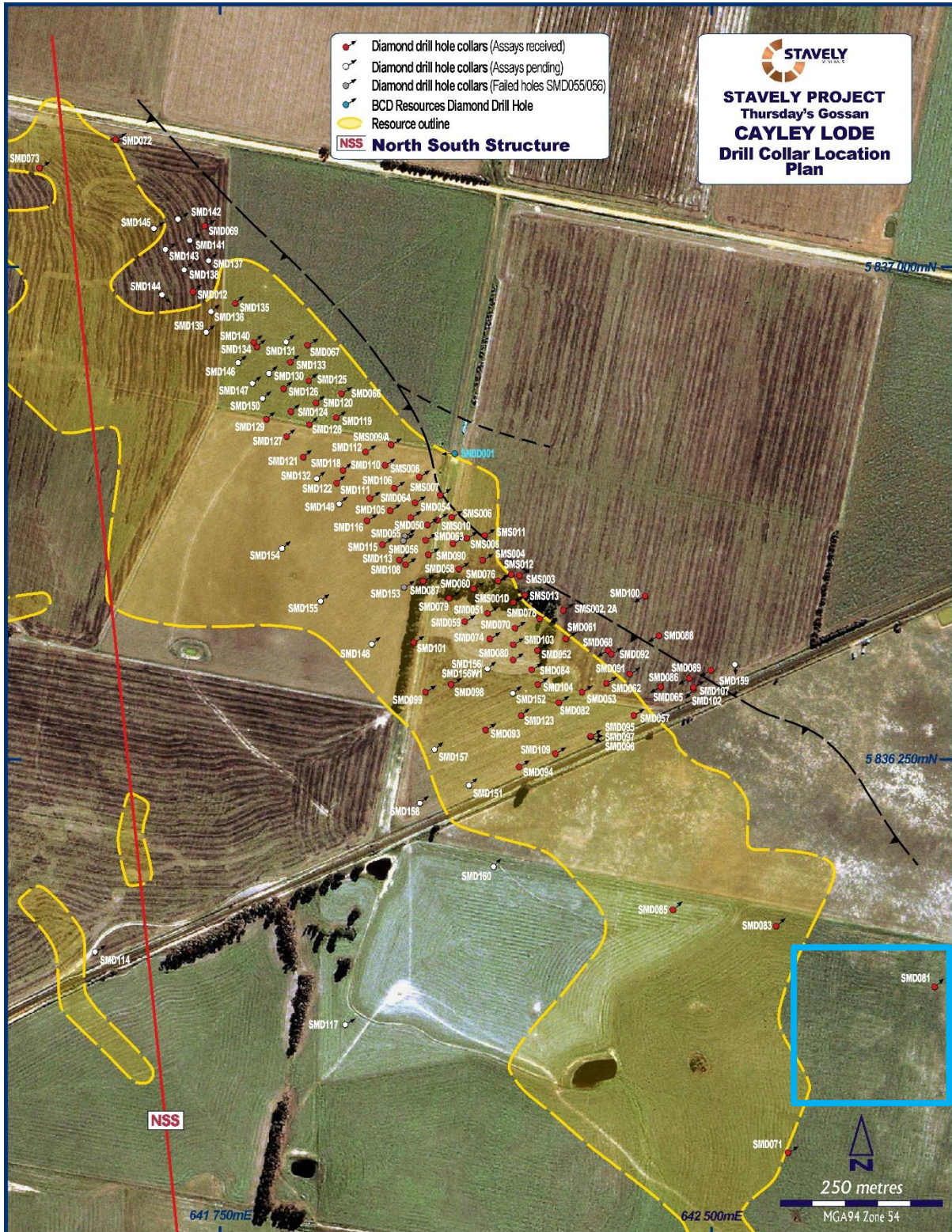
Figure 3. Thursday’s Gossan drill collar location plan showing the location of planned drilling.
