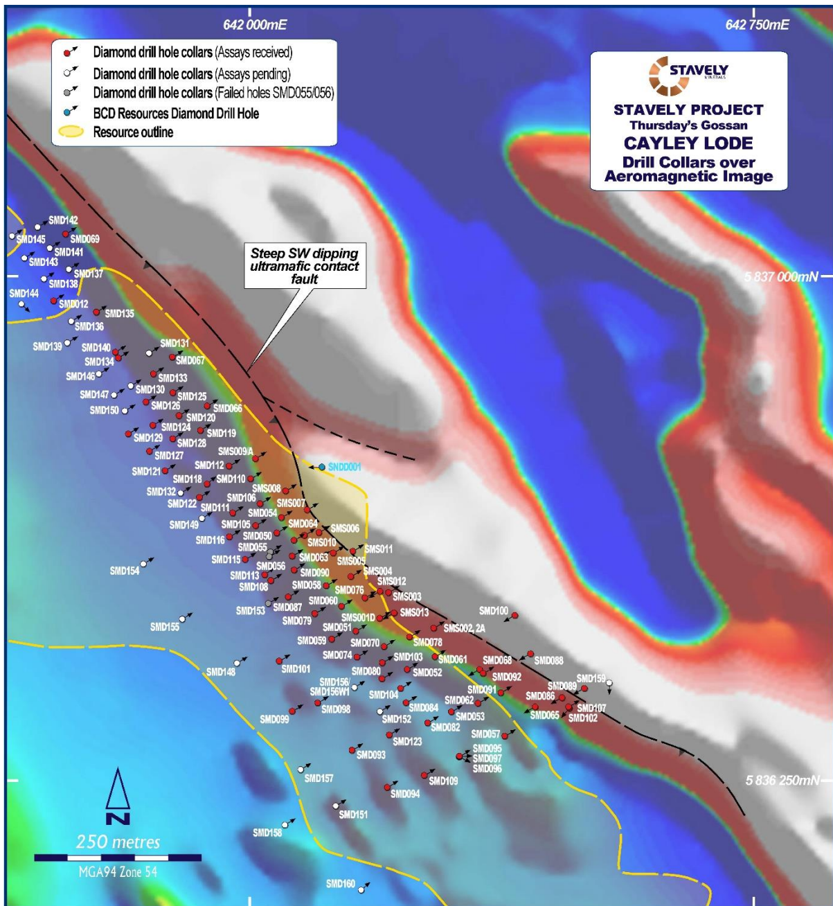
Figure 4. Aeromagnetic image with drill collar locations.
