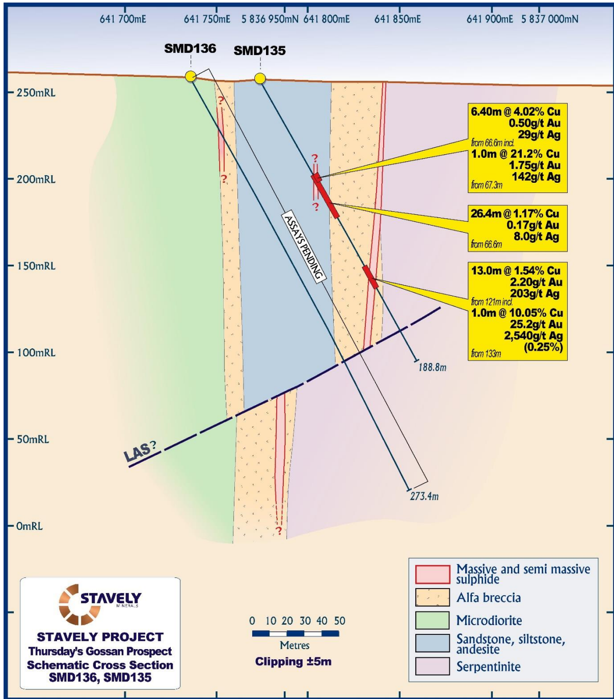
Figure 5. SMD135 drill section.
