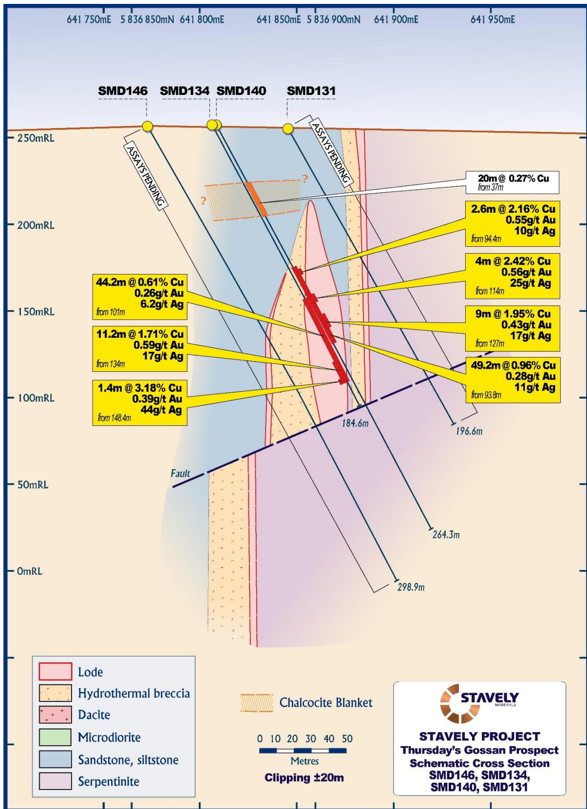
Figure 6. SMD134 and SMD140 drill section.
