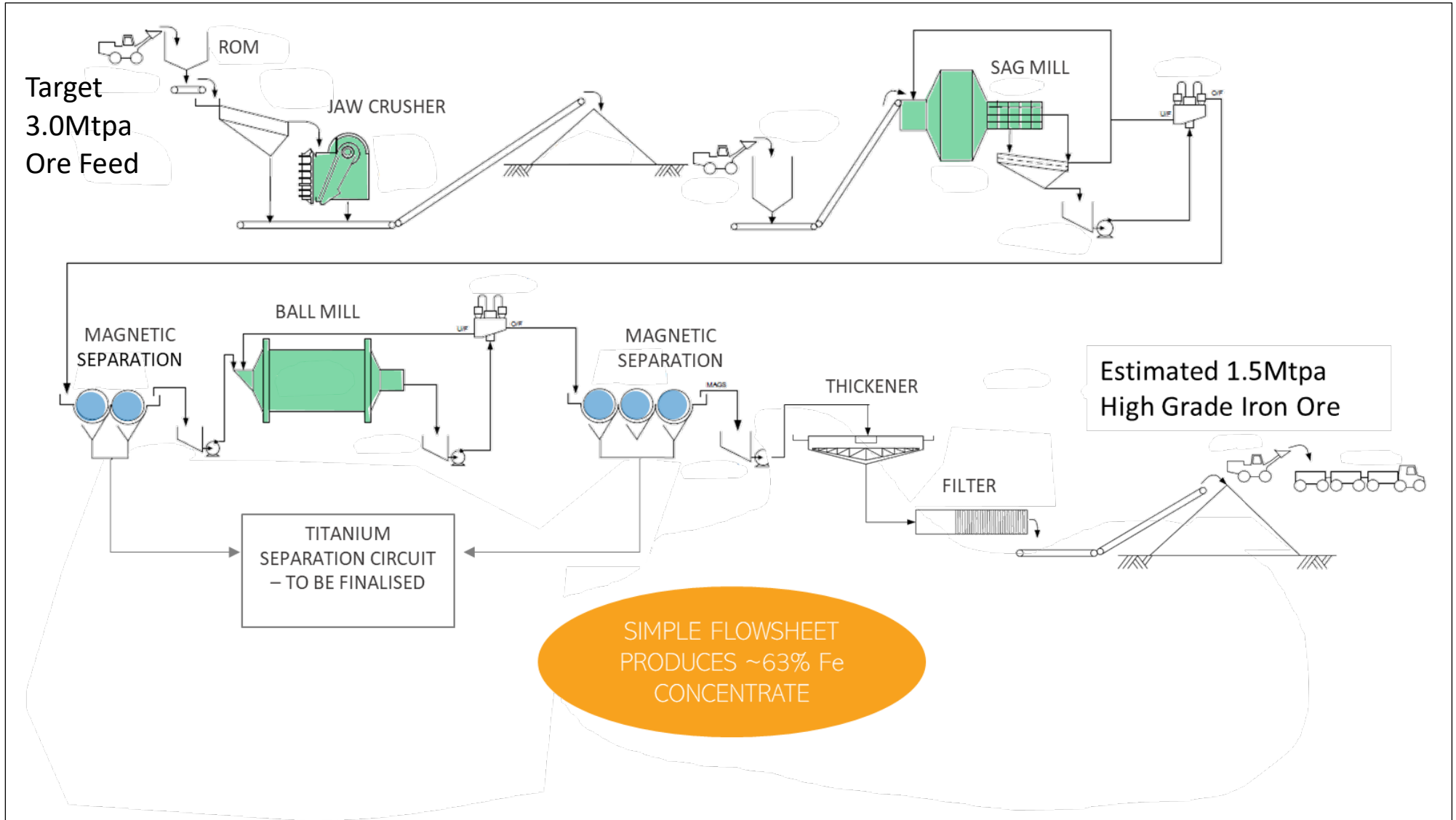
Figure 1: Yarrabubba Indicative CMB Flowsheet
