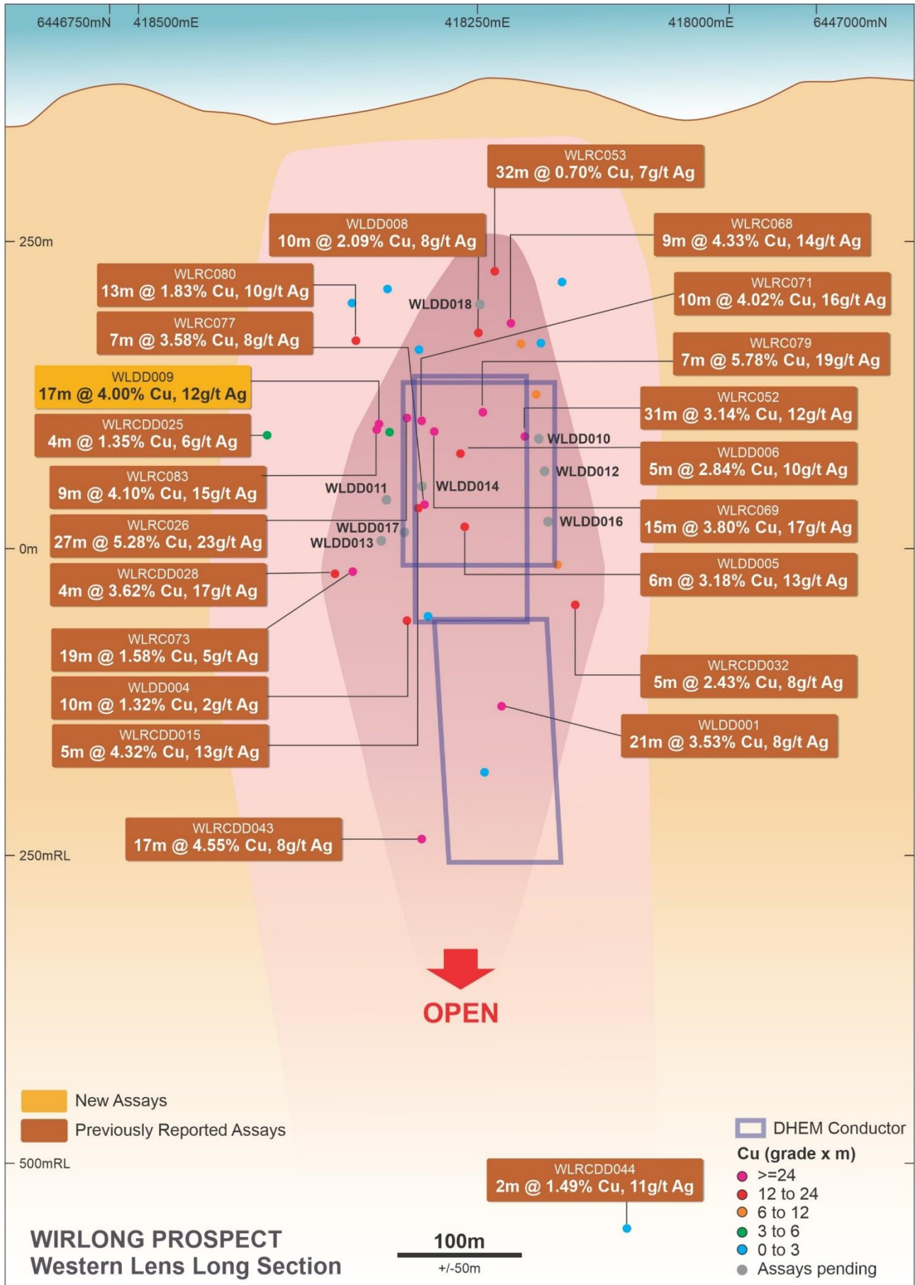
Figure 3 – Wirlong Western Lens Long Section
