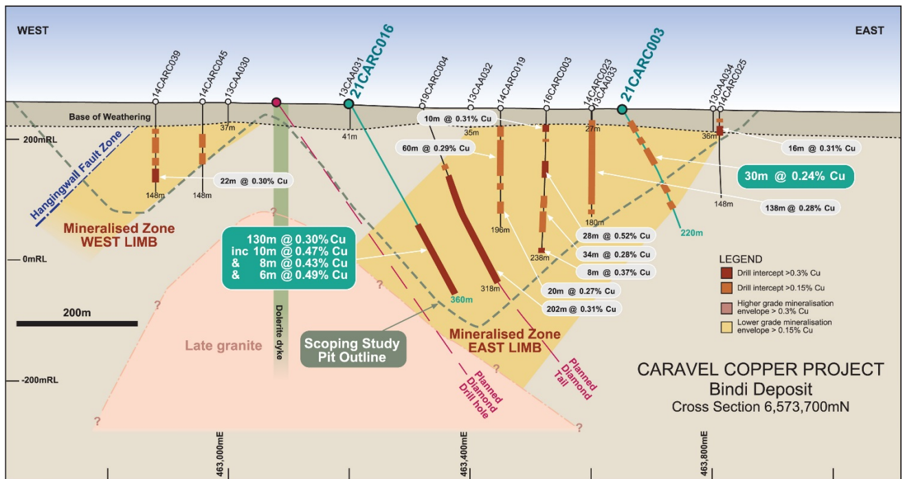
Figure 3: Schematic geological cross section of the Bindi Deposit (6,573,700mN) showing location of recent RC percussion (CARC prefix) drill holes.
