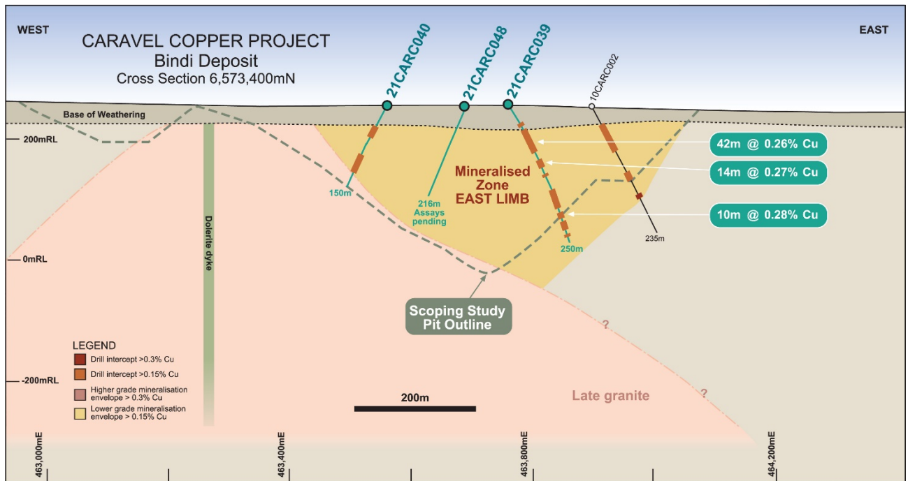
Figure 6: Schematic geological cross section of the Bindi Deposit (6,573,400mN) showing location of recent RC percussion (CARC prefix) drill holes.
