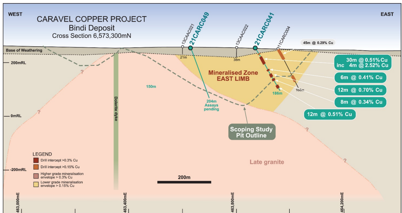
Figure 7: Schematic geological cross section of the Bindi Deposit (6,573,300mN) showing location of recent RC percussion (CARC prefix) drill holes. Note that 21CARC049 is drilled oblique to the plane of the cross section.
