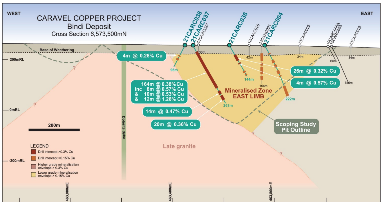
Figure 5: Schematic geological cross section of the Bindi Deposit (6,573,500mN) showing location of recent RC percussion (CARC prefix) drill holes.
