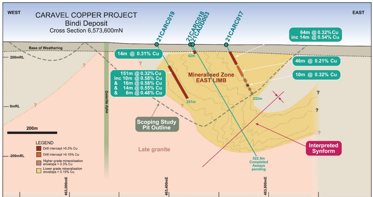
Figure 4: Schematic geological cross section of the Bindi Deposit (6,573,600mN) showing location of recent RC percussion (CARC prefix) and diamond (CADD prefix) drill holes.
