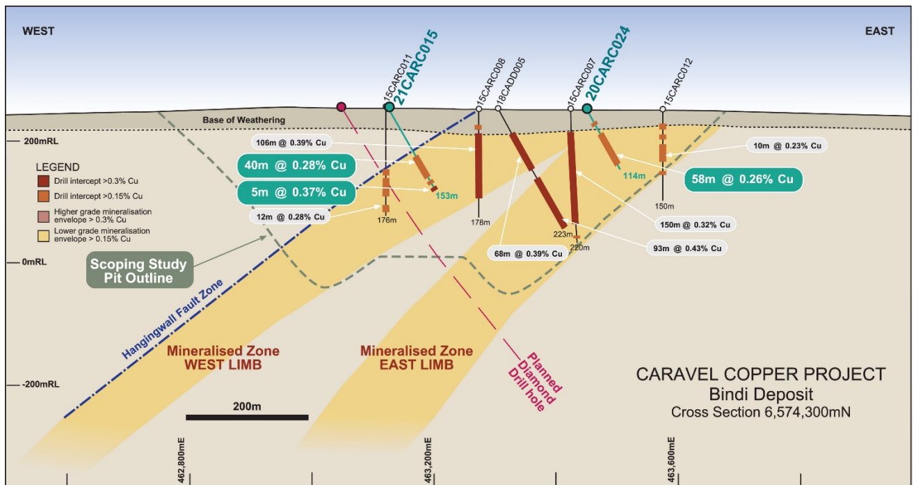
Figure 2: Schematic geological cross section of the Bindi Deposit (6,574,300mN) showing location of recent RC percussion (CARC prefix) drill holes.
