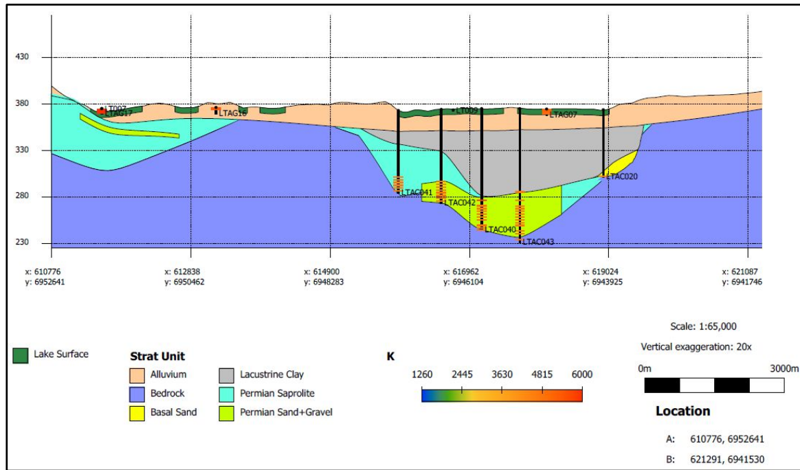
Figure 7: Geological cross section at Lake Throssell South
