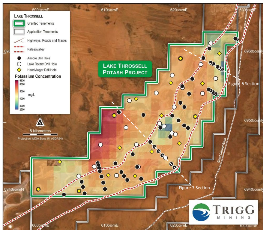
Figure 8: Lake Throssell shallow potassium grade distribution and sample points (370mRL depth slice)
