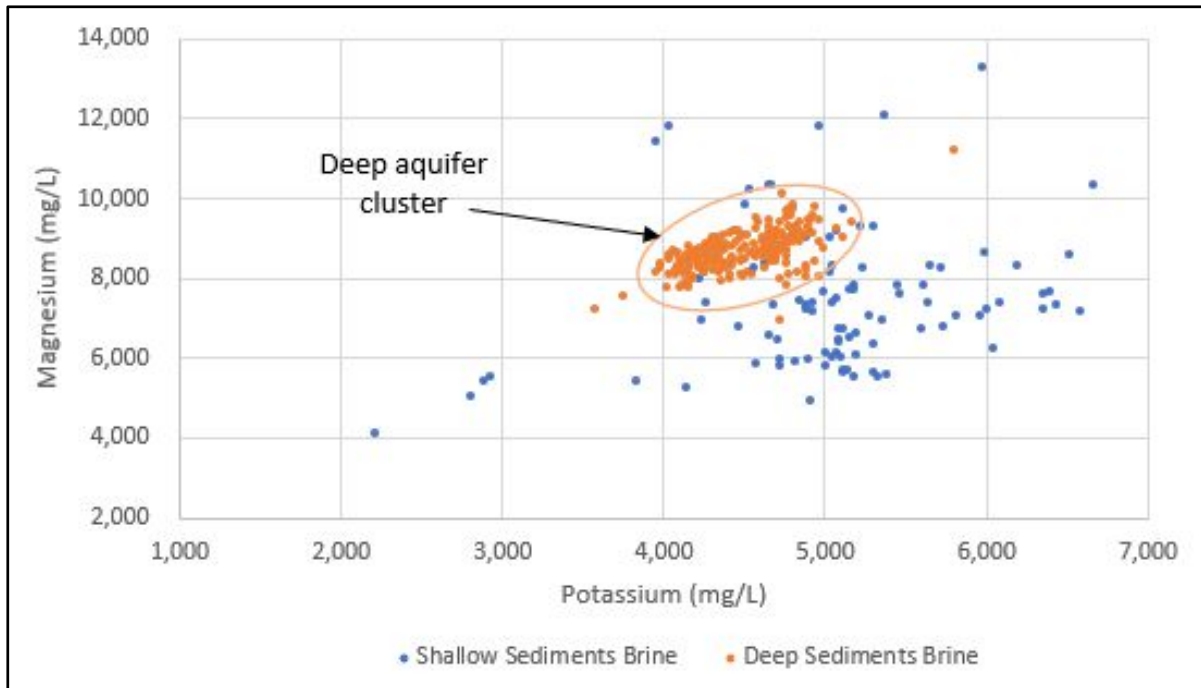
Figure 5: Potassium magnesium concentrations for the lake surface and deep brine aquifers
