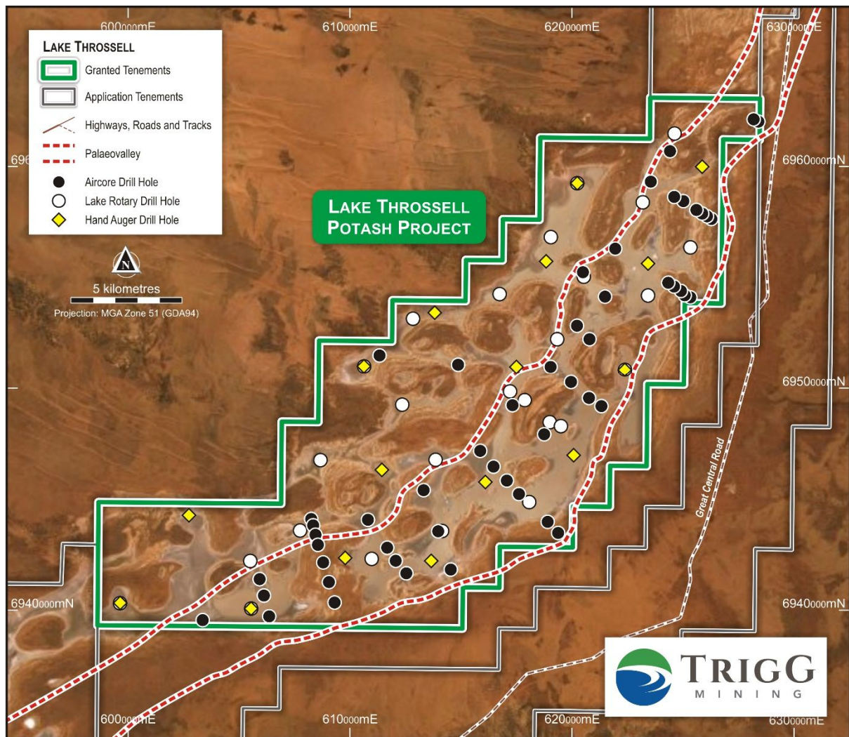
Figure 1: Lake Throssell investigation locations
