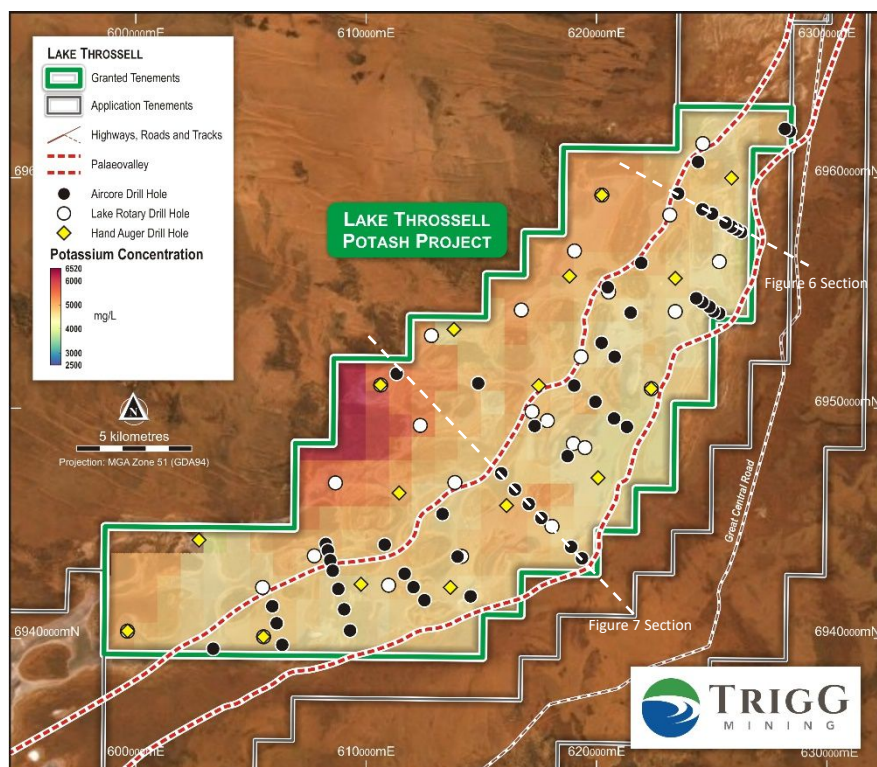
Figure 9: Lake Throssell deep potassium grade distribution and sample points (280mRL depth slice)
