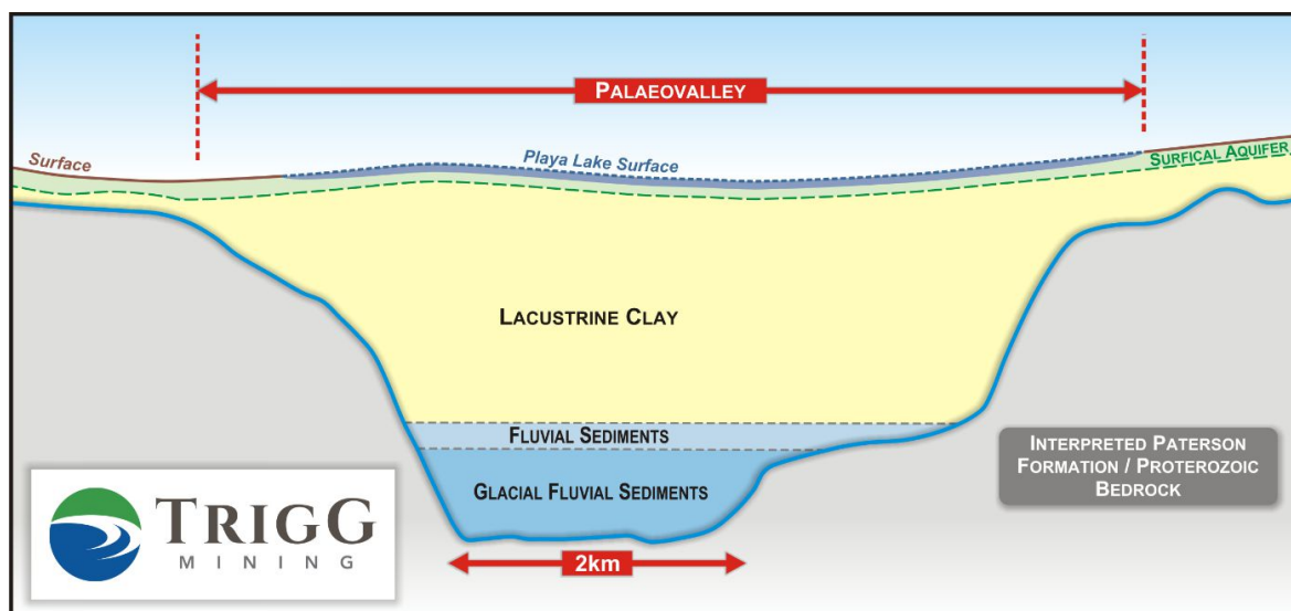
Figure 3: Schematic cross section of the palaeovalley sequence at Lake Throssell
