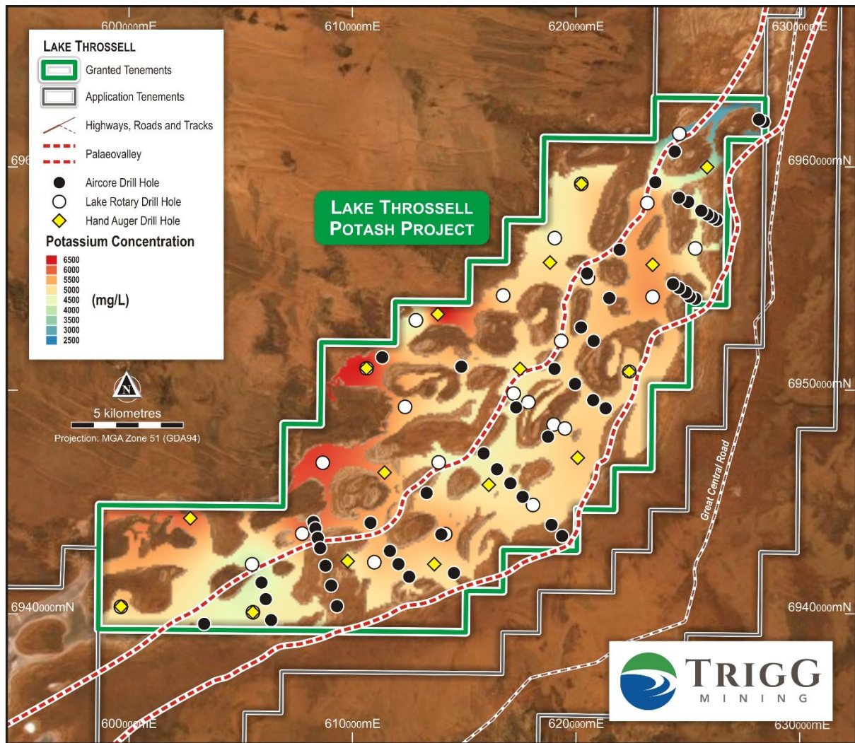
Figure 4: Potassium concentration at the lake surface
