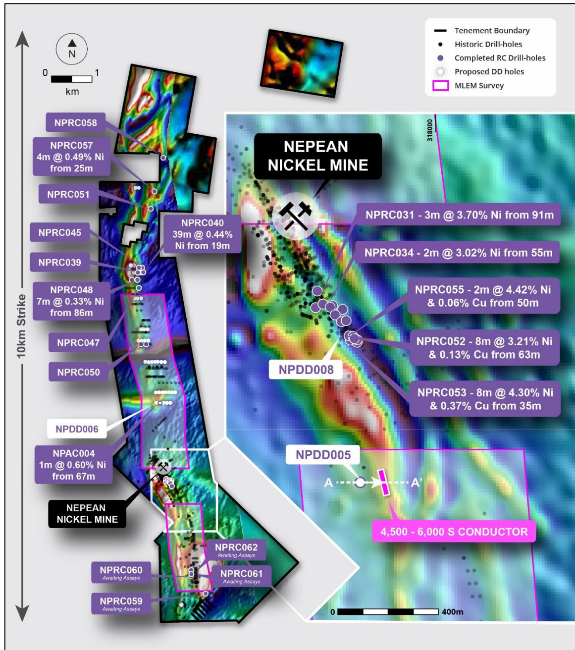
Figure 1 – Plan map of aeromagnetics over the Nepean Nickel Project showing new diamond drill collars in relation to RC drill collars and the MLEM conductor to the south of the historic Nepean nickel mine
