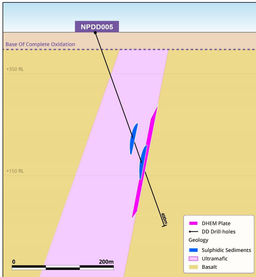
Figure 2 – Cross-section A – A' (see Figure 1) showing completed diamond drill-hole NPDD005 and the modelled DHEM conductor in relation to the modelled ultramafic unit, sulphidic sediments and interpreted footwall contact
