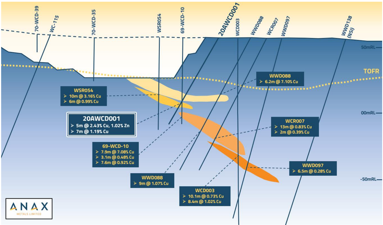
Figure 2: Oblique cross-section (looking towards 305^\circ ) showing 20AWCD001, select previous drill holes and interpreted copper domains. Refer to Figure 1 for approximate cross-section location. Note: A number of holes have been omitted from the section for ease of display.
