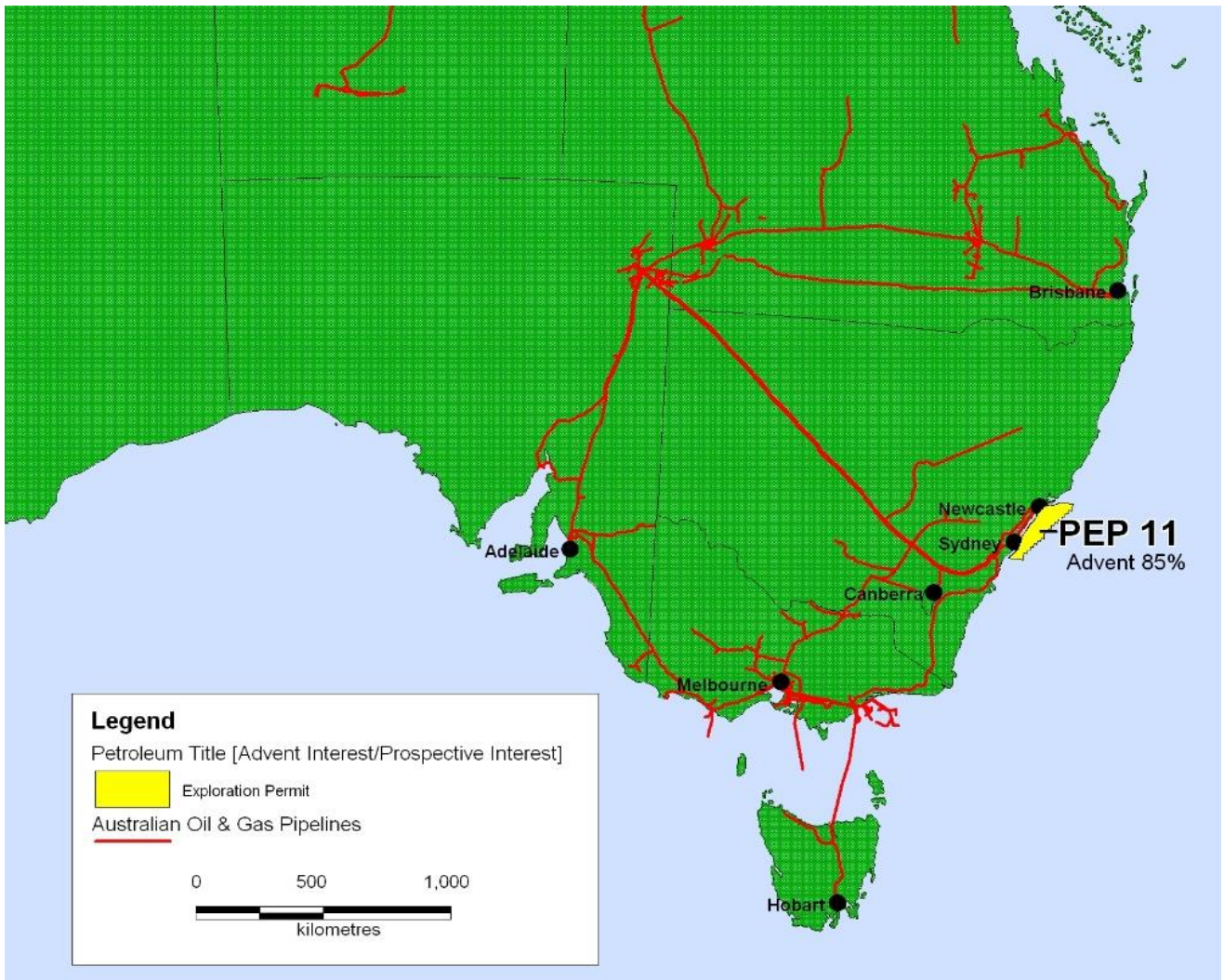
Location of Block PEP 11 offshore Australia (above) and location of Baleen well site (Location marked DM below)
