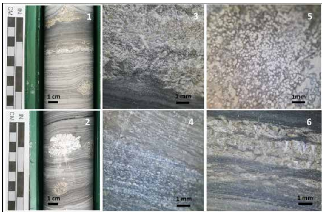
Figure 8-8: Close-up photographs of some of the searlesite crystals and textures from REK_002
