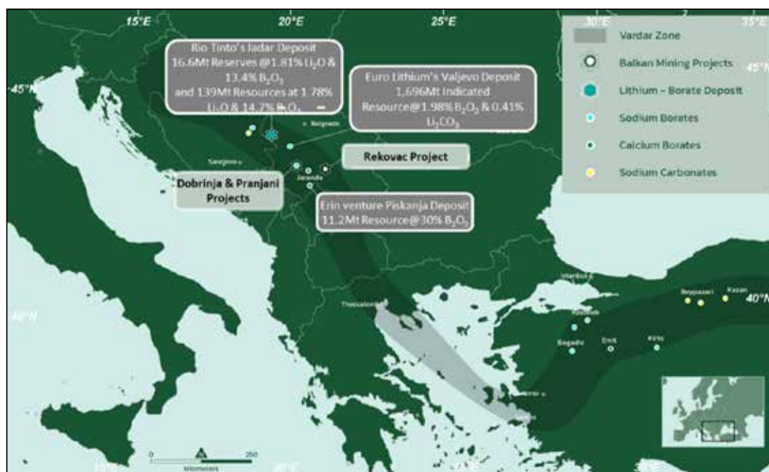
Figure 5-1: Map showing the extent of the Vardar Zone and associated mineralisation
