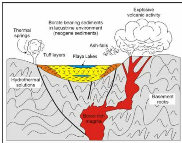
Figure 7-2: Schematic playa-lake in western Anatolia, Turkey – a depositional model for borate deposits
