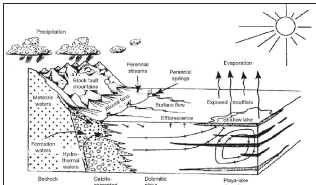
Figure 7-3: The Kramer Borax deposit, USA – a schematic playa-lake palaeo-depositional environment and model
