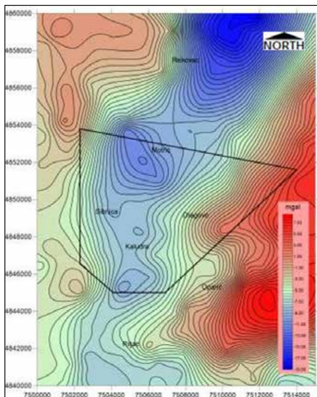
Figure 8-11: Map of the processed gravity data showing the Bouguer anomalies with a density of 2.20 \text{ g/cm}^3 for the Rekovac licence within the Rekovac Project
