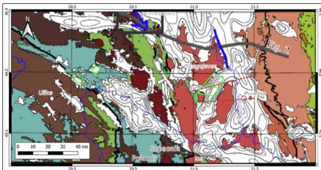
Figure 6-2: Regional map showing the location of the project areas within the regional tectonic setting of Serbia; the white contoured areas represent the Neogene sedimentary basins
