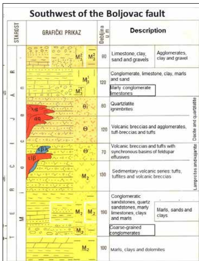
Figure 8-21: Generalised stratigraphy of the Miocene sediments within the Pranjani and Dobrinja basins (see Figure 8-20 for geological map)
