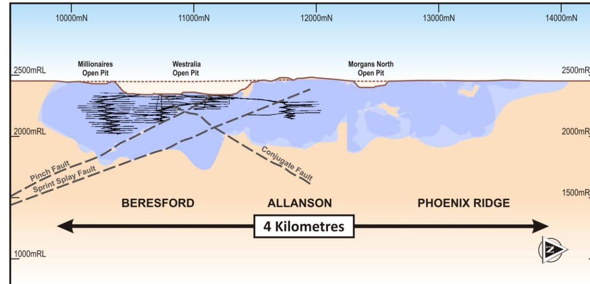
Long-Section of the Westralia Underground
