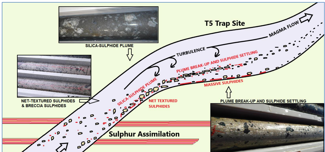
Figure 3: Geological interpretation of the T5 pyroxenitic feeder zone trap site. This image is not to scale and the extent of the T5 mineralisation has not been found to date.
