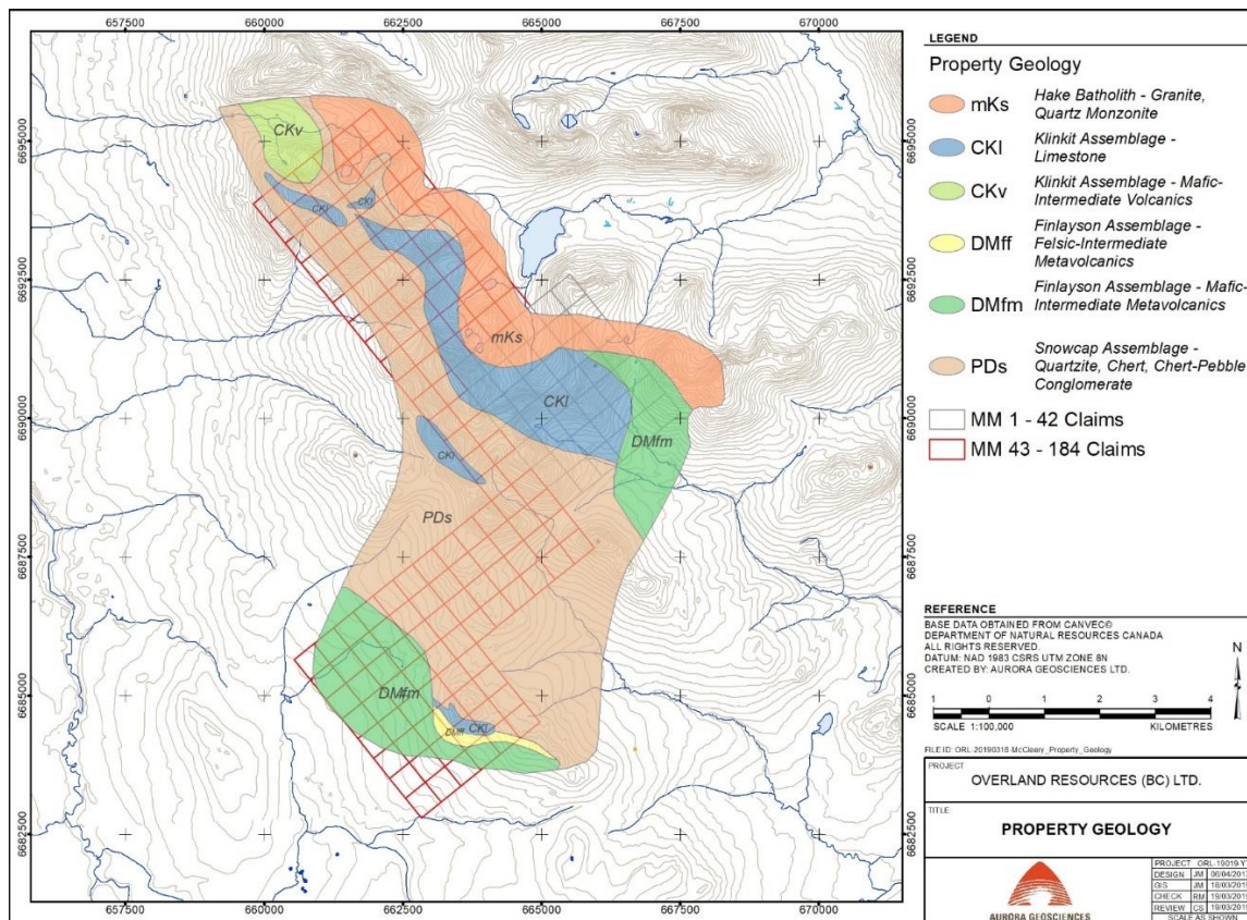
Figure 1: Property Geology sketch, Mount McCleery area
