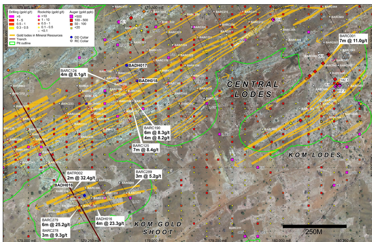
Figure 1. Plan depicting the location of new diamond holes BADH016, BADH017 and BADH018; previous DD/RC drill holes; and auger holes in the Central Lodes.
