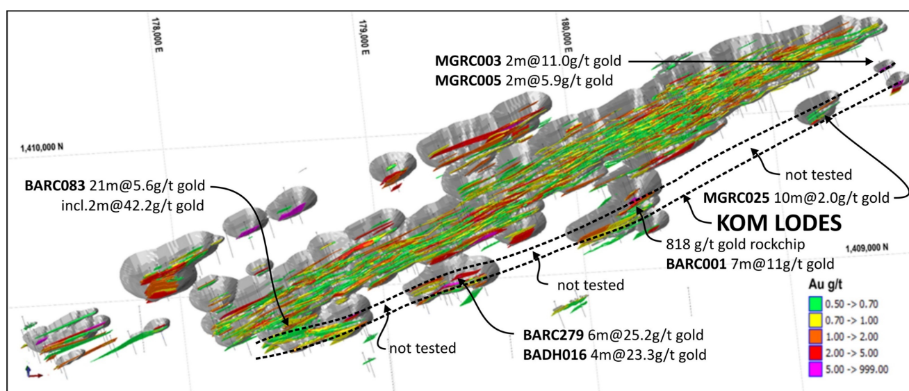
Figure 2. 3D Perspective view of the Mineral Resource blocks and constraining pits (grey) at the Central Lodes (1.9Moz at 1.2g/t gold) with the location of the Kom Gold Shoot. Resource blocks are coloured by gold grade in g/t.
