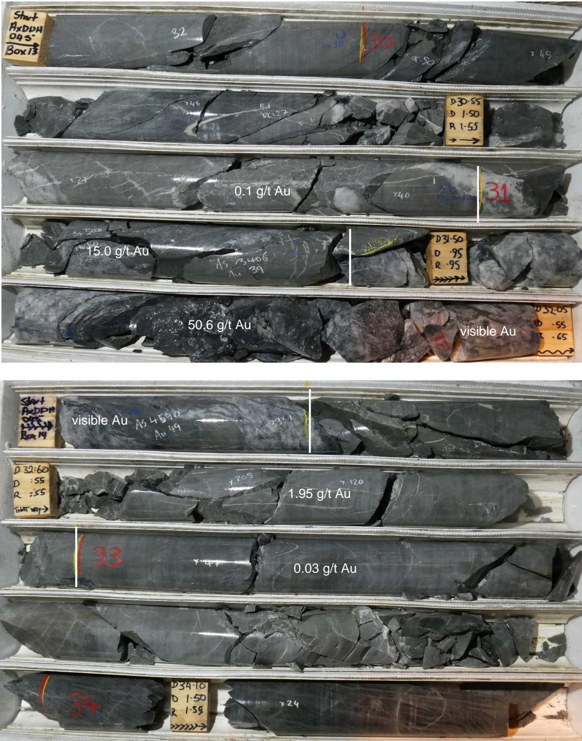
Figure 6. AX45 core with assays of 2.0m @ 26.8g/t Au
