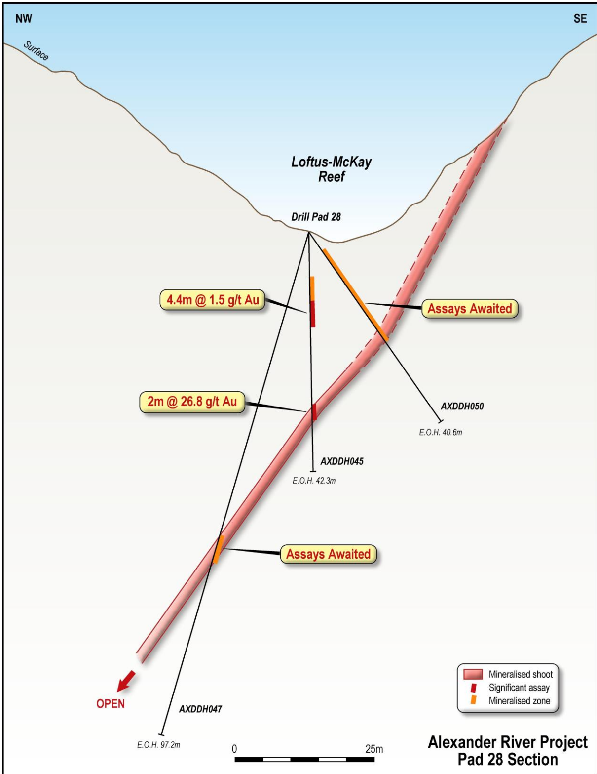
Figure 7. Cross section through AXDDH045, AXDDH047 and AXDDH050.
