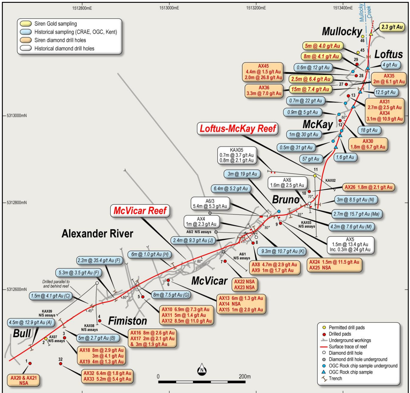
Figure 2. Plan of the trench and drillhole intersections.
