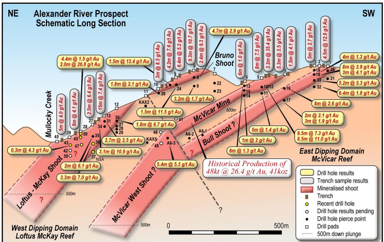
Figure 1. Schematic long section through Alexander reef system.
