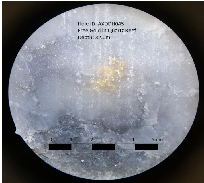
Figure 5. Abundant free gold in quartz between 31.5m and 32.4m in AXDDH045
