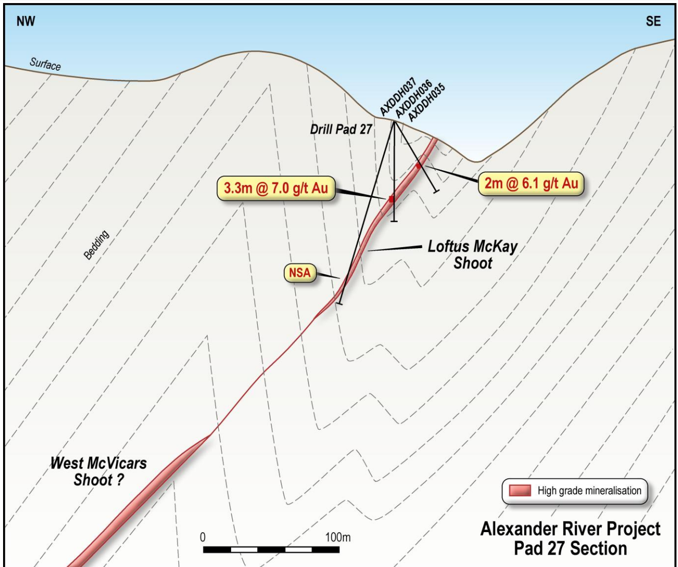
Figure 4 Cross section through AXDDH035, AXDDH036 and AXDDH037.
