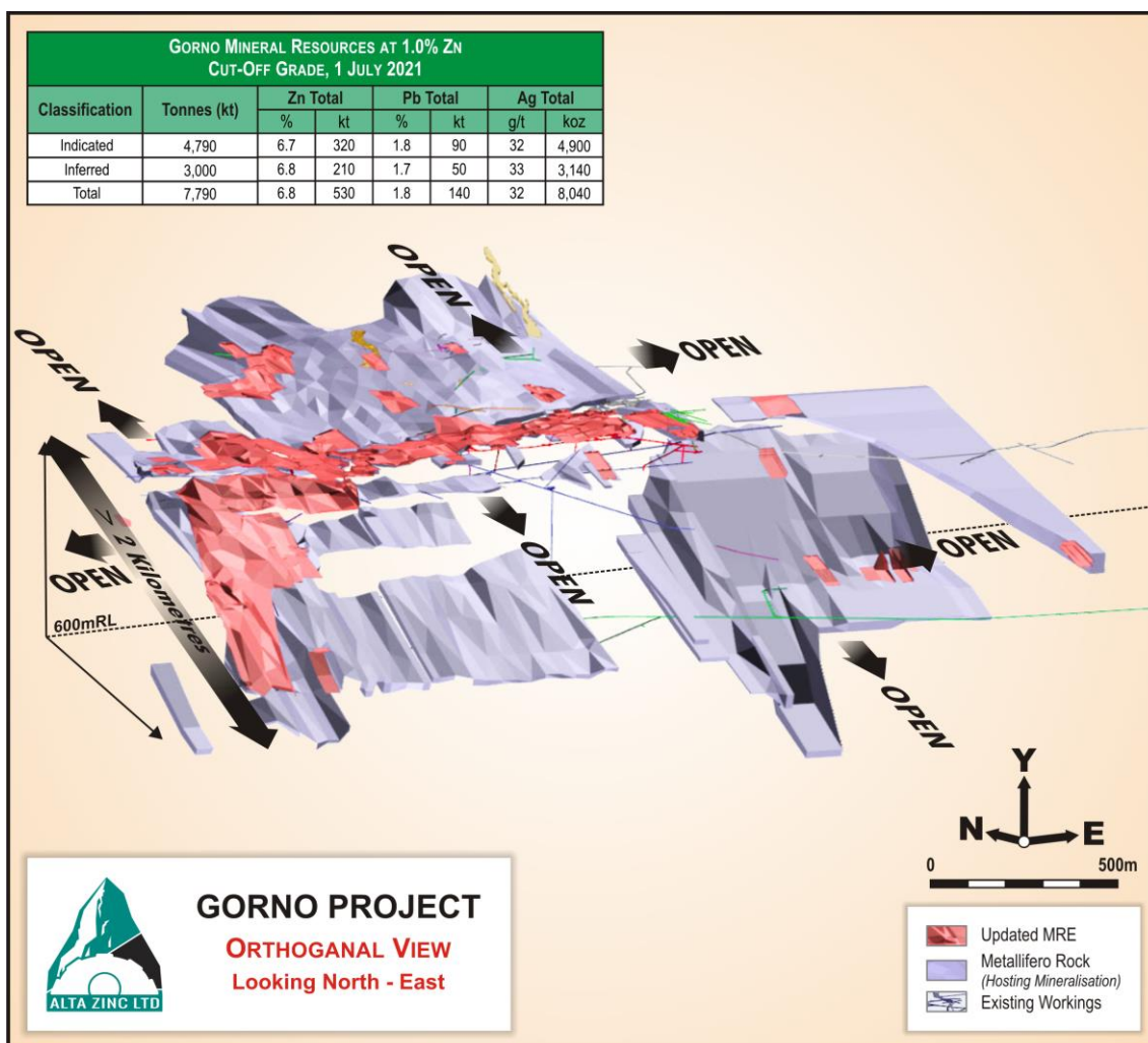
Figure 1: Orthogonal View of the Gorno MRE
