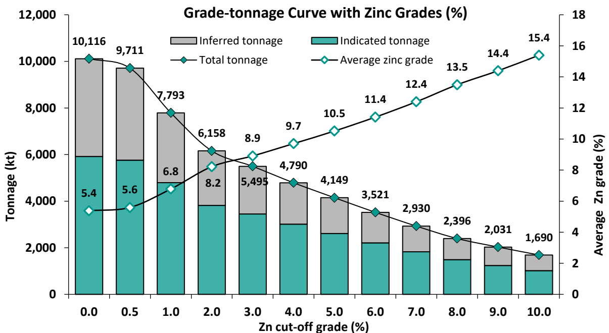
Figure 7: Grade Tonnage Curve Showing Zinc Grades
