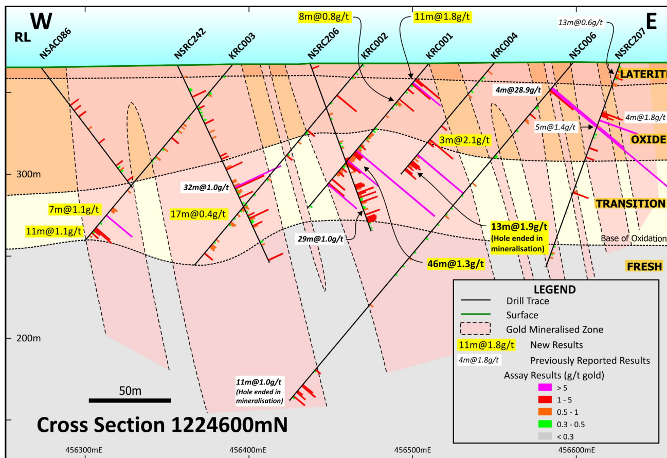
Figure 1. Drill section 1,224,600mN with new assays for KRC001 - KRC004.
