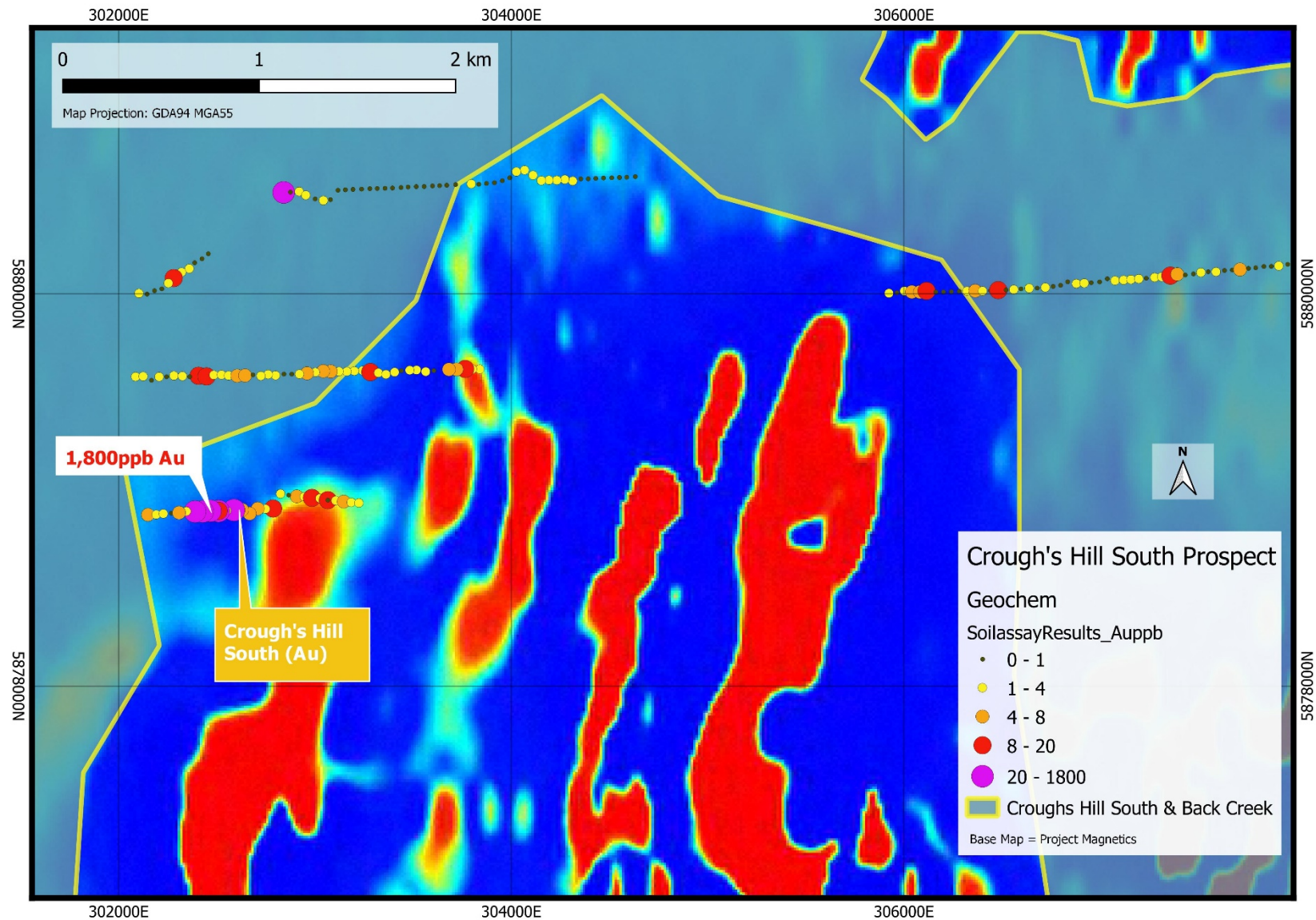
Figure 3 – Gold assays returned from soil sampling at the Crough's Hill South Prospect overlying the Project Magnetics (RTP 1VD)
