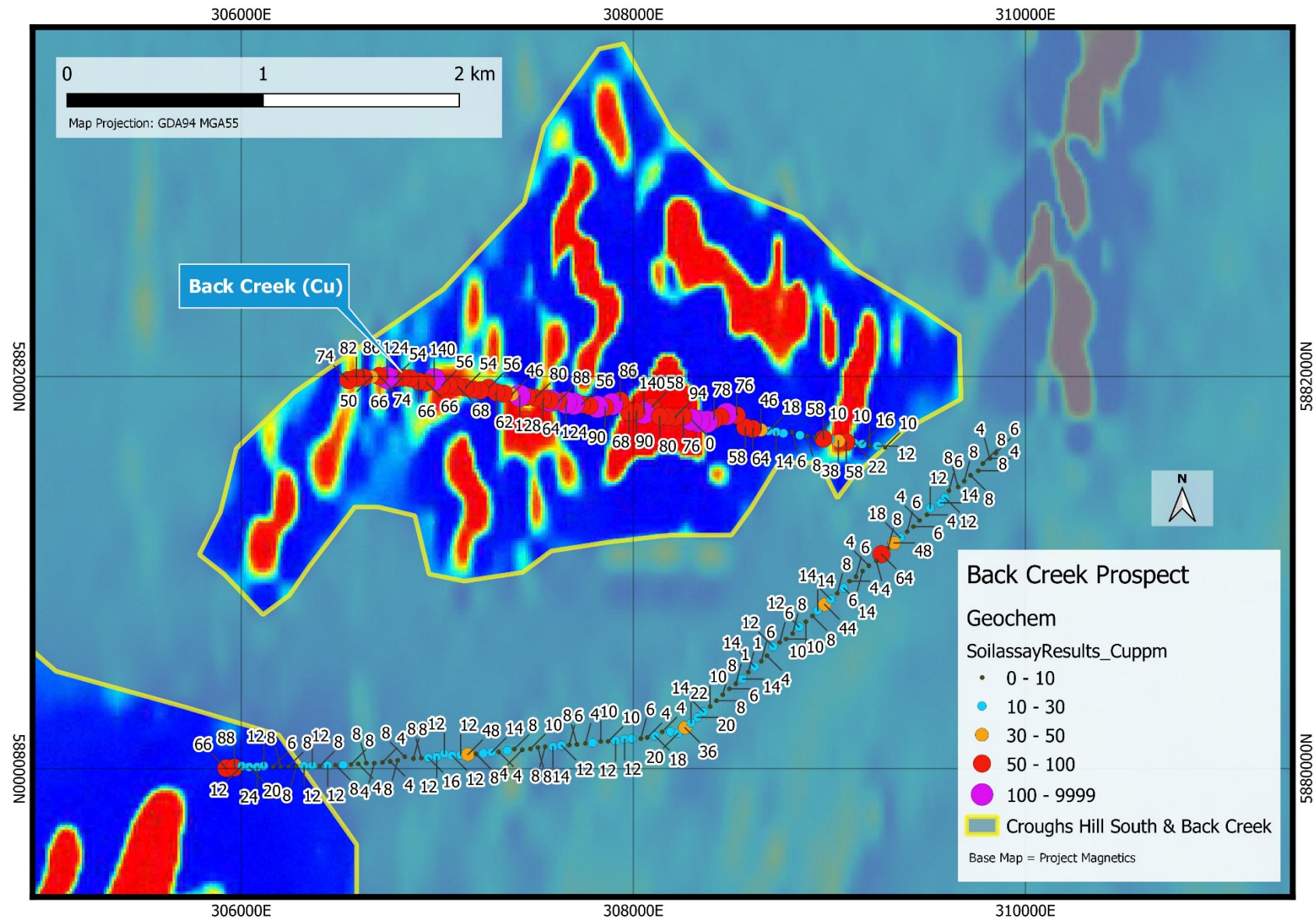
Figure 4 – Copper assays returned from soil sampling at the Back Creek Prospect overlying the Project Magnetics (RTP 1VD)
