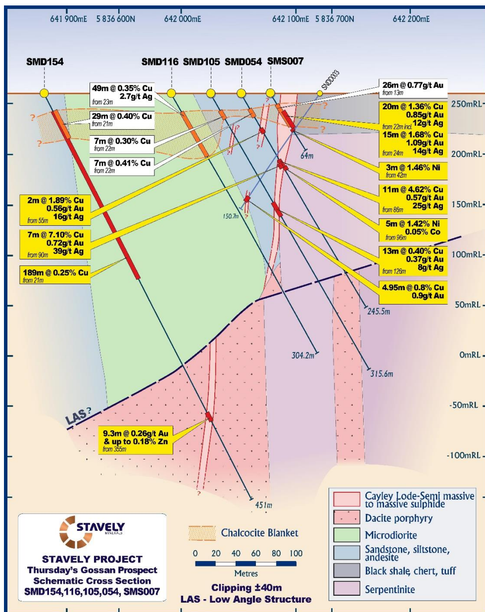
Figure 8. SMD154 drill section.
