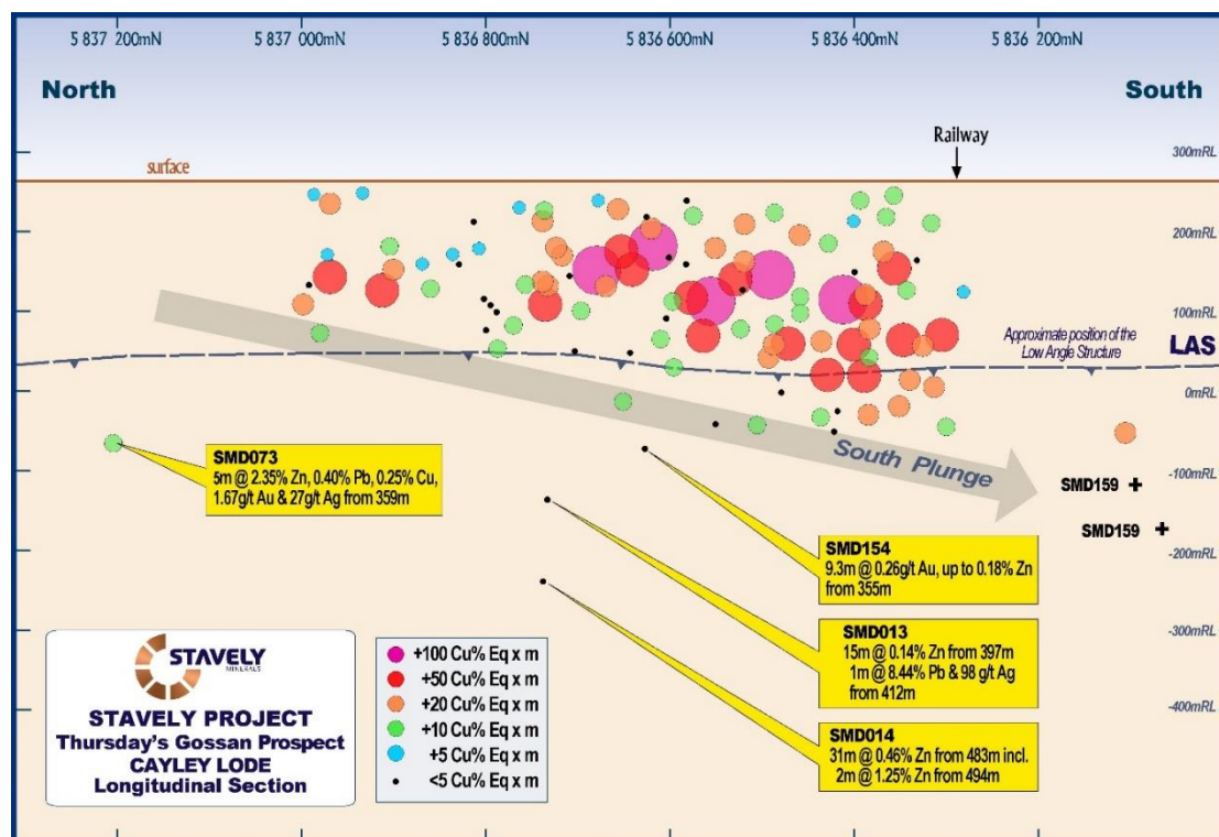
Figure 9. Cayley Lode long section.
