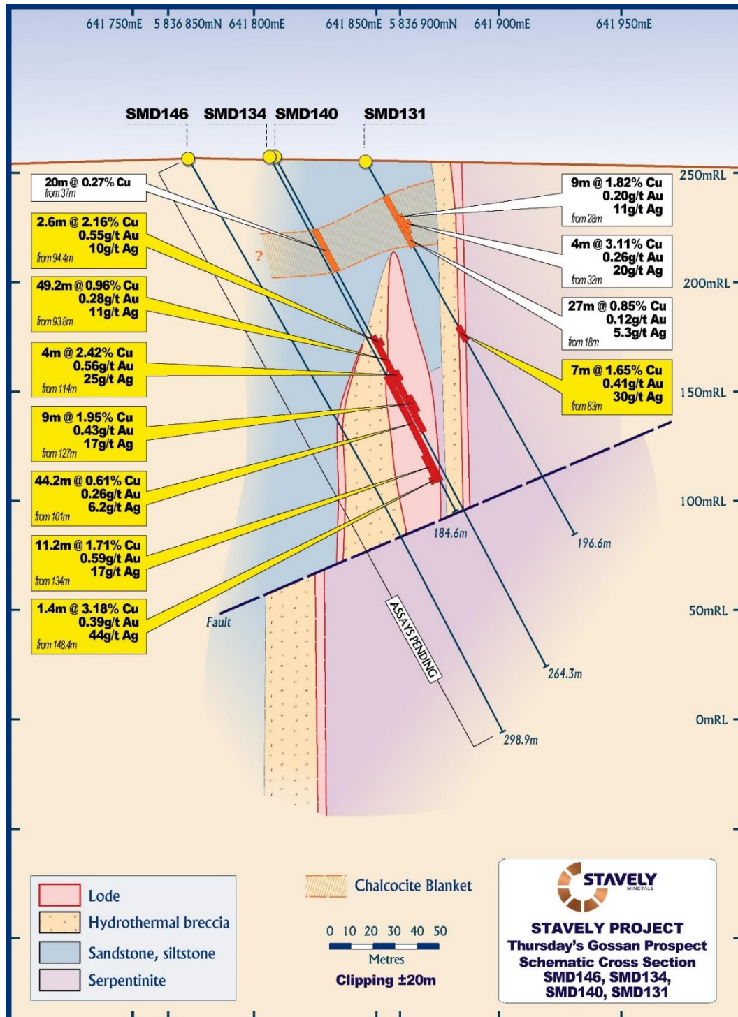
Figure 6. SMD131 drill section.
