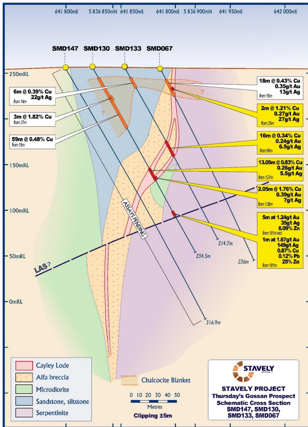
Figure 5. SMD130 drill section.
