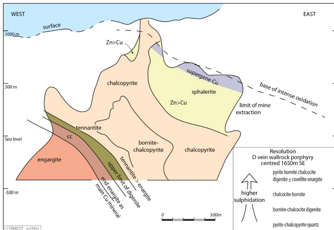
Figure 10. Sulphide zonation of the Magma, Arizona lode-style system.
