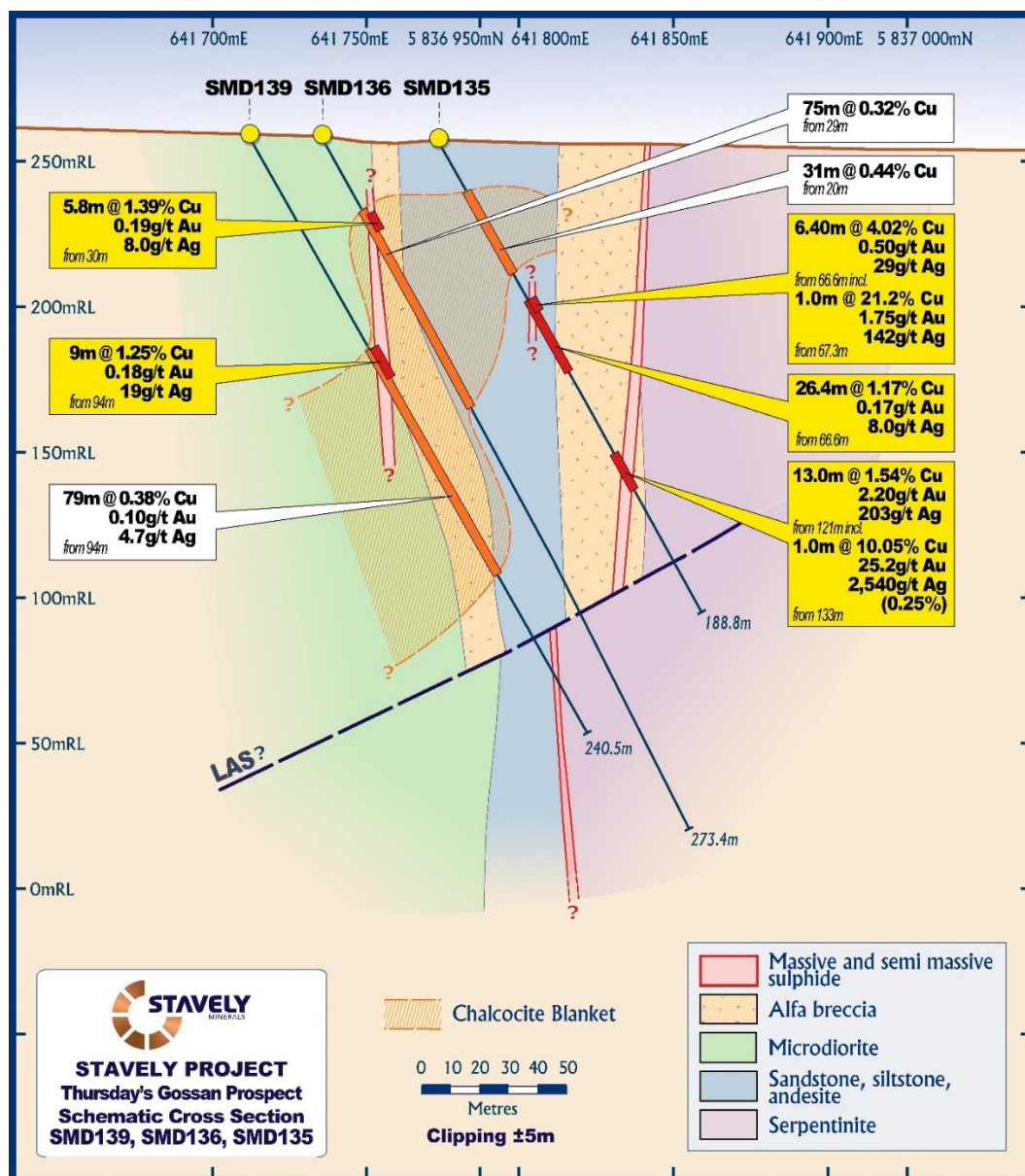
Figure 7. SMD136 and SMD139 drill section.
