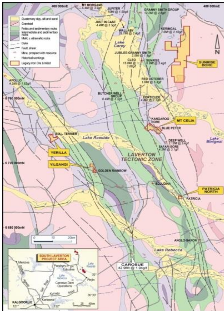
Figure 9 Legacy Iron's South Laverton Gold Projects including Mt Celia
