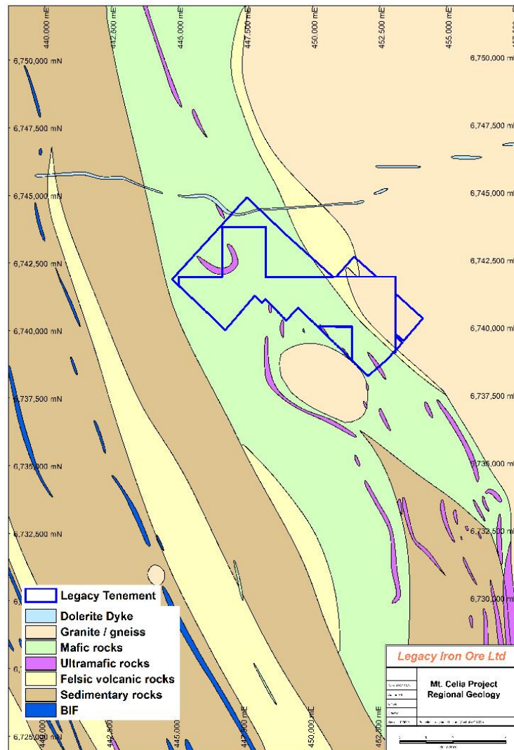
Figure 11 Regional Geology of the Mt Celia area
