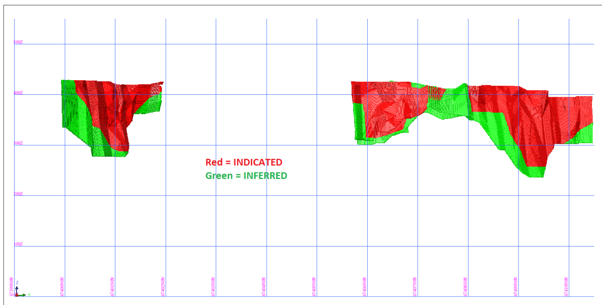
Figure 2 Long section of Blue Peter resource defining the classification showing the majority of the indicated category within 150m from surface.
