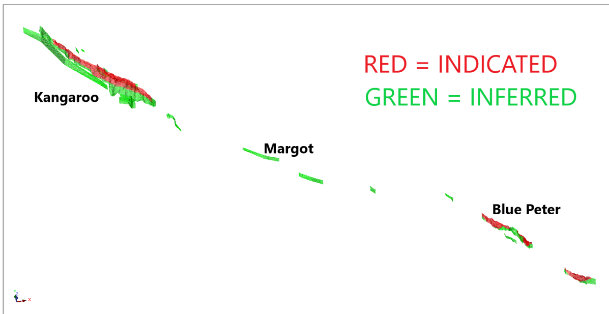
Figure 3 Classification of individual lodes with each prospect area.
