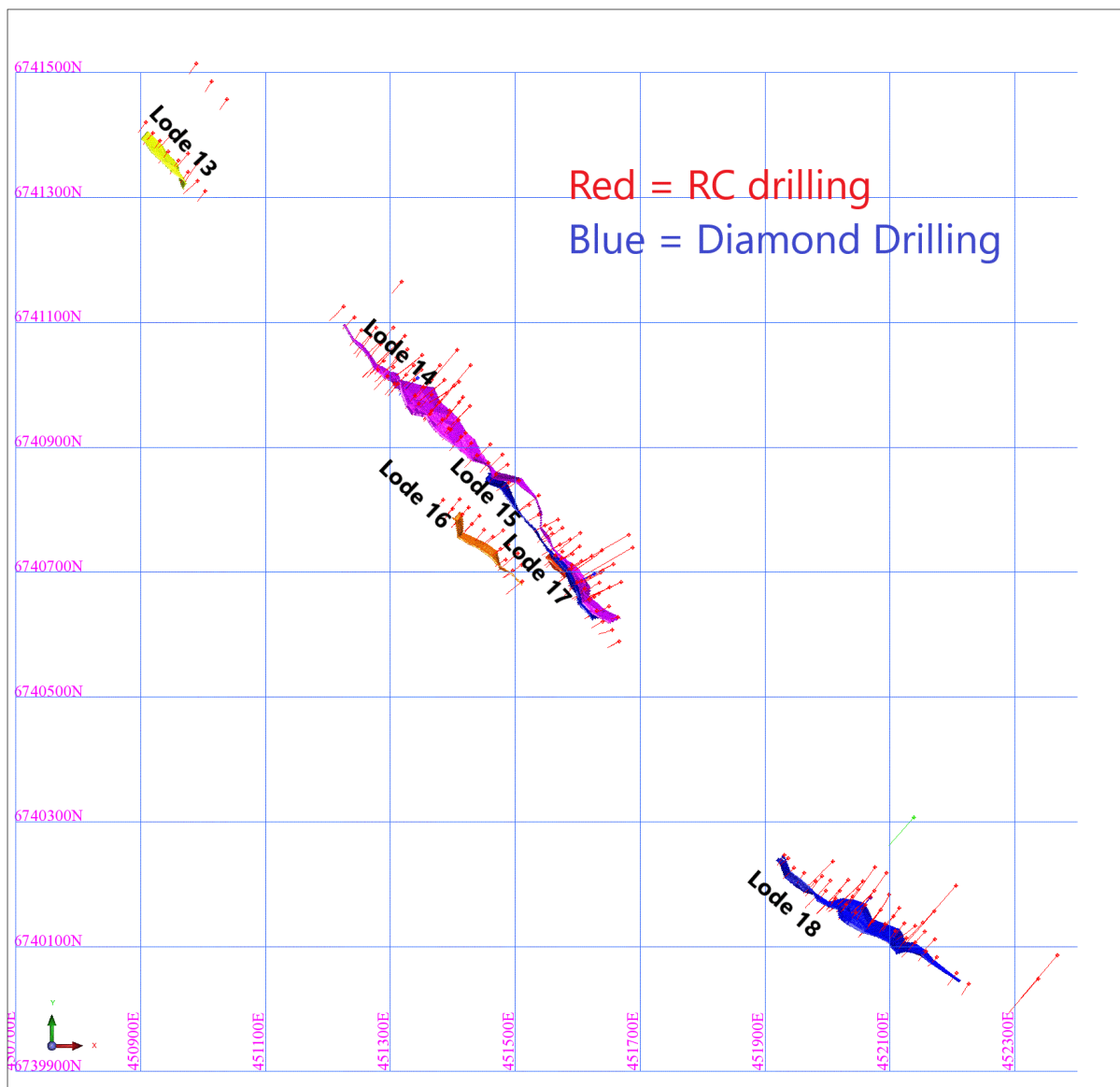
Figure 5 Blue Peter lodes and drillhole collars
