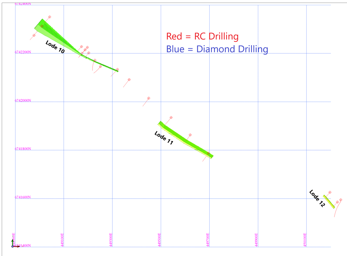
Figure 6 Margot lodes and drillhole collars
