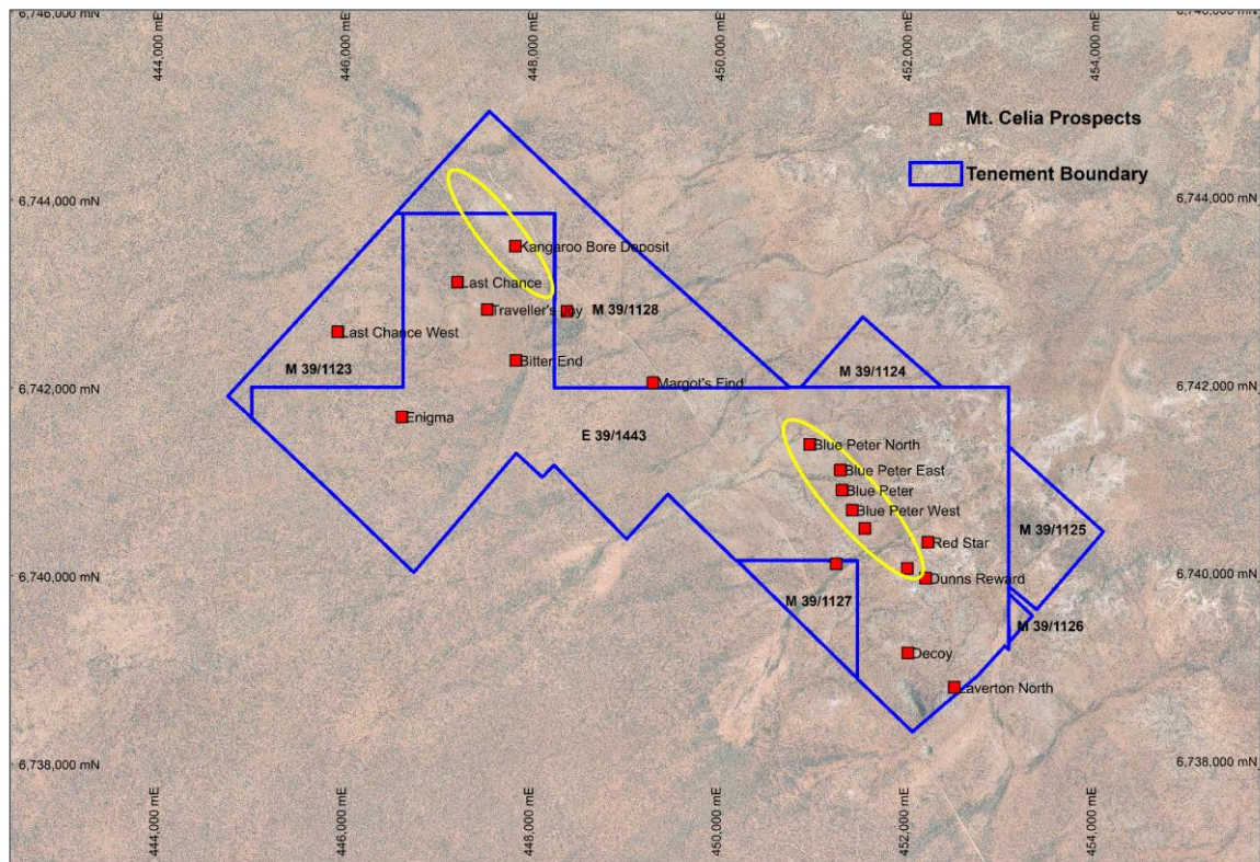
Figure 10 Mt Celia Project - Showing Kangaroo Bore, Blue Peter, Coronation and other prospects
