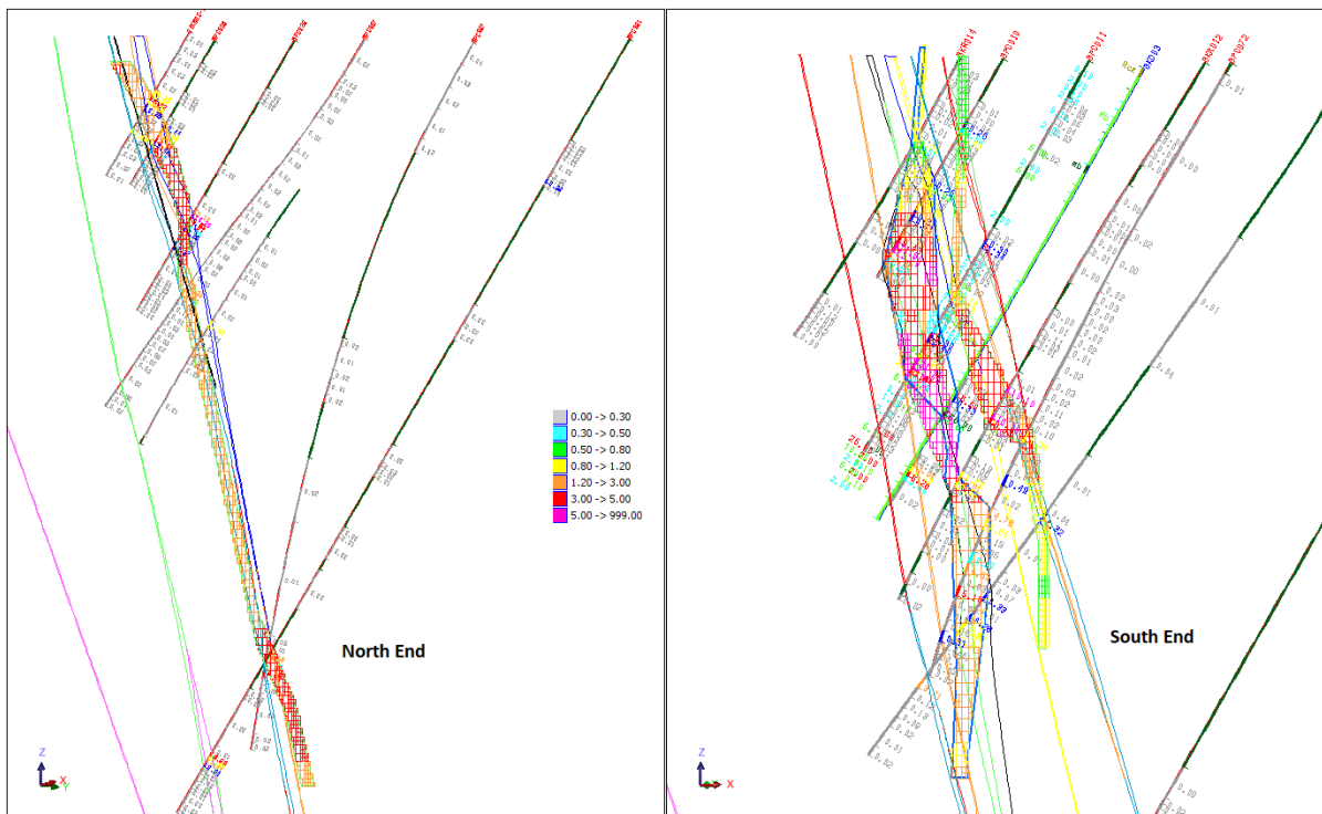
Figure 8 Blue Peter - Model section showing block grades, drilling and Dec 2020 interpretation outlines.
