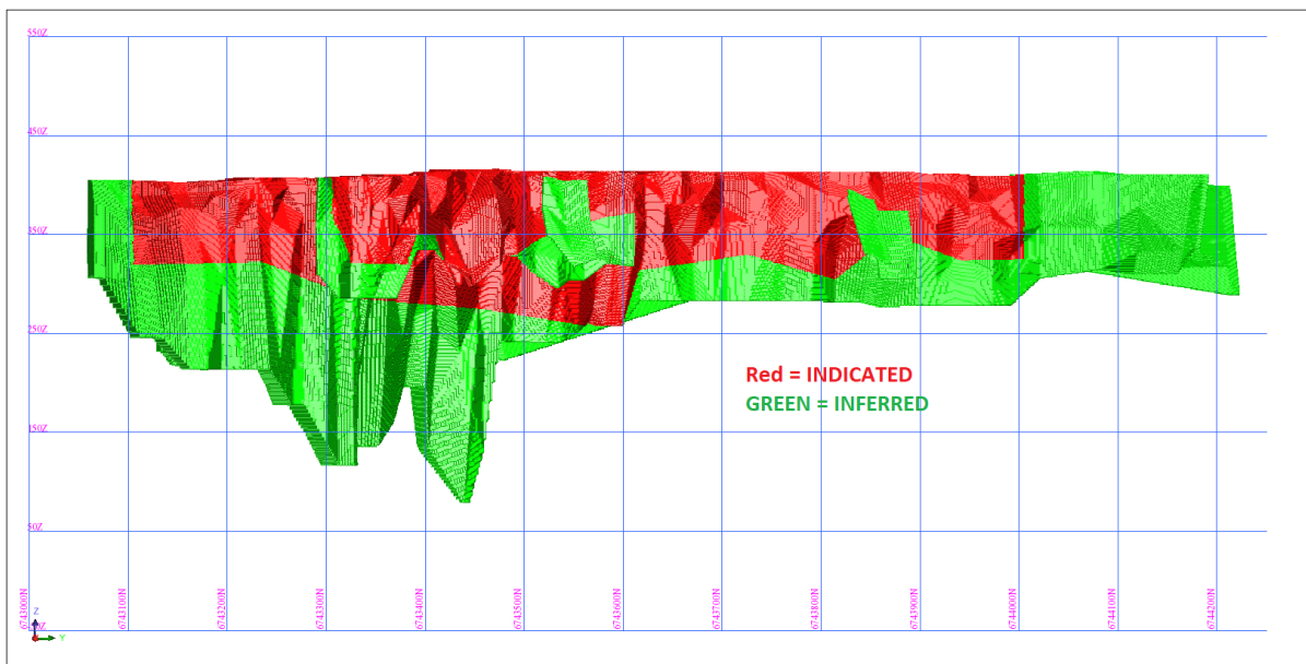
Figure 1 Long section of Kangaroo resource defining the classification showing the majority of the indicated category within 150m from surface.
