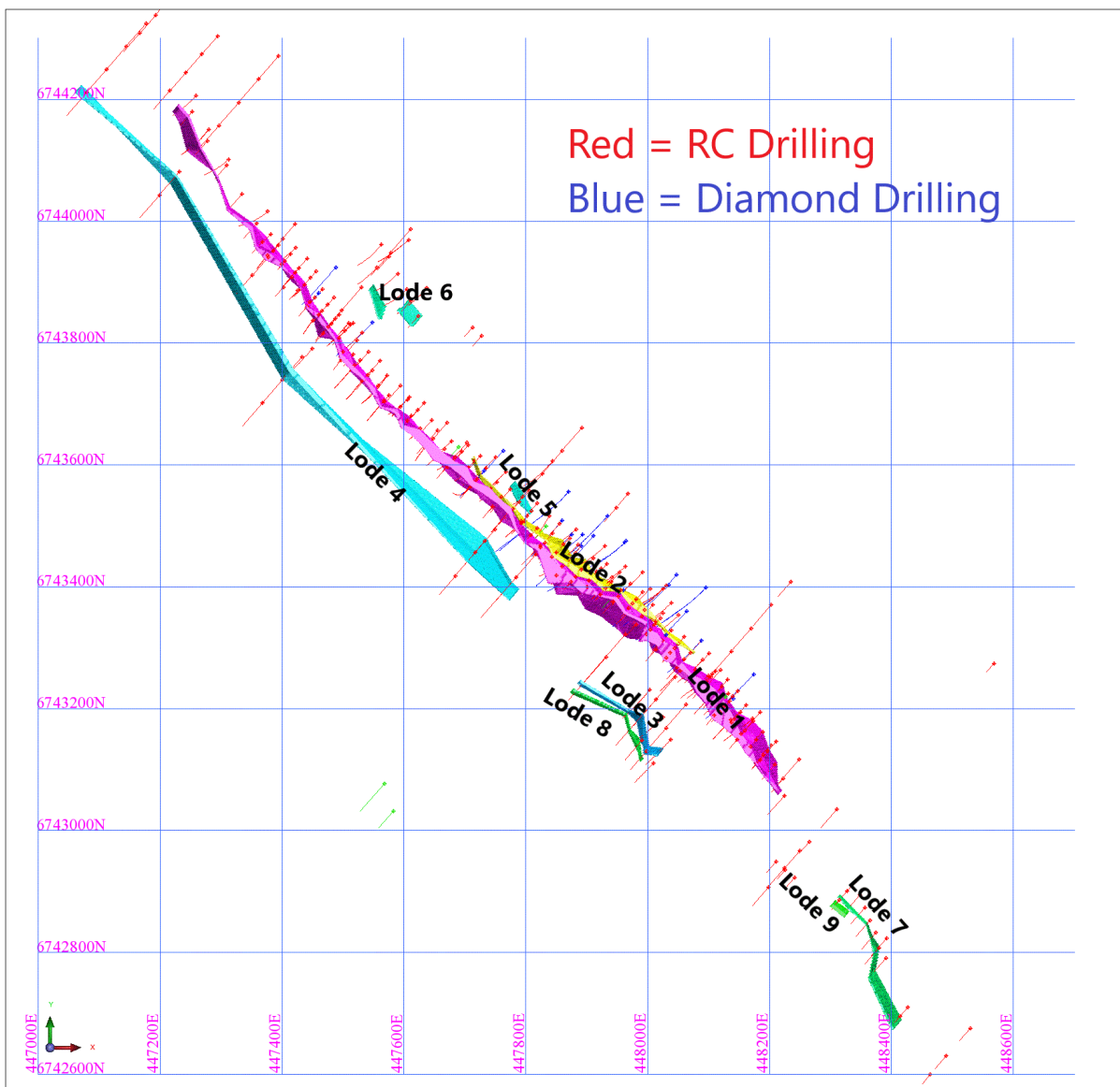
Figure 4 Kangaroo Bore lodes and drillhole collars
