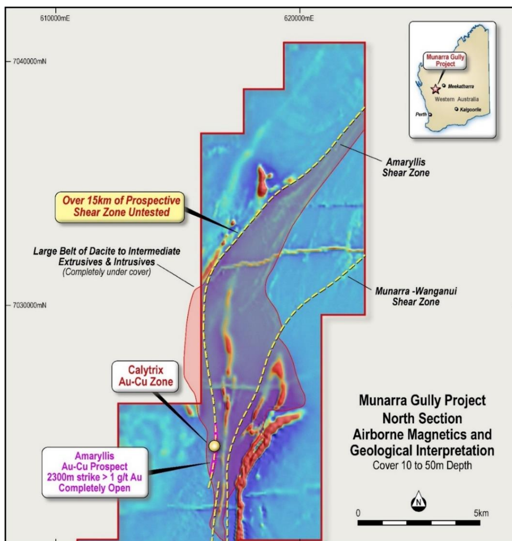
Image 10 – Munarra Gully Project – Location of Amaryllis Prospect over Airborne Magnetism
