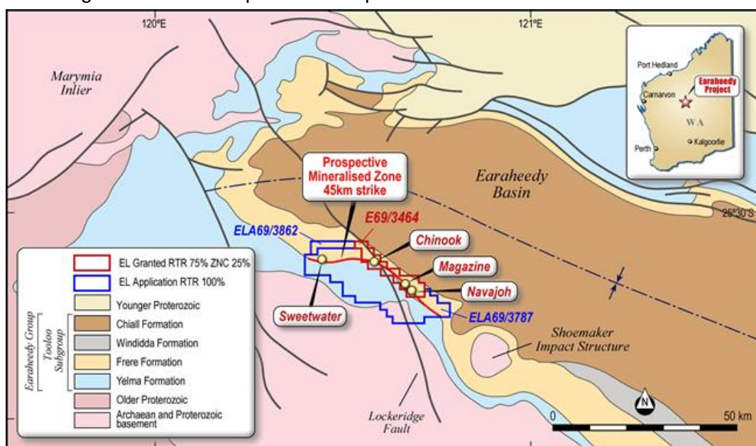
Image 1 – Earahedy Project With Regional Geology and Prospect Locations
