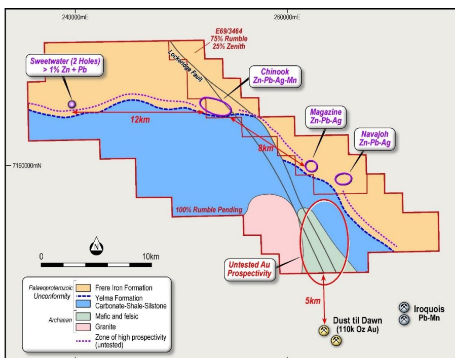
Image 2 – Earahedy Project Geology and Prospect Locations
