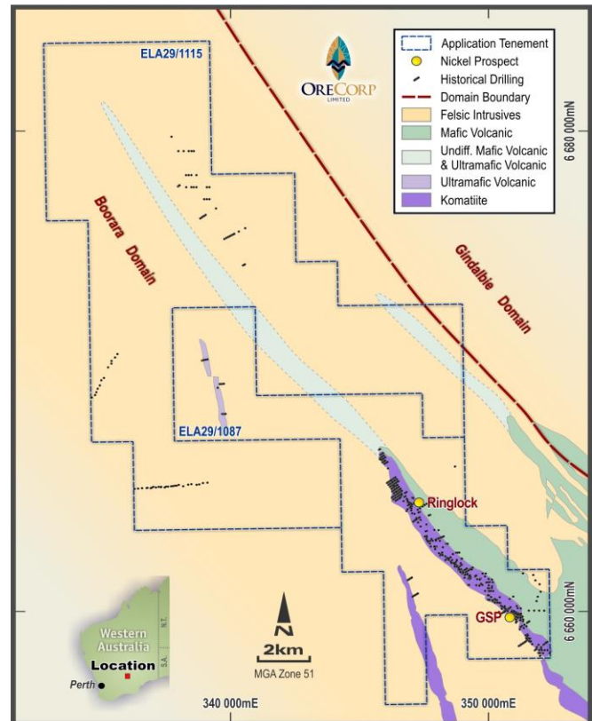
Figure 7: Historical drilling over geology
