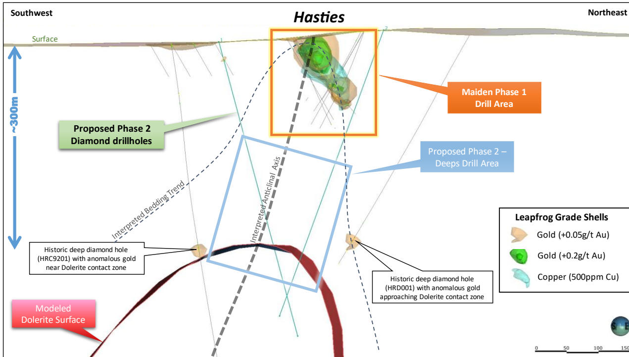
Schematic section through Hasties (looking north-west) showing modelled surface of Dolerite at depth and the area to be tested with Phase 2 diamond drilling
