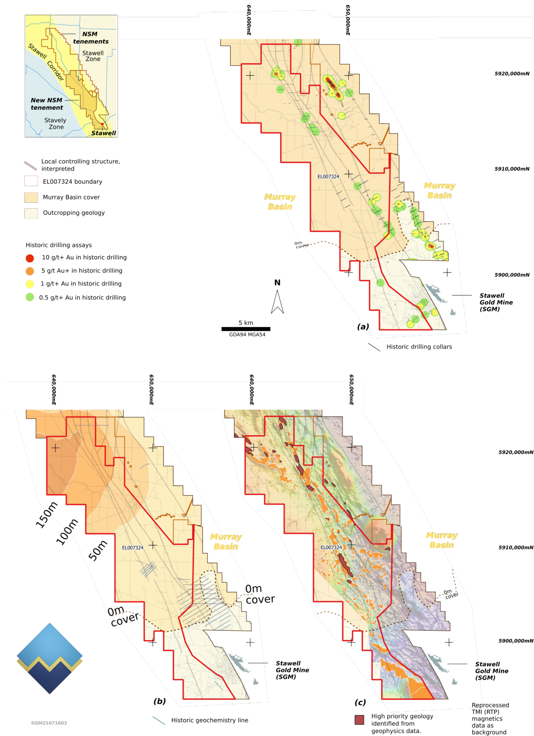
Figure 2. Detail of EL007324; (a) historic drilling and gold anomalism based on individual assays grades downhole, (b) historic geochemistry lines and depth of the Murray Basin sediments, and (c) magnetics data (RTP) with identified, interpreted basalt dome structures
