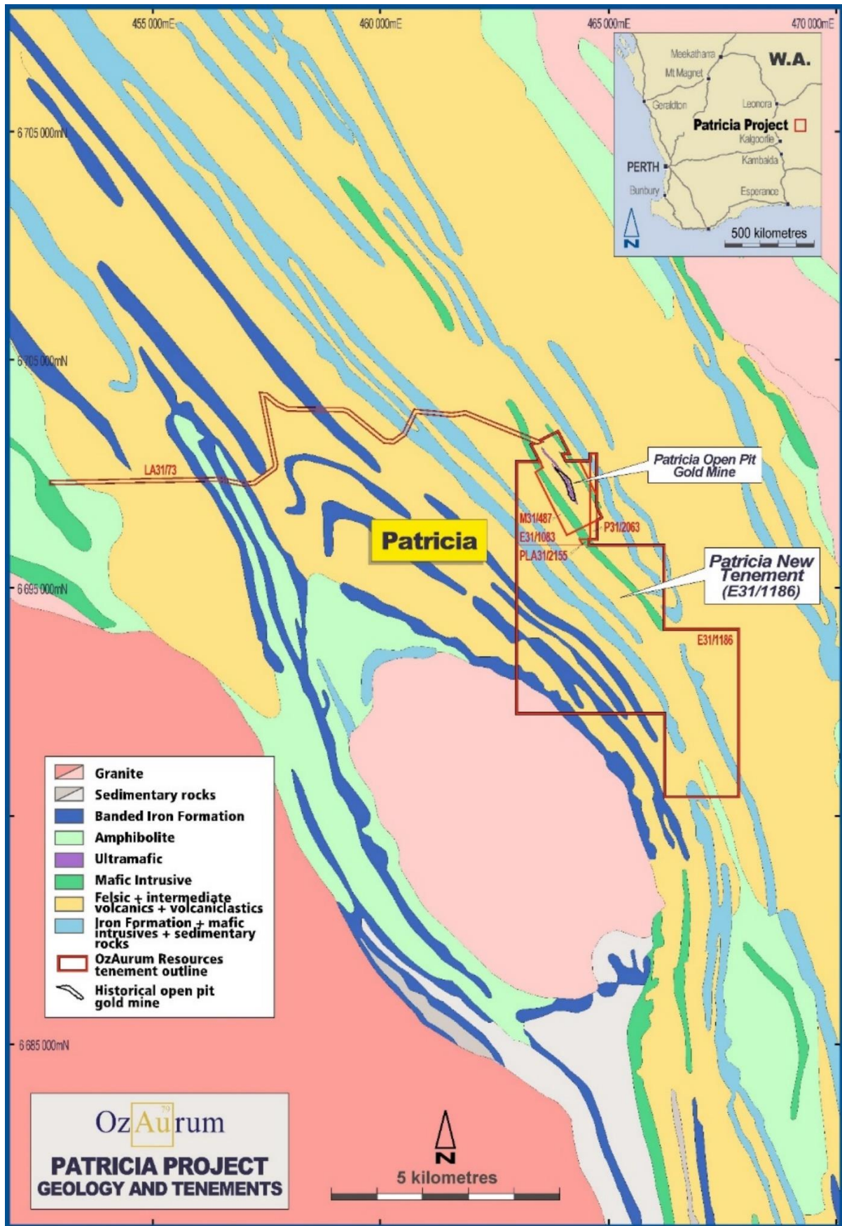
Figure 4: Patricia Gold Project Interpreted Geological Plan
