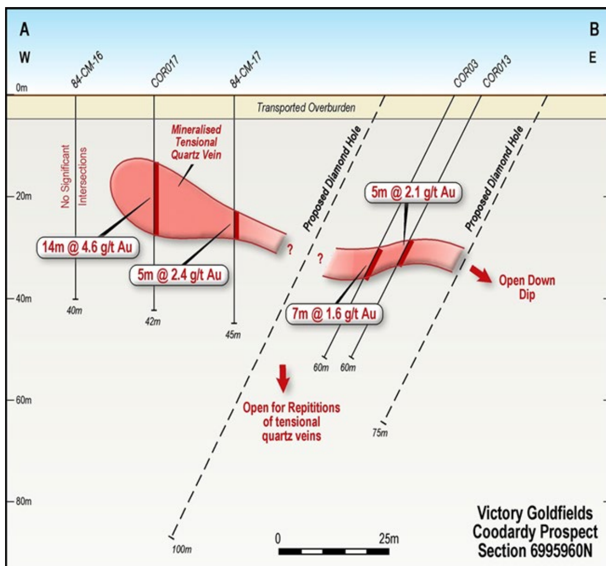
Coodardy Project cross section showing two DD hole locations
