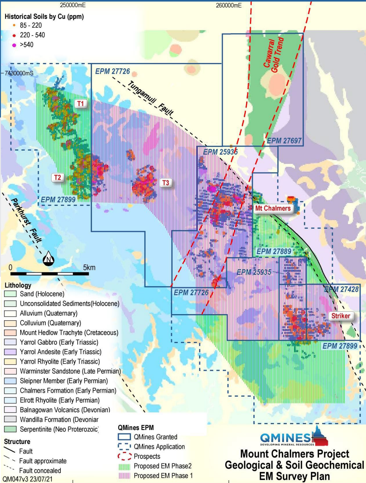
Figure 2: TDEM airborne survey area with flight lines, tenements and Mt Chalmers, T1, T2, T3 and the Striker copper in soil geochemical results.
